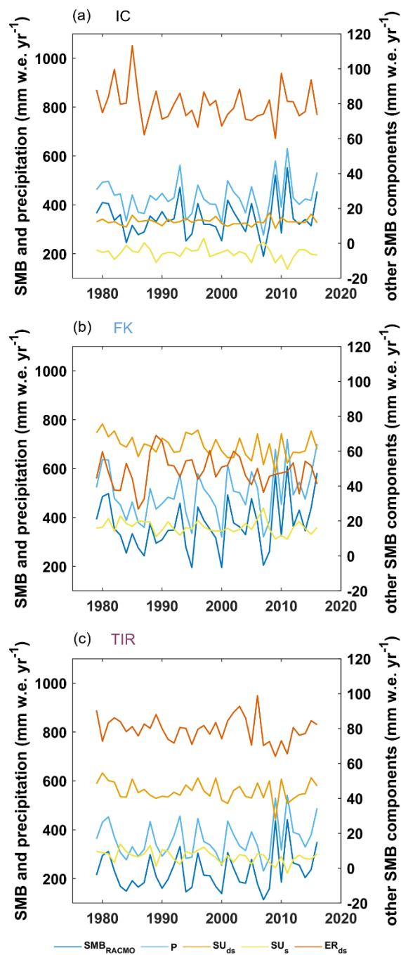
Figure S1: Temporal evolution of the SMB components and SMB derived from RACMO2.3 between 1979 and 2016 at (a) IC, (b) FK, and (c) TIR, expressed in \text{mm w.e. yr}^{-1} . Precipitation and SMB are represented on the left axis while sublimations and erosion are represented on the right axis.
