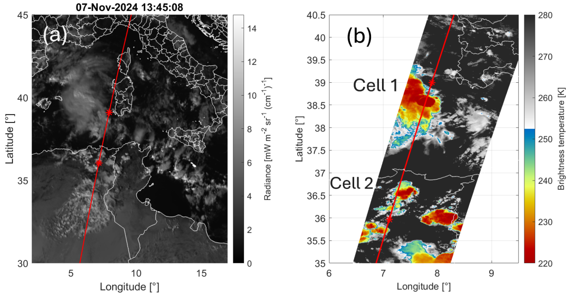
Figure 7. (a) Radiance from channel 1 ( 0.6\mu\text{m} ) of MSG, on November 7th, 2024 at 13:45 UTC. The EarthCARE ground track, corrected for parallax is shown as the red line. (b) The MSI IR channel data from the EarthCARE satellite. The overpass time is 13:43 UTC on November 7th, 2024, frame 2530D. The red line is the satellite ground track. The segment between the two stars is plotted in Fig. 8.
