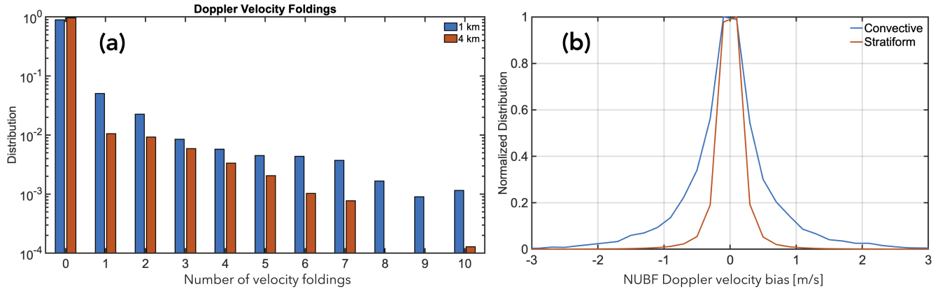
Figure 6. (a) The normalized frequency of occurrence of CPR Doppler velocity folding, (b) The NUBF induced CPR Doppler velocity bias in m/s in convective and stratiform regions, derived by multiplying the along track reflectivity gradient by a correction coefficient ( 0.165 \text{ m} \cdot \text{km/s} \cdot \text{dB} ) (Kollias et al. 2023).
