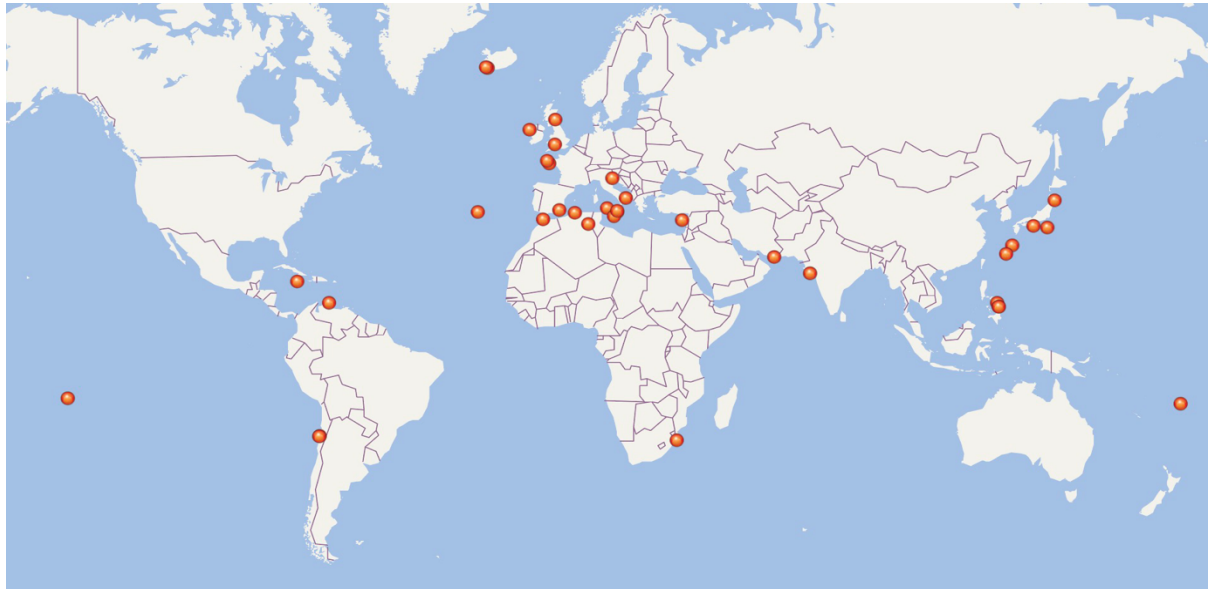
Figure 3. Locations of coastal boulder deposit datasets recorded in ISROC-DB V1p0 (Kennedy et al., 2025b)
