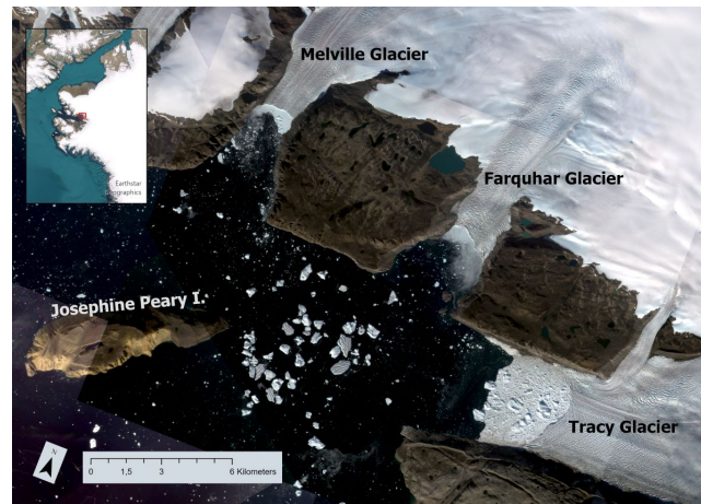
Figure 1. Map of Inglefield Fjord with the three study glaciers Tracy, Farquhar, and Melville marked as well as Josephine Peary Island (Qeqertarsussarssuaq). The basemap is a mosaic of optical satellite images between 25 th and 29 th of August 2022 obtained from Planet labs ( planet.com/explorer )
