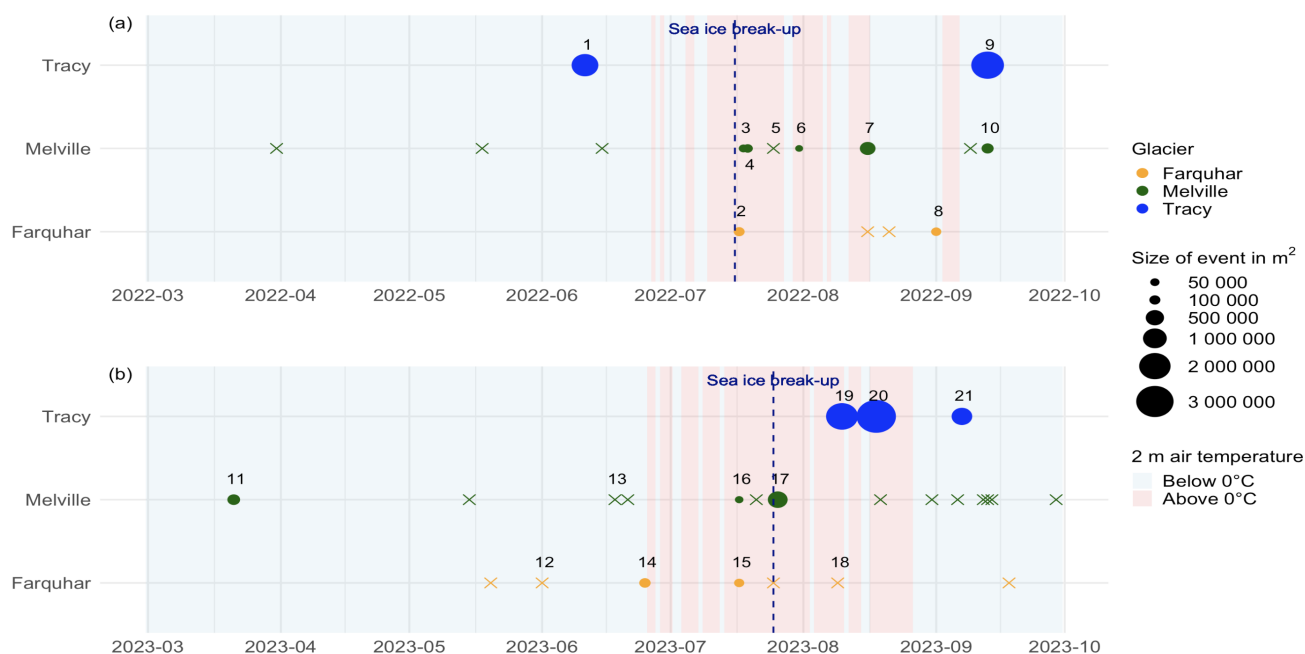
Figure 10. All identified calving events on Melville, Farquhar and Tracy Glacier in 2022 (a) and 2023 (b). An event is plotted on the first detectable day (in satellite imagery) after the event has happened on the x-axis and distributed to its glacier location on the y-axis. Further, the colours orange, green and blue represent Farquhar, Melville, and Tracy. The approximate spatial size of each calving event in m^2 (if measured) are indicated by the size of the points. If it is not possible to determine the size of the calving event, it is marked as a cross. Red and blue backgrounds symbolise positive and negative daytime air temperatures, respectively, based on 2 m air temperature data from CARRA at 12:00 PM UTC. The numbers (1-21) added to some points are reference numbers for events given in Table A1 and the dashed vertical lines represent sea ice break-up dates: 16/7/2022 and 25/7/2023, identified from changes in buoy movements and satellite imagery.
