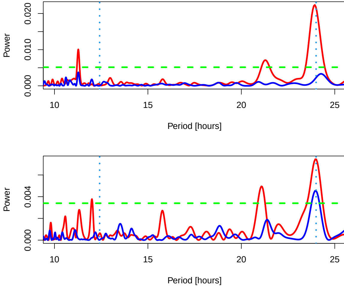
Figure 13. Power spectra of OMB buoy velocity data decomposed to assess if there is any evidence of tidal forcing in the mélange movements at this location. (a) shows the OMBDXT buoy (top) and (b) shows data from the OMBEXB (bottom). The observed velocities from the two buoys were split into two intervals covering the first and second halves of the observation period in 2023. The spectra for the time varying velocities for each interval are shown (red is first half, blue last half). The vertical dashed lines indicate the period of the tidal M2 constituent (12 hours 25 minutes) and the 24-hour period which would be expected if the velocities were responding to a tidal forcing. The green dashed line is the significance level at p=0.01 . Lomb-Scargle periodogram methods (VanderPlas, 2018) were used because the data are gapped and not evenly spaced.
