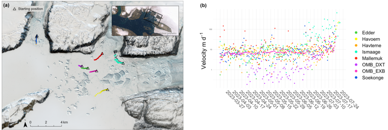
Figure 4. The movement of the 8 buoys (Edder, Havterne, Havørn, Ismaage, Mallemuk and Soekonge, DXT and EXB) placed in front of Tracy, Farquhar, and Melville daily averaged from the end of March until mid-July 2023. The basemap in (a) is Sentinel-2 from 25 th May 2024 as in Fig 2. The triangle indicates the starting position.
