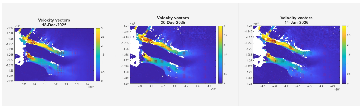
Figure A1. Ice velocity vectors for the study glaciers for three snapshots in winter 2025 to 2026, derived from Sentinel-1 feature tracking as described in Solgaard et al. (2021). Arrows show the velocity vectors, colours indicate absolute velocities. Close to the front of all glaciers and in the mélange zone, the increased surface variability makes feature tracking challenging and it is only occasionally possible to extend as far shown here, hence why we show figures from a different time to the period when GNSS buoys were deployed.
