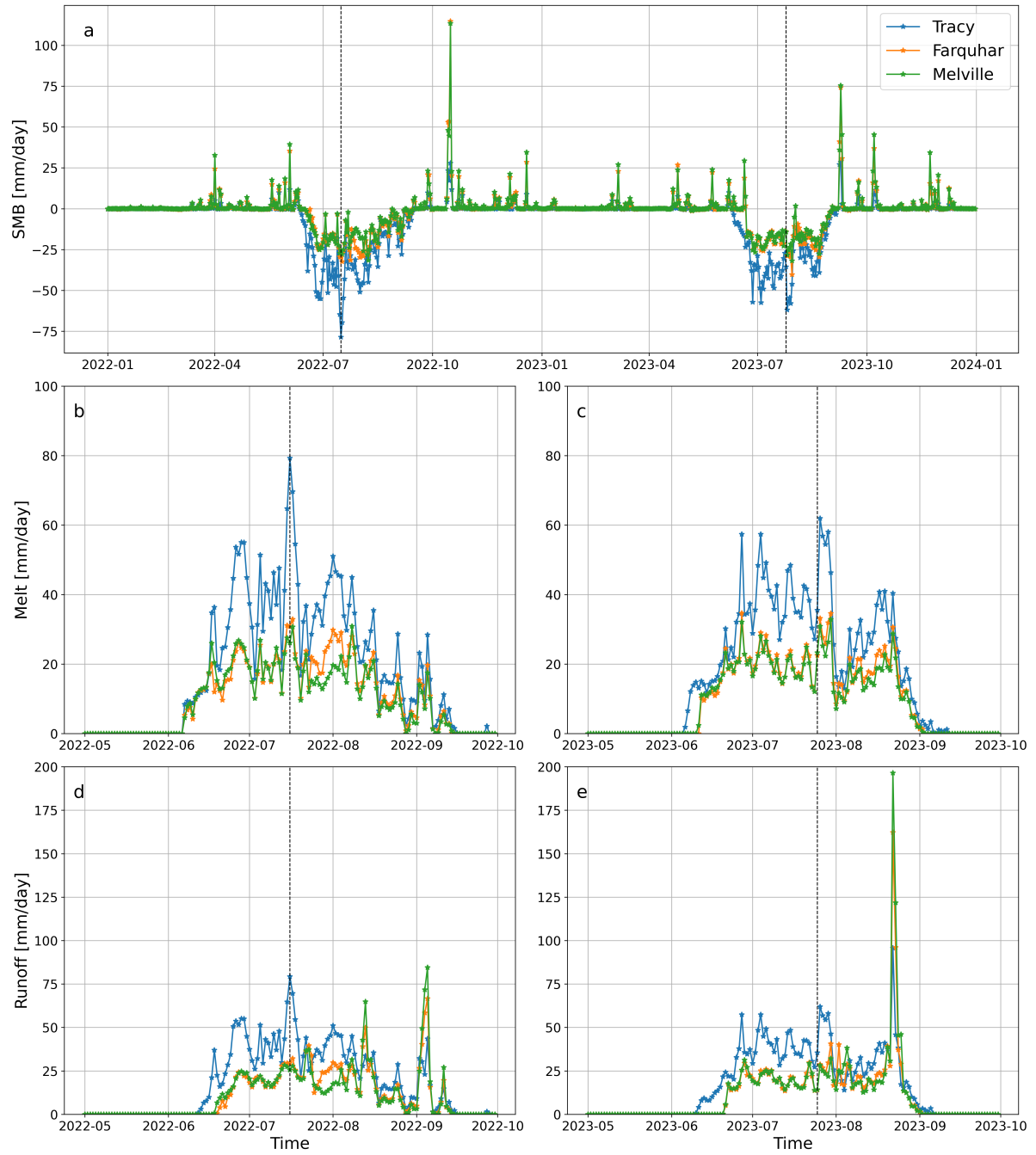
Figure 15. Daily SMB (a), surface melt 2022 and 2023 (b and c, respectively), and surface runoff 2022 and 2023 (d and e, respectively) for the three glaciers. All values are given in mm per day, from the model grid cell nearest the glaciers. The vertical black dashed lines show the date of the sea ice break-up in 2022 and 2023.
