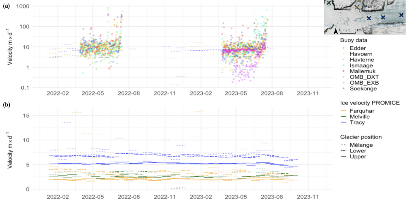
Glacier, mélange and buoy velocities in 2022 and 2023
