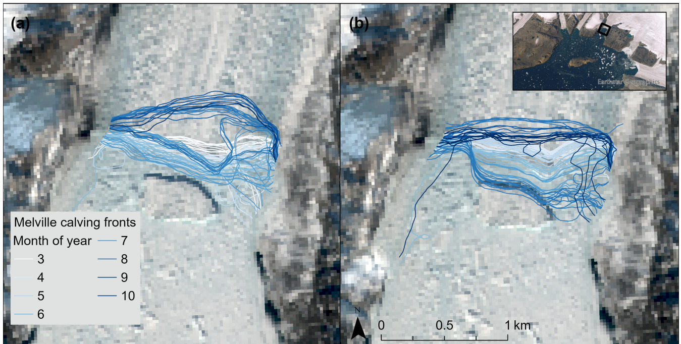
Figure 8. Calving front positions for Melville Glacier in 2022 (a) and 2023 (b) generated with deep learning (Loebel et al., 2024). The basemap is Sentinel-2 from 25 th May 2024, processed on Sentinel Hub EO Browser using a natural colour optimisation (Sinergise) to highlight the annual cycle from winter months (white) through to summer (blue) and autumn (dark blue). Note the different spatial scale compared to Fig 7. Note also that some lines denote errors generated by the deep learning algorithm which we retain here to highlight the importance of manual checking.
