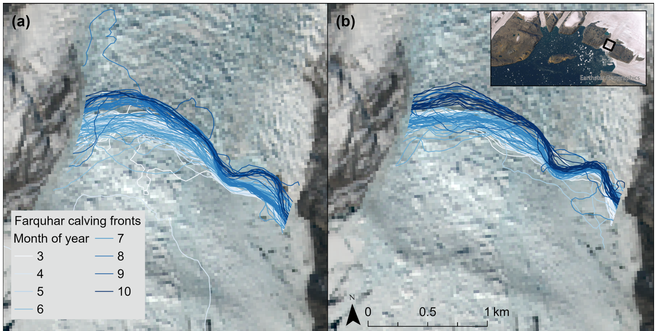
Figure 7. Calving front positions for Farquhar Glacier in 2022 (a) and 2023 (b) generated with deep learning (Loebel et al., 2023). Calving front positions for Farquhar Glacier in 2022 (a) and 2023 (b) generated with deep learning (Loebel et al., 2023). The basemap is Sentinel-2 from 25 th May 2024, processed on Sentinel Hub EO Browser using a natural colour optimisation (Sinergise) to highlight the annual cycle from winter months (white) through to summer (blue) and autumn (dark blue). Note the different spatial scale compared to Fig 7. Note also that some of the lines representing calving fronts are likely to be errors generated by the deep learning algorithm which we retain here to highlight the importance of manual checking.
