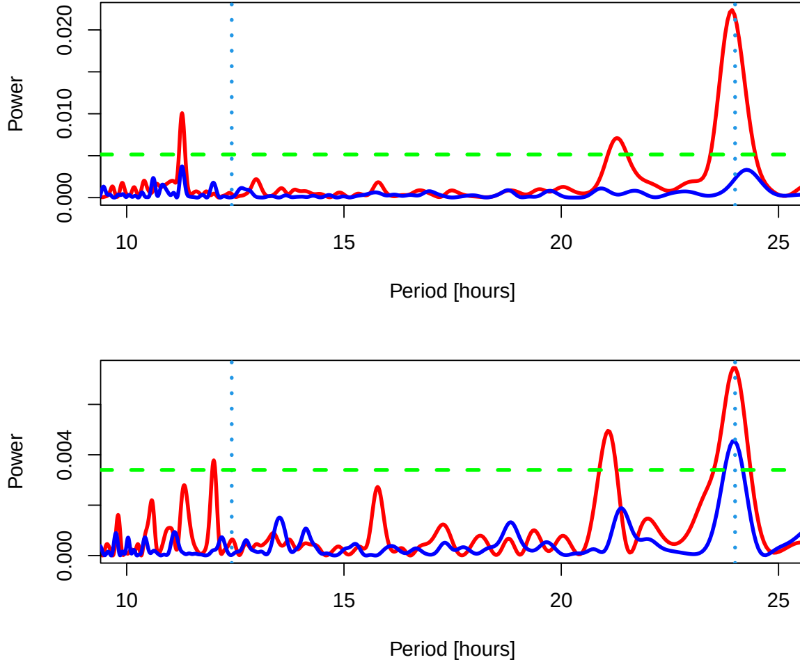
Figure 13. Power spectra of OMB buoy speed-velocity data decomposed to assess if there is any evidence of tidal forcing in the mélange movements at this location. (DXT-a) shows the OMBDXT buoy (top, EXB- ) and (b) shows data from the OMBEXB (bottom). The intervals observed velocities from the two buoys were split into two intervals covering the first and second halves and-of the observation period in 2023. The spectra for the time varying velocities for each half interval are shown (red is first half, blue last half). The vertical dashed lines indicate the period of the tidal M2 constituent (12 hours 25 minutes) and the 24-hour period which would be expected if the velocities were responding to a tidal forcing . The green dashed line is the significance level at p=0.01 . Lomb-Scargle periodogram methods (?) (VanderPlas, 2018) were used because the data are gapped and not evenly spaced.
