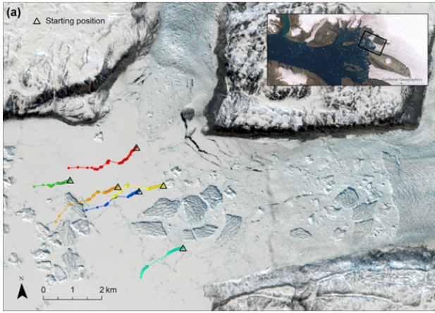
Figure 3. Movement of the TRUSTED buoys in the mélange of Tracy and Farquhar glaciers averaged over the day from the end of March until mid-July 2022. The basemap in (a) is an image from the Sentinel-2 satellite from 25 th May 2024. The grey-outline-around-the-coloured points-triangle indicates the starting position.
