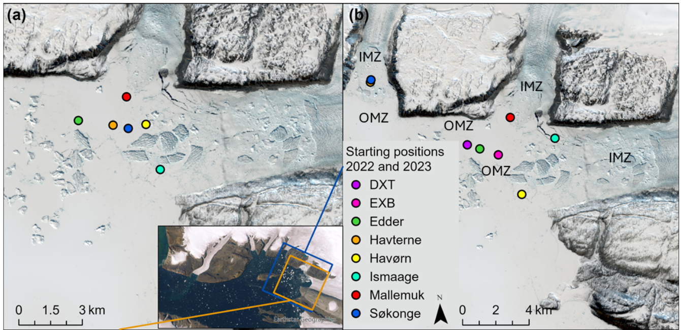
Figure 2. Starting positions of the buoys in 2022 (a) and 2023 (b). On the map (a) the The basemap is Sentinel-2 from 25 th May 2024, processed on Sentinel Hub EO Browser using a natural colour optimisation (Sinergise). Note the different spatial scales. We also label the inner (IMZ) and outer (OMZ) mélange zones as discussed above. While a subjective label, the inner zone reflects much rougher and likely thicker mélange with larger numbers of large icebergs that are very difficult to access. The OMZ is also difficult to access with many icebergs but also includes some areas of flatter sea ice that permits access on foot.
