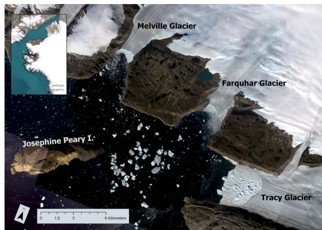
Figure 1. Map of Inglefield Fjord with the three study glaciers Tracy, Farquhar, and Melville marked as well as Josephine Peary Island (Qeqertarsussarsuuaq). The basemap is a mosaic of optical satellite images between 25 th and 29 th of August 2022 obtained from Planet labs (planet.com/explorer)
