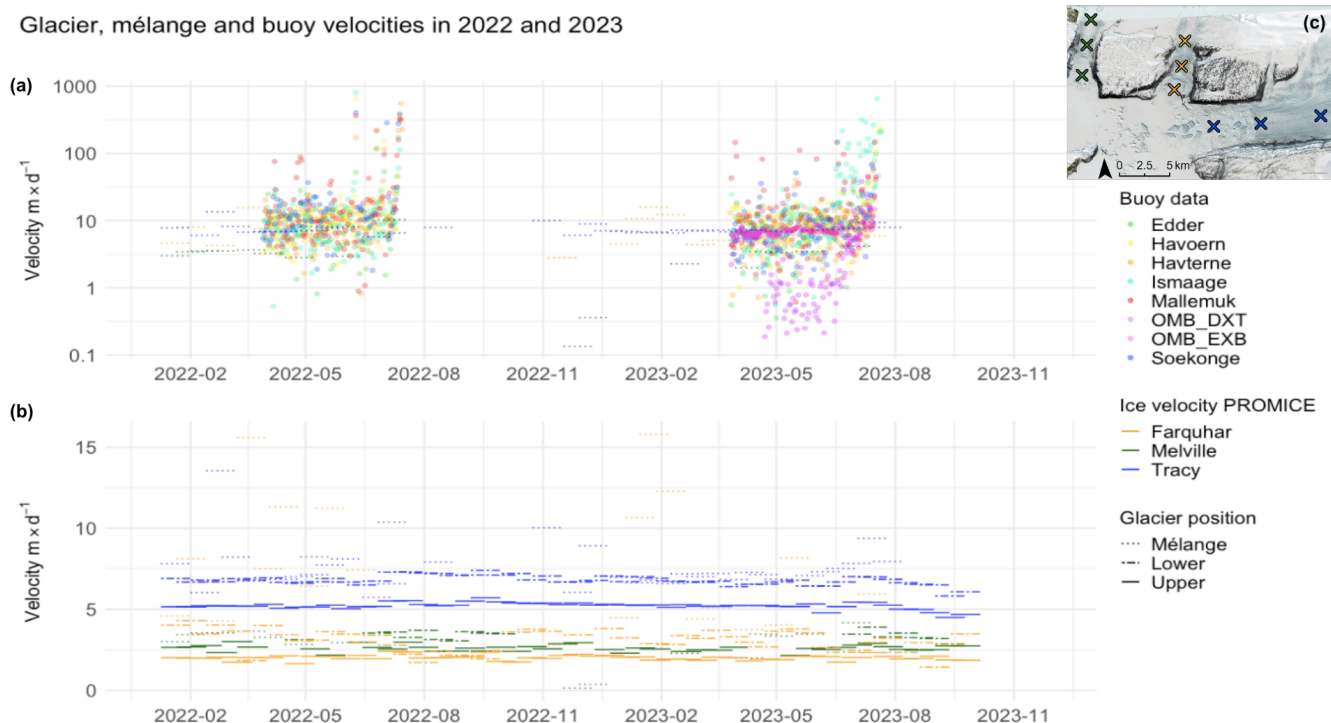
Figure 5. Mélange and glacier velocities for Farquhar, Melville and Tracy from the PROMICE Sentinel-1 ice velocity dataset (Solgaard et al., 2021) and in situ buoy movements. a) shows a comparison of the velocity of the mélange represented by in situ buoys (dots) and the PROMICE mélange product (dotted line), b) shows the velocity from PROMICE from the three positions shown on c) for the mélange, the upper and the lower point on each of the glaciers. Buoy marker colours in a) correspond to same colours as in Fig. 3 & 4 but are translucent to allow easier comparison with satellite derived velocities.
