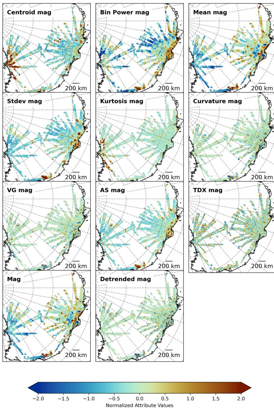
470 Figure A2: Normalized attributes based on magnetic data. See text and Table 1 for more details.
