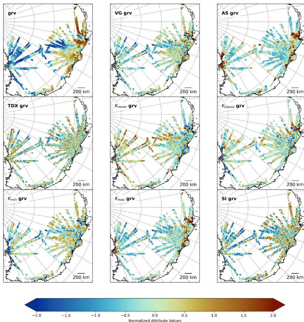
480 Figure A3. Normalized attributes based on gravity data. See text and Table 1 for more details.
