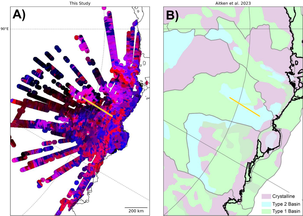
405 Figure 8: Zoom in for the Wilkes land area for comparison of our results and Aitken et al. (2023): (A) Geographical distribution of the SOM, (B) Geological bed types from the study by Aitken et al. (2023). See Figure 7 for location and orange line indicates profile shown in Figure 9.
