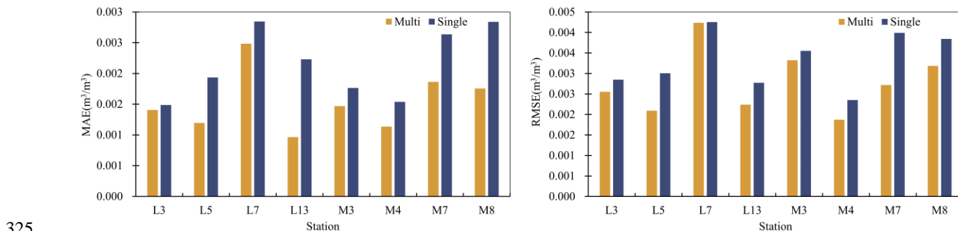
325 Figure 7: Comparison of accuracy before and after correlated sites joining, showing high correlations among nearby small-scale sites and varying correlations among larger sites.
