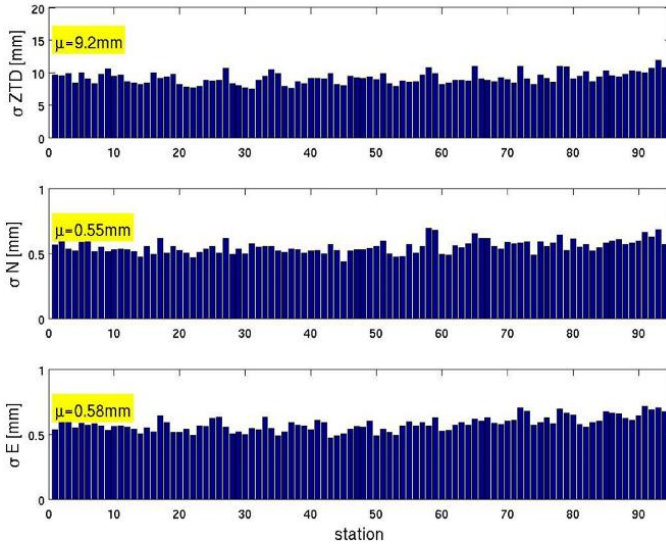
Figure A5. Same as Figure A1, but for ZTD run in the sparse network configuration.
