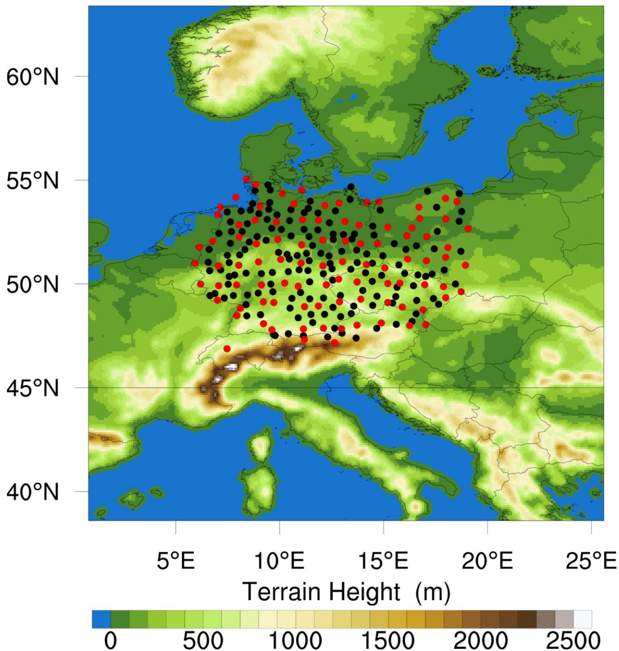
505 Figure 1. The WRF model domain with terrain height representation. The GNSS stations in the assimilation study are depicted in red to signify the sparse network with a 1-degree density, while the combination of black and red indicates the dense network with a 0.5-degree density.
