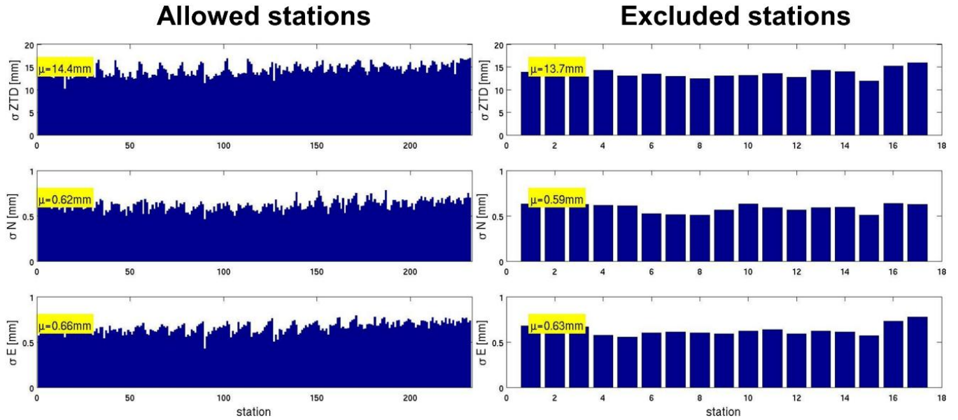
Figure A1. Station specific standard deviation of the Control run with dense network configuration. ZTD, North gradient, and East gradient of the allowed and excluded stations are shown on the left column and right column, respectively. The mean values are shown as text with the yellow background.
