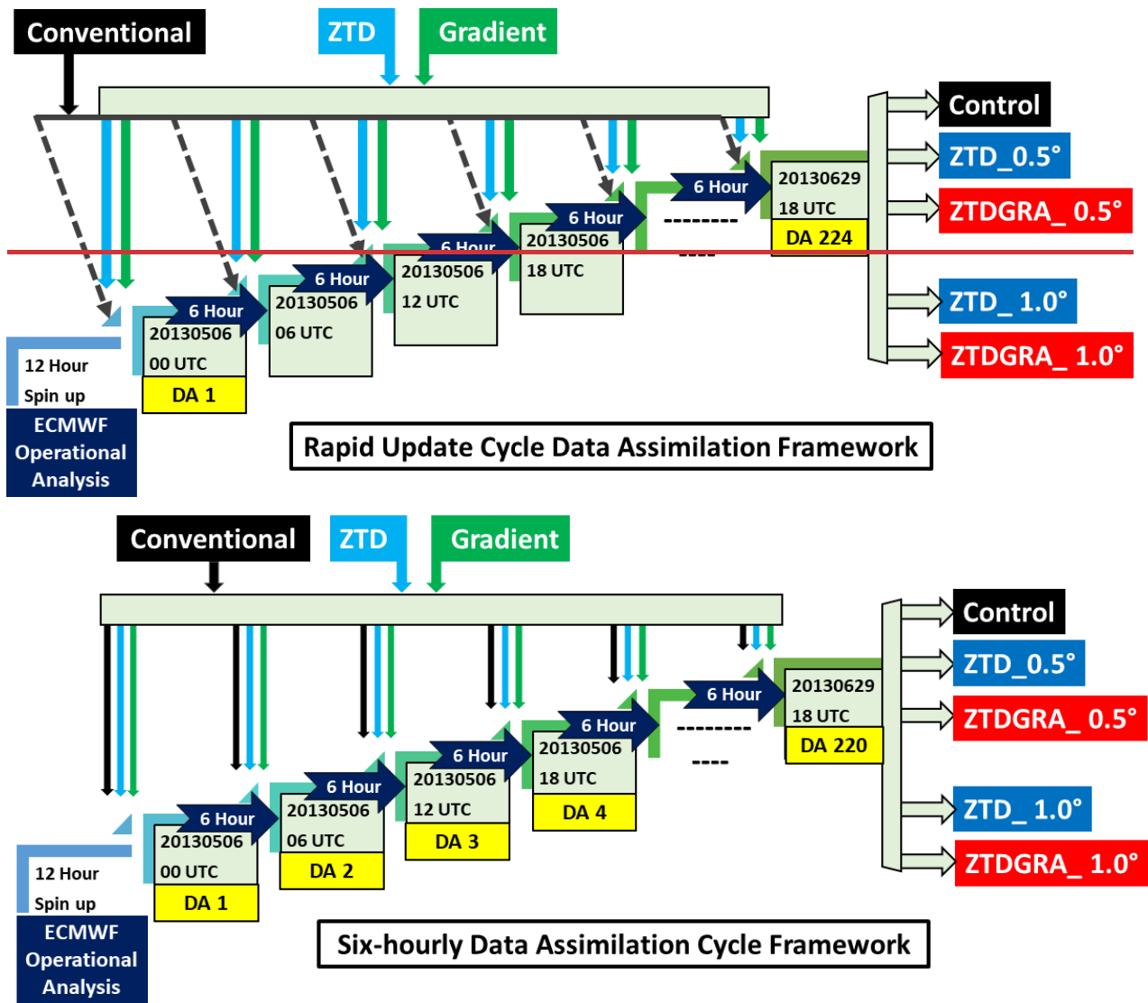
Figure 2. Schematic of the 3D-Var Six-hourly DA cycle rapid update cycle initialized from the ECMWF operational analysis. A spin-up of 12-h was performed until 00:00 UTC on 6 May 2013. Five experiments with different setups are performed in two sets. The first set comprises a control run assimilating conventional data, a ZTD_0.5° run assimilating ZTDs on top of the control run, and a ZTDGRA_0.5° run assimilating ZTD and TGs on top of the control run. These experiments are conducted with the observations from the (dense) 0.5-degree station network. The second set runs are ZTD_1_0° and ZTDGRA_1_0° with the assimilation of observations from the (sparse) 1-degree station network.
