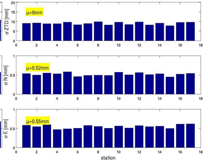
Figure A5. Same as Figure A1, but for ZTD run in the sparse network configuration.
