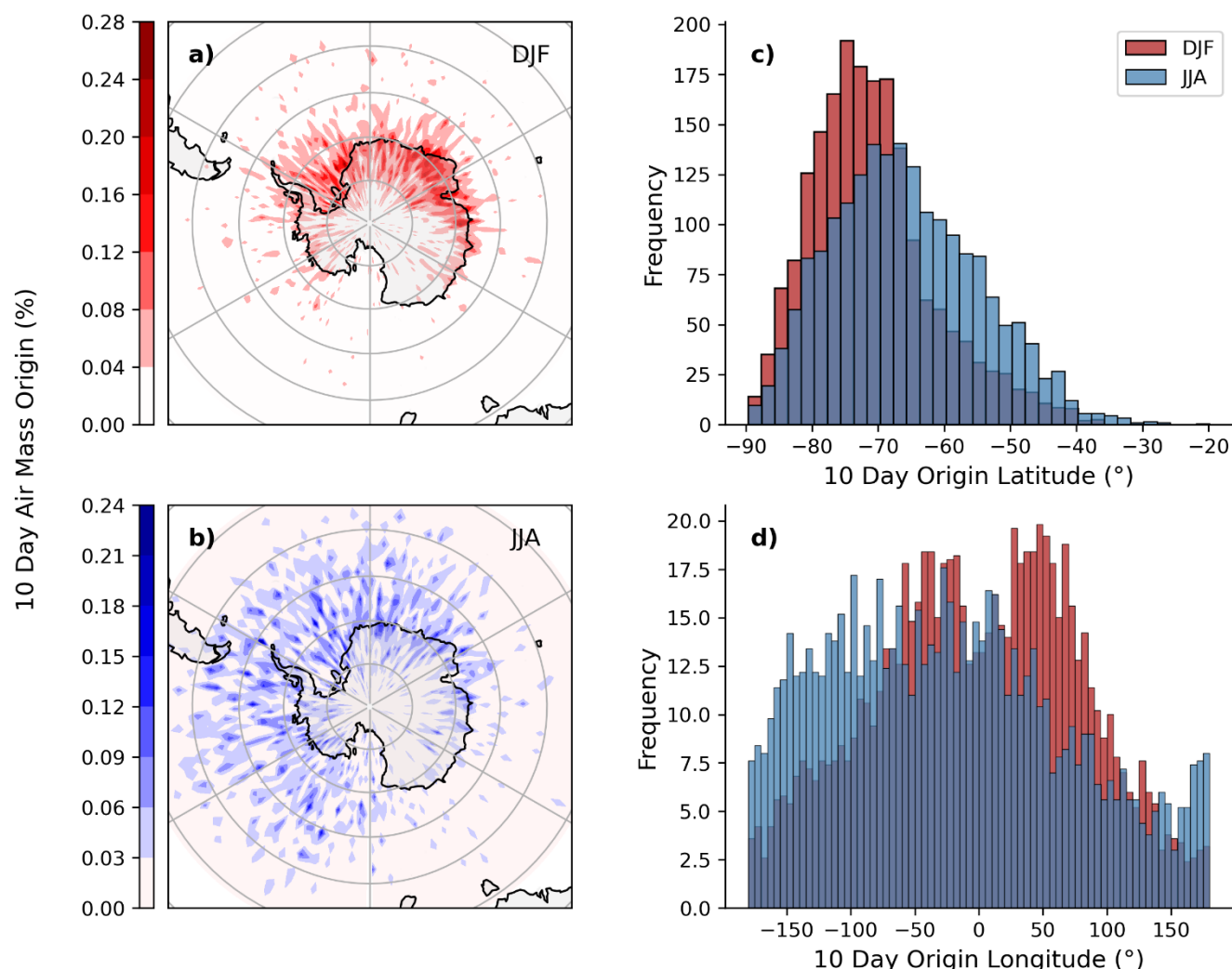
Figure 2a - d: NOAA HYSPLIT analysis of 10-day hourly back-trajectory of air masses to the South Pole from 1980 – 2020 (Rolph et al., 2017; Stein et al., 2015). Height elevation of back trajectory is 1000m. 2a and b indicate the percentage of 10-day air masses (240 hour) in a 2x2° grid. 2c and d are histograms of frequency of seasonal data by latitude and longitude, respectively.
