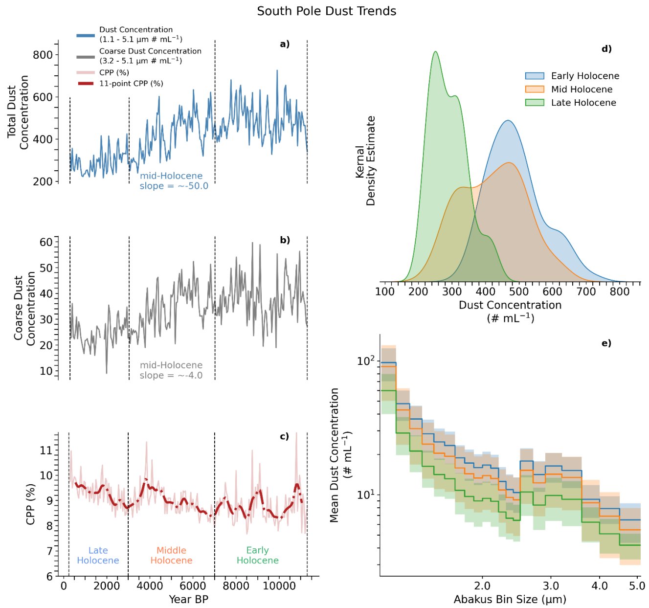
Figure 1a – e: 1a) 50-year median resampled SPC14 total dust concentration (1.1 – 5.1 \mu\text{m} # particles \text{mL}^{-1} ; blue line), 1b) 50-year median resampled coarse particle concentration (3.2 – 5.1 \mu\text{m} # particles \text{mL}^{-1} ; grey line), 1c) 50-year median resampled CPP (light
