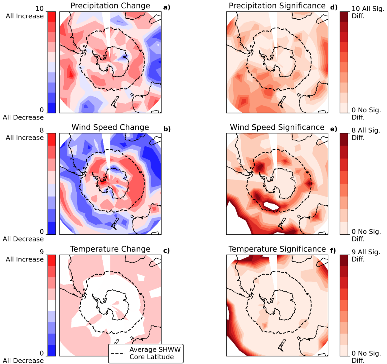
320 Figure 4a – f: CMIP6-PMIP4 models agreement displaying difference between mid-Holocene and piControl precipitation (4a), wind speed(4b), and temperature (4c; Otto-Bliesner et al., 2017; Brierley et al., 2020). Figure 4d – f highlights statistically significant 325 difference (p-value < 0.05) between mid-Holocene and piControl using a two-sided t-test. Data are from a 10 \times 10^\circ grid to account for original model grid resolution (Table 1). Figure 4a – c color bars indicate the number of models that infer a positive or no/negative change in each variable between 6000 years BP and during the Pre-Industrial. Red regions indicate a stronger model consensus towards an increase and blue indicates a consensus towards a decrease in the respective variable. Values in the middle represent a lack of consensus. Figures 4d – f color bars highlight the number of models showing a significant change in the specific region, where darker red indicates all models used show a significant change. The black dotted line represents the average position of peak surface wind speed for both time periods.
