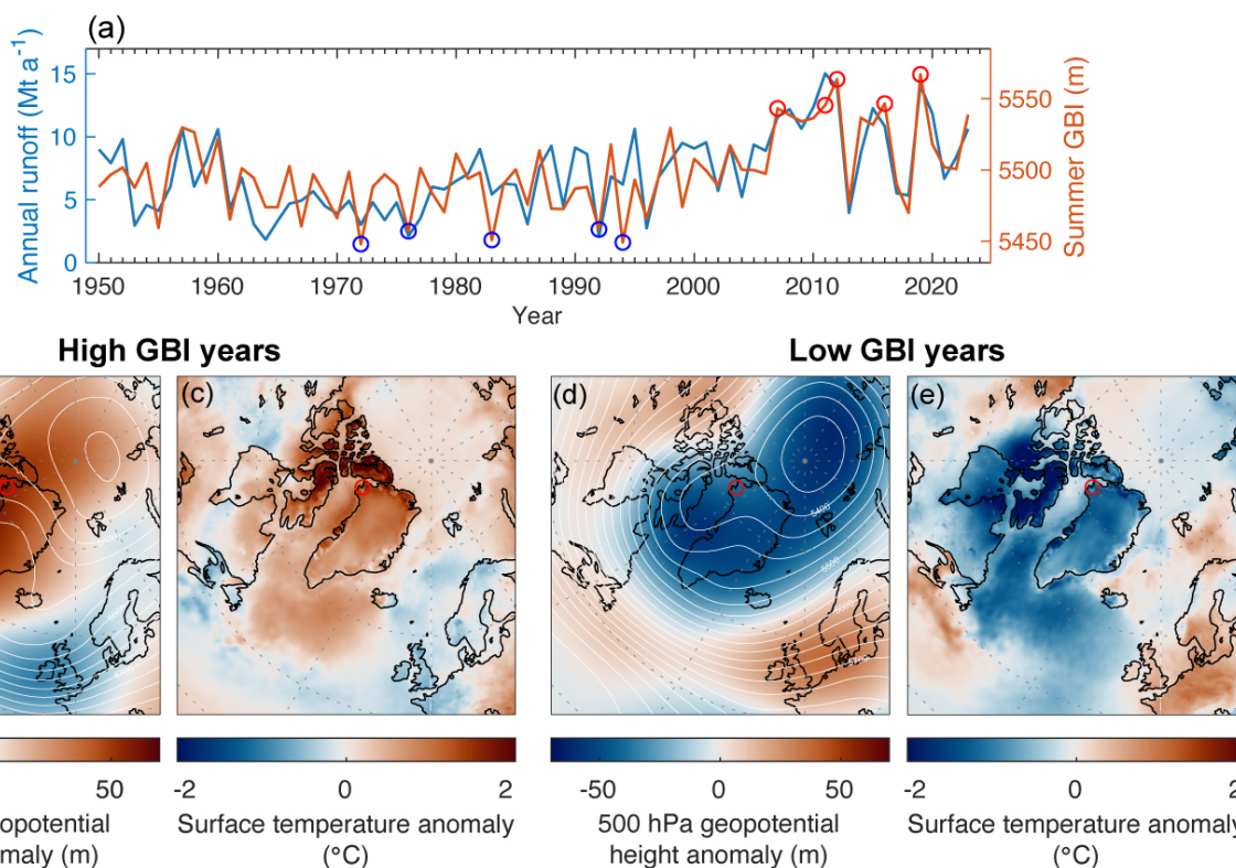
500 Figure 9: (a) Modelled annual runoff (blue line) and the Greenland Blocking Index (GBI) in summer (orange line). Circles indicate the five years with the highest (red) and lowest (blue) summer GBI. Composites of ERA5 reanalysis data for 500 hPa geopotential height (white lines) and its regression anomaly from the temporal trend (color) are shown for the five years with the (b) highest
