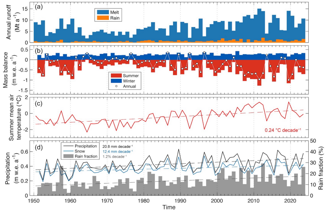
350 Figure 6: (a) Annual runoff and the contribution of snow/ice melt (blue) and rain (orange). (b) Calculated glacier-wide summer (red), winter (blue), and annual (dot) mass balances. (c) Summer mean air temperature at the SIGMA-B site taken from ERA5-Land. (d) Precipitation (black), snowfall (light blue), and rain fraction (bars) averaged over the catchment. The dashed lines in (c) and (d) are linear regressions of the data with p < 0.01 . The trend slope of the regression is also shown.
