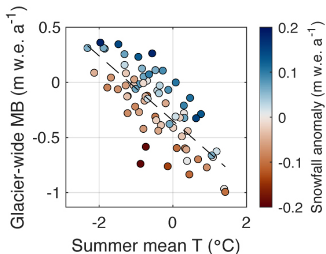
Figure 8: Summer mean air temperature (T) versus glacier-wide mass balance (MB). Symbol colors indicate the snowfall anomaly in the corresponding mass balance year.
