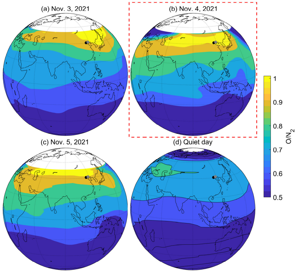
Figure 4. GUVI O/N_2 distribution in the Eastern Hemisphere. The observations on (a) 3 November, (b) 4 November, (c) 5 November, 2021 and (d) the quiet day for reference are displayed. The black and gray dots represent the locations of Yanqing and Pingquan, respectively.
