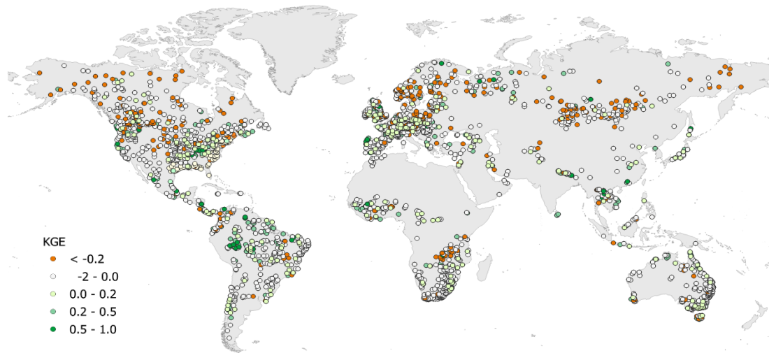
Figure 9: Kling-Gupta Efficiency (KGE) for simulated monthly river discharge ( \text{m}^3/\text{s} ) at global gauging stations. The map evaluates the performance of the uncalibrated global SWAT+ model for the 1982-1990 period against GRDC observations.
