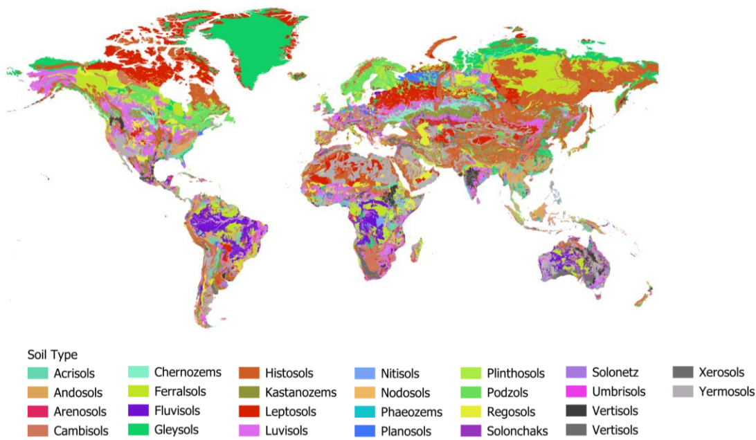
Figure 3: Global extent of FAO soil types (Fischer et al., 2008)
