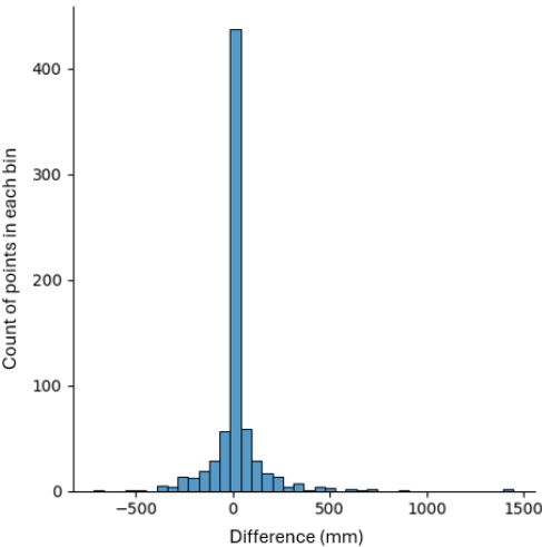
285 Figure 10: Distribution of differences between GLEAM v4 and SWAT+ simulated mean annual evapotranspiration (ET). The histogram shows the frequency of ET differences, calculated as (GLEAM - SWAT+), at sample points (shown in Figure 6) for the 1982-1990 period.
