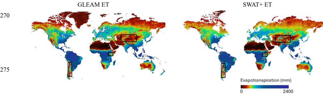
280 Figure 9: A comparison of the GLEAM v4 and SWAT+ ET maps. Highlighted regions show artefacts in the SWAT+ Output due to lack of representation of large water bodies and snow issues in high mountains.
