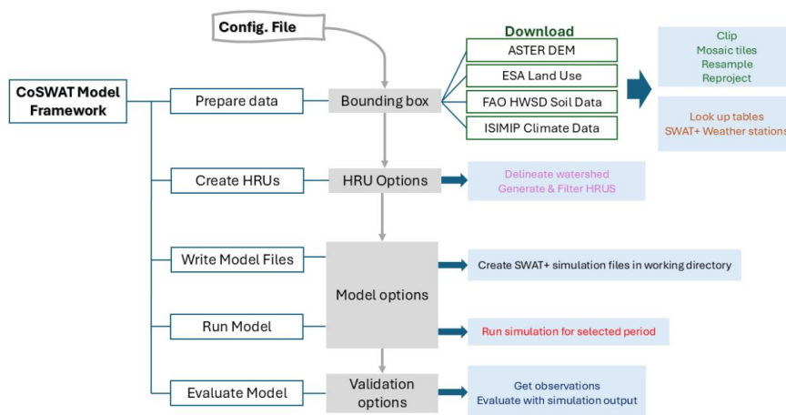
Figure 4: Schematic of the Community SWAT (CoSWAT) modelling framework. The flowchart illustrates the scripted workflow designed to automate the setup, execution, and evaluation of large-scale SWAT+ models. The entire process is controlled by a single configuration file, ensuring consistency and reproducibility.
