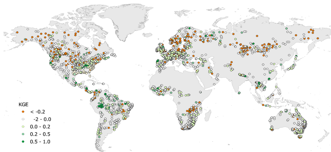
Figure 11: Kling-Gupta Efficiency (KGE) for simulated monthly river discharge ( \text{m}^3/\text{s} ) at global gauging stations. The map evaluates the performance of the uncalibrated global SWAT+ model for the 1982-1990 period against GRDC observations.
