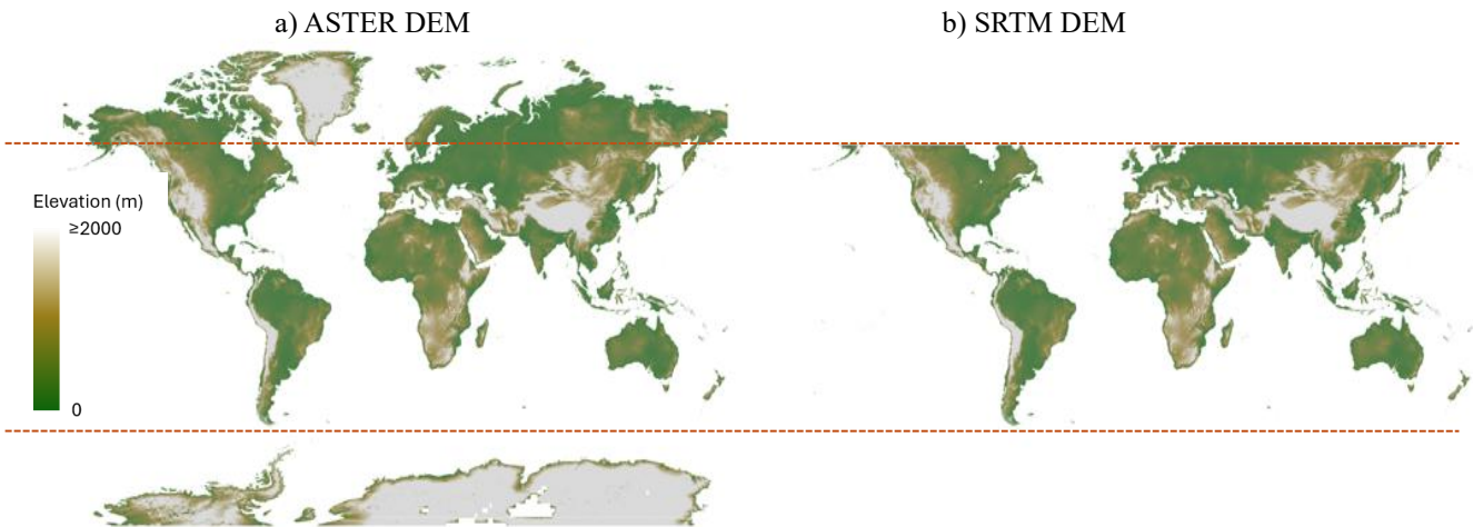
145 Figure 1: Spatial coverage of ASTER Global DEM vs SRTM. SRTM data only cover over 80% of the Earth's land surface (60°N–56°S), while ASTER goes further North and South (Yue et al., 2017).
