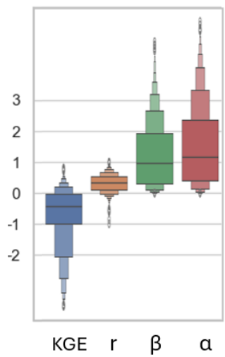
Figure 12: Distribution of river discharge performance metrics across all evaluated gauging stations. The boxenplots show the statistical distribution of the Kling-Gupta Efficiency (KGE) and its three components: the linear correlation coefficient ( r ), the variability ratio (alpha, \alpha ), and the bias ratio (beta, \beta ).
