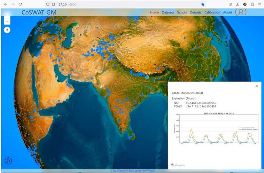
Figure 8: Django Web User Interface for visualising and managing the CoSWAT Global Model ( https://github.com/celray/coswat )
