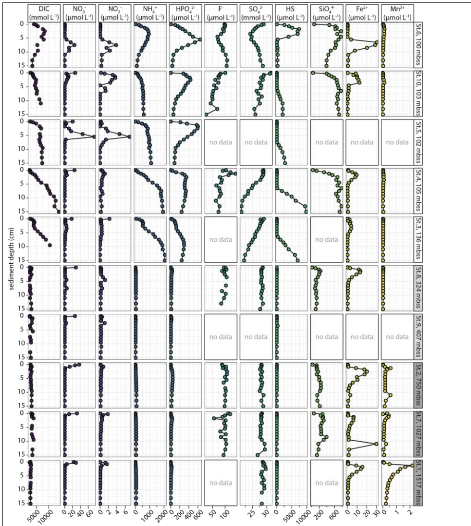
Figure 5: Key pore-water species plotted against sediment depth. Top data point is from bottom-water sample.
