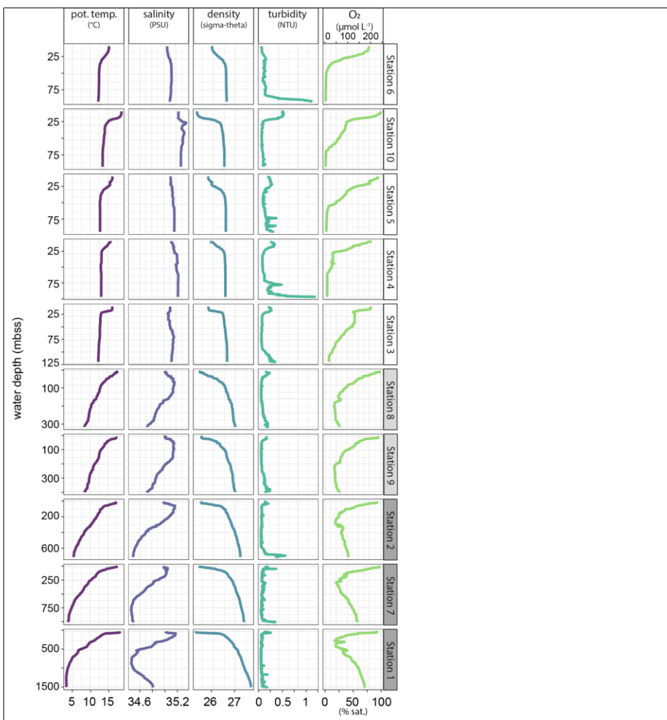
Figure 9: Profiles of key physical and chemical water-column properties plotted against water depth. Stations are in order of increasing water depth.
