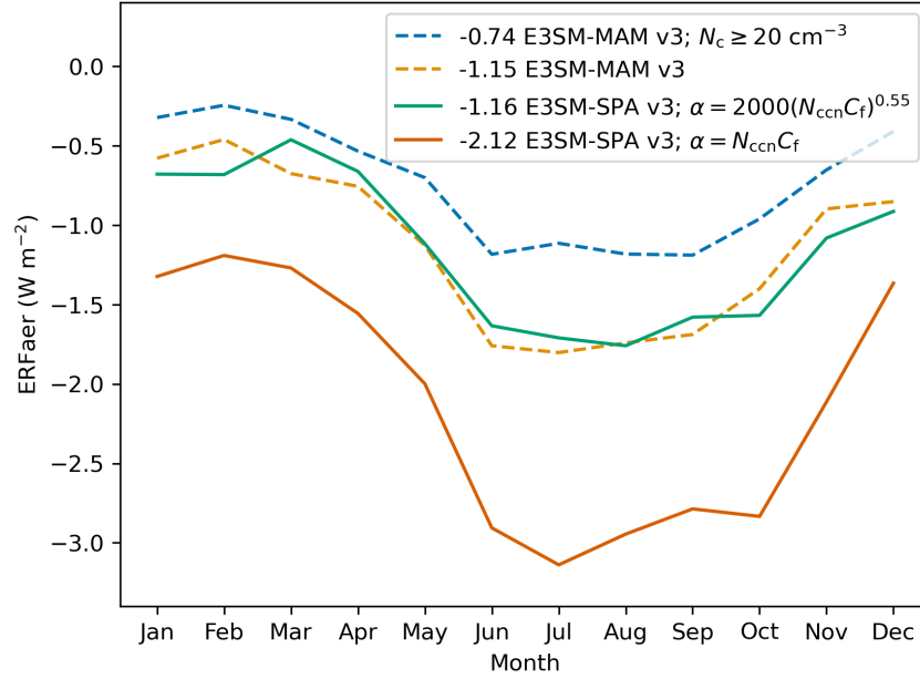
Figure 4. Like Figure 1, but for the E3SM v3 configurations tested.
