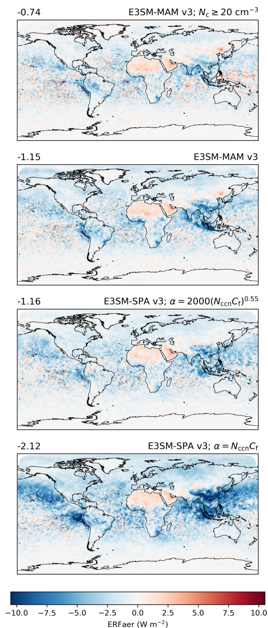
Figure 5. Like Figure 2, but for the E3SM v3 configurations tested.
