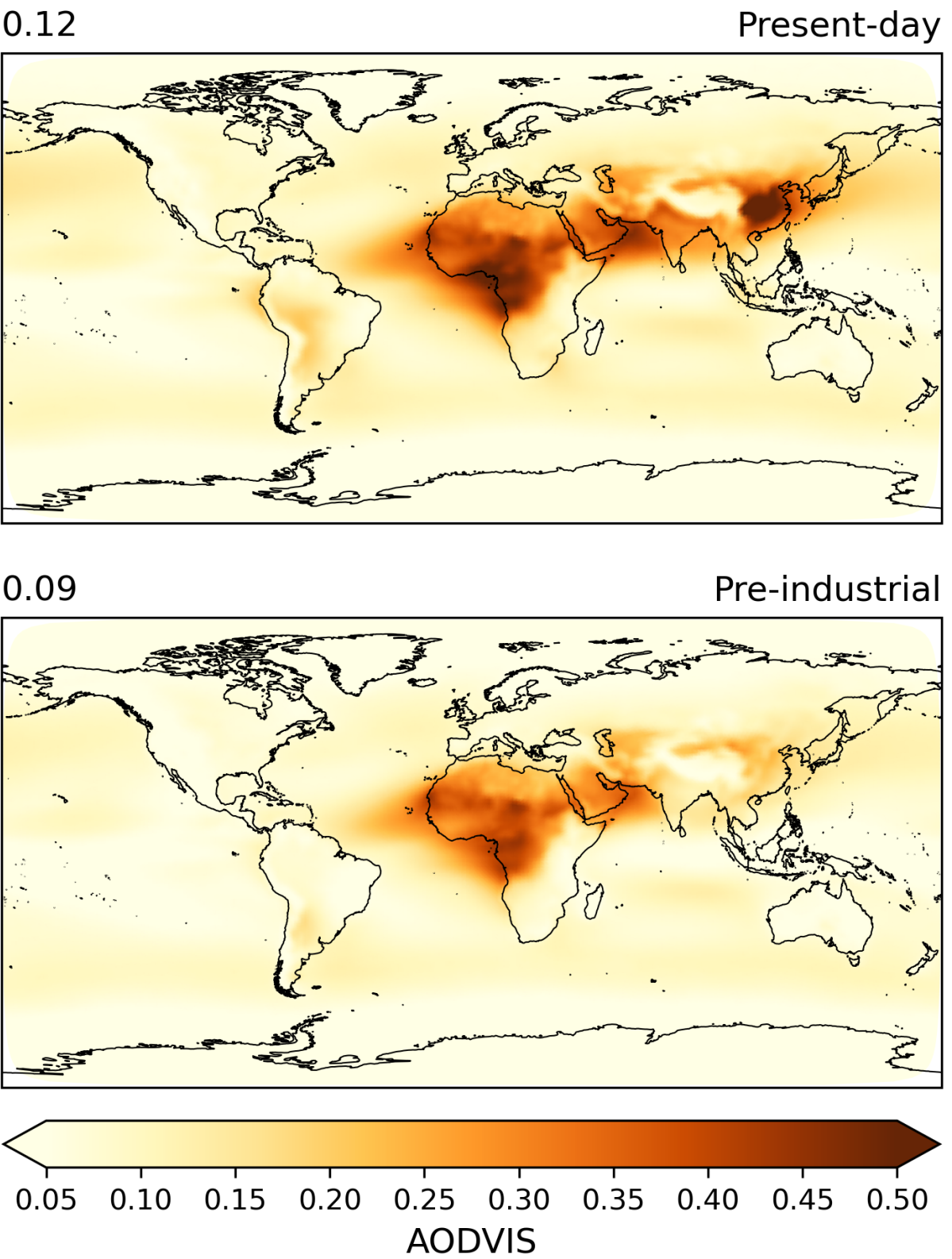
Figure 1: The aerosol optical depth at 550 nm for the present-day (top) and pre-industrial (bottom) scenarios. Comparing the two scenarios, we see a clear anthropogenic aerosol signal over China and India, and to lesser extent over South America and western Africa.
