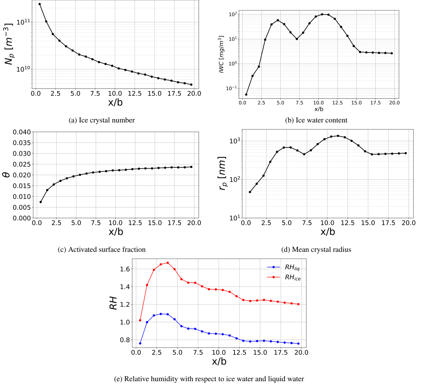
Figure 7. Microphysical quantities averaged in a cross-section of the plume contrail as a function of the distance behind the aircraft x
