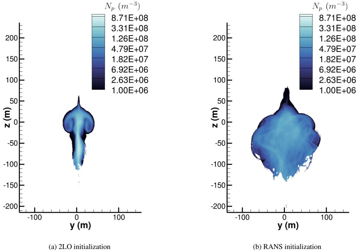
Figure 12. Spatially averaged ice crystal number field N_p in m^{-3} at t/t_b = 8 ( t_b = 25.7 s) and for N_b = 0.012 s ^{-1} . A logarithmic scale is used for the color levels.
