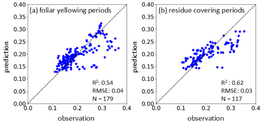
380 Figure 2 The comparison of daily surface albedo ( \alpha_{surf} ) predictions based on the new parameterization (Fig. 1) with independent observation from 5 sites in Europe during (a) the foliar yellowing and (b) residue covering periods, with coefficient of determination ( R^2 ) and root mean square error ( RMSE ) in the bottom-right corners. The dotted black line is the 1:1 line.
