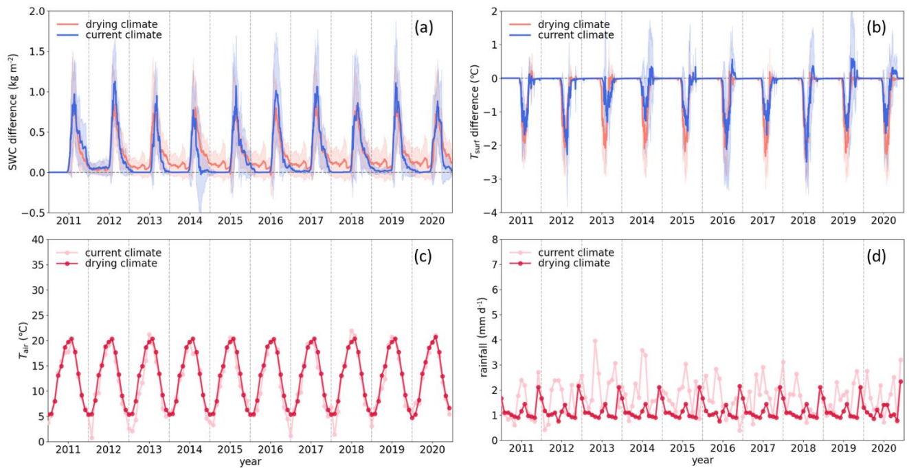
Figure 5 The 10-year cumulative effect of new parameterization of surface albedo ( \alpha_{surf} ), surface roughness ( Z_0 ) and soil conductance ( \beta_4 ) on (a) soil water content ( SWC ) and (b) simulated daily soil temperature ( T_{soil} ) at 12.5 % soil depth under current and drying climate scenarios at 6 sites from 2011 to 2020. Monthly temperature and rainfall are obtained from the meteorological variables of 6-hourly 0.5^{\circ} CRU-JRA product (v2.4), shown in (c) and (d). Shown are differences between results from ORC-AE and ORC-D. ORC-AE represents the new model version with effects of the modified \alpha_{surf} and the refined \beta_4 and Z_0 , while ORC-D suggests the initial version of the model.
