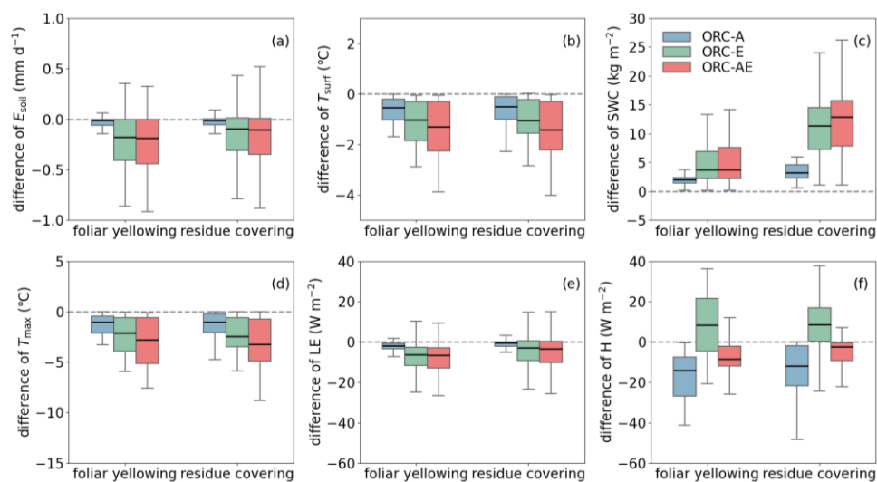
457 458 Figure 4 The average effect of model improvements for yellowing and residues cover on daily soil evaporation ( E_{soil} ), surface 459 temperature ( T_{surf} ), the total soil water content up to 2 m ( SWC ), the maximum daily surface temperature ( T_{max} ), the latent 460 heat flux ( LE ) and the sensible heat fluxes ( H ) across 12 sites. Shown are the simulated differences between three 461 configurations of the refined model and old model: ORC-A represents the effect of the modified surface albedo ( \alpha_{surf} ), ORC- 462 E shows the effect of refined soil conductance ( \beta_k ) and surface roughness ( Z_0 ), and ORC-AE indicates suggests the effect of 463 both modifications. The solid and dotted black lines within each box indicate the mean and median daily values across sites 464 and timepoints, respectively. The box spans the interquartile range, covering the 25th percentile (lower bound) to the 75th 465 percentile (upper bound). Black crossbars at the top and bottom represent the dataset's minimum and maximum values. The 466 grey dotted vertical line in each plot represents zero on the y-axis.
