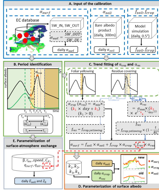
Figure 1 The procedure of parameterization of crop and residue albedo ( \alpha_{surf} and \alpha_{res} ), soil evaporation ( E_{soil} and E_{soil} ) and surface roughness ( Z_0 and Z_0 ) in the ORCHIDEE-CROP model. Panel (A) illustrates the input datasets for albedo calibration. \alpha_{soil} and \alpha_{surf} are bare soil albedo ( \alpha_{soil} ) and surface albedo ( \alpha_{surf} ), respectively. f_{crop} and f_{soil} are the gridded fractions of crop ( f_{crop} ) and residues ( f_{res} ), respectively. SW\_IN and SW\_OUT are half-hourly incoming ( SW\_IN ) and outgoing ( SW\_OUT ) solar radiation observed at 7 eddy-covariance (EC) sites. Panel (B) shows the identification of foliar yellowing and residue covering periods based on time series of \alpha_{surf} (black curve) and leaf area index (LAI, green curve). T_{0-5} represent the dates of maximum LAI ( T_0 , green dotted vertical line), albedo increase start ( T_1 , orange dotted vertical line), harvest ( T_2 , black-grey dotted vertical line) and albedo increase end ( T_3 , shallow-blue dotted vertical line), 30 days after harvest ( T_4 , grey solid vertical line) and tillage (equals to 90 if no tillage) ( T_5 , dark-blue dotted vertical line). \alpha_{min} and \alpha_{max} are the minimum and maximum surface albedo on T_1 and T_3 . The shallow-green, orange, yellow and brown areas show the conceptual growing, maturity, residue covering and bare soil periods of winter wheat. Panel (C) describes trend fittings for crop albedo ( \alpha_{crop} ) and \alpha_{res} . Features in two plots have the same meanings with the ones in Panel (B). f_{crop, yellowing} is the fraction of crop during the foliar yellowing period. RC is the duration of T_2 and T_5 . k_1, k_2, k_3 and k_4 are the fitting parameters during foliar yellowing and residue covering periods. Day and t are the days since T_1 and T_2 . Panel (D) illustrates
