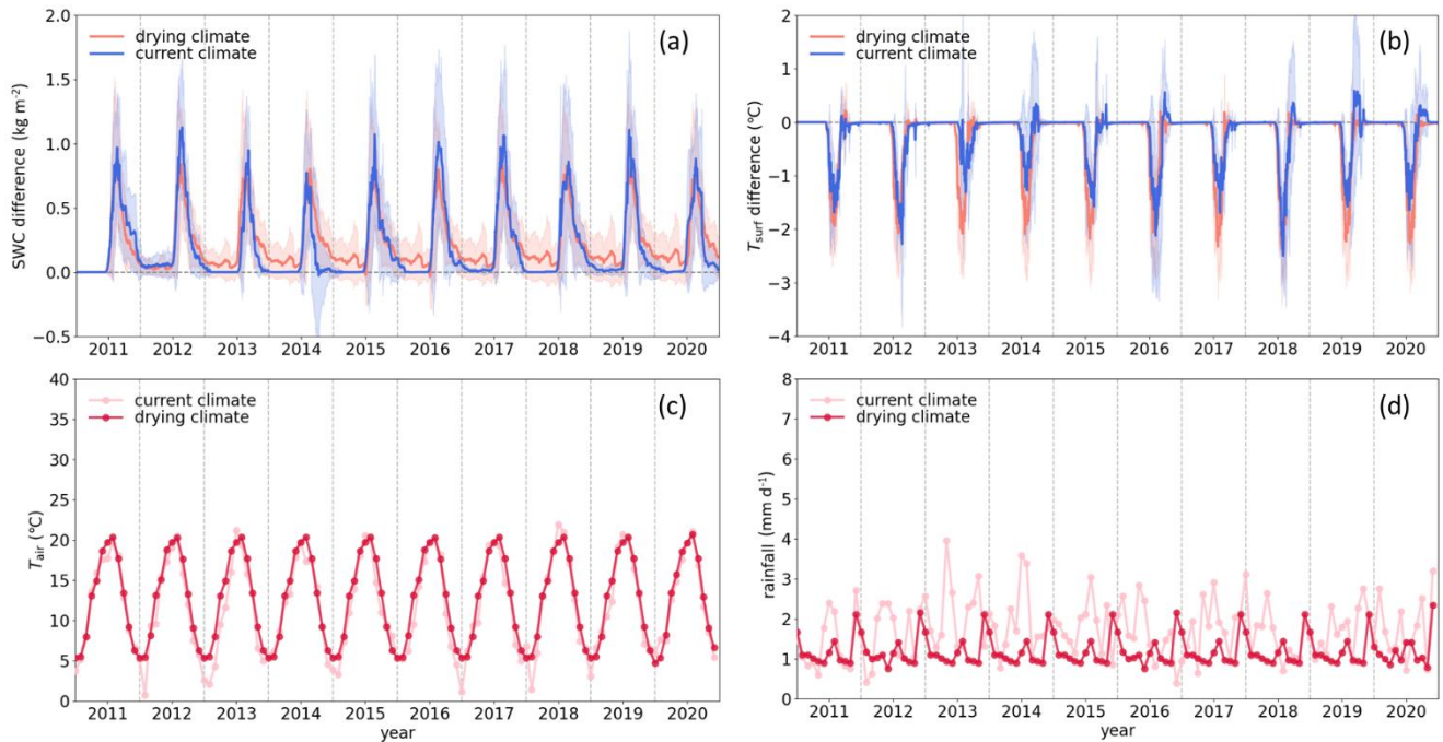
Figure 5 The 10-year cumulated effect of new parameterization of surface albedo ( \alpha_{surf} ), surface roughness ( Z_0 , Z_0 ) and soil conductance ( \beta_4 ) on (a) soil water content ( SWC ) and (b) simulated daily soil temperature ( T_{soil} ) at 12.5 % soil depth under current and drying climate scenarios at 6 sites from 2011 to 2020 . Monthly temperature and rainfall are obtained from the meteorological variables from 6-hourly 0.5° CRU-JRA product (v2.4) , shown in (c) and (d), respectively . Shown are differences between results from ORC-AE and ORC-D. ORC-AE represents the new model version with effects of the modified \alpha_{surf} and the refined \beta_4 and Z_0 , while ORC-D suggests the initial version of the model. ORC-AE represents the effect of the modified \alpha_{surf} , \beta_4 and Z_0 . ORC-D is the old model.
