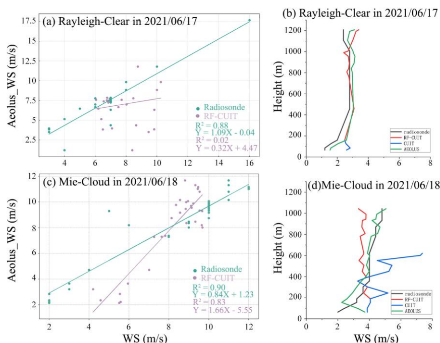
390 Fig. 9. The relationship between interpolated CUIT Lidar, radiosonde, and Aeolus satellite data in the (a) Rayleigh and (c) Mie channels; and (b, d) a profile plot from a single radiosonde observation.
