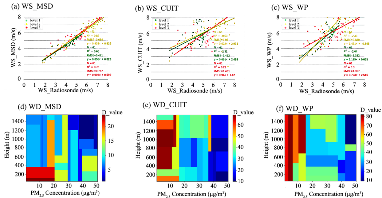
Fig 5. Comparison of radiosonde data with CUIT, MSD, WP (a-c) WS, and (d-f) WD at different heights and PM 2.5 concentrations.
