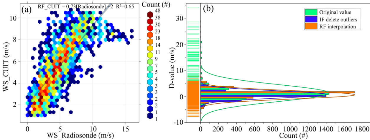
Fig. 8. (a) WS scatter plot of CUIT Lidar and radiosonde after processing; (b) Comparison distribution map of the difference between CUIT and radiosonde after IF and RF processing.
