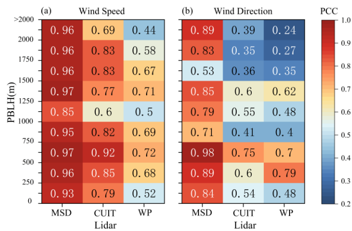
Fig. 6. Comparison of (a) WS and (b) WD between radiosonde data and CUIT Lidar, MSD Lidar, and WP Lidar at different PBLH; Color bar represents Pearson correlation coefficient.
