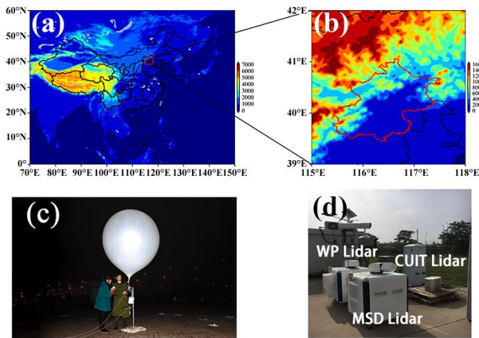
Fig. 1. Location of the Nanjiao Observatory and instruments deployed during the campaign. Location and instruments of the radiosonde station.
