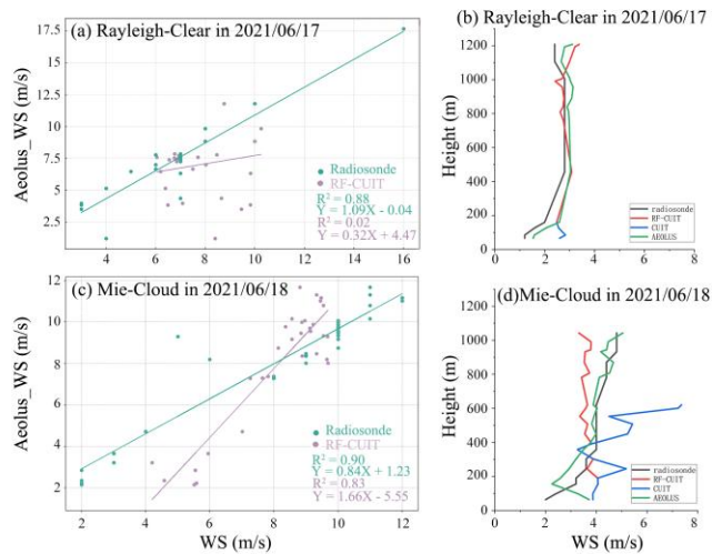
Fig. 9. The relationship between interpolated CUIT Lidar, radiosonde, and Aeolus satellite data in the (a) Rayleigh and (c) Mic channels; and (b, d) a profile plot from a single radiosonde observation.
