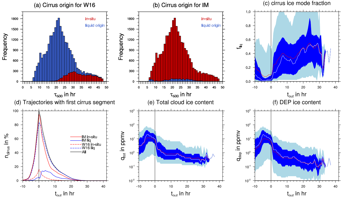
Figure 7. Histogram of WCB ascent timescale \tau_{600} with-colored by cirrus cloud origin according to (a) W16 and (b) our ice modes based classification , respectively. Panel (c) shows the liquid origin fraction as a function of time after ascent t_{out} with the mean (median) indicated by a red (white) line and the 25 th to 75 th (5 th to 95 th ) percentile range by dark (light) blue shading. Panel (d) shows the percentage of trajectories containing a (first) cirrus segment in the outflow for all segments (black), ice modes in-situ (red), ice modes liquid origin (blue), W16 in-situ (red dashed), W16 liquid origin (blue dashed). Panels (e) and (f) show the total ice water content and the ice water content of DEP, respectively.
