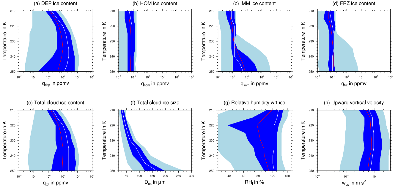
Figure 6. Statistics of the ice-water-mass content of the different ice modes q_{dep} , q_{hom} , q_{imm} , q_{frz} , the total cloud ice mass content q_{tot} , mean cloud ice size D_{tot} , relative humidity wrt ice RH_i and upward vertical velocity w_{up} as a function of temperature. The median (mean) of each variable is shown by the white (red) line, the 25 th to 75 th percentile range by dark blue shading and the 5 th to 95 th percentile in light blue shading.
