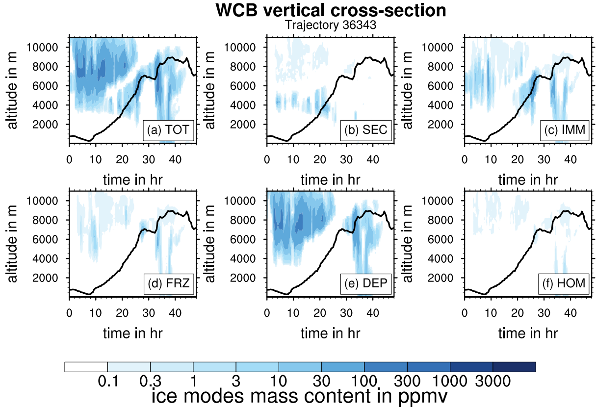
Figure 4. Vertical cross-section of the WCB along a sample trajectory. Profiles are co-located in time and horizontal position with the shown air parcel, the altitude of which is indicated by the black line. Cloud ice mass content for the five ice modes as well as the sum of all ice modes (TOT) is shown by the color coding in the different panels.
