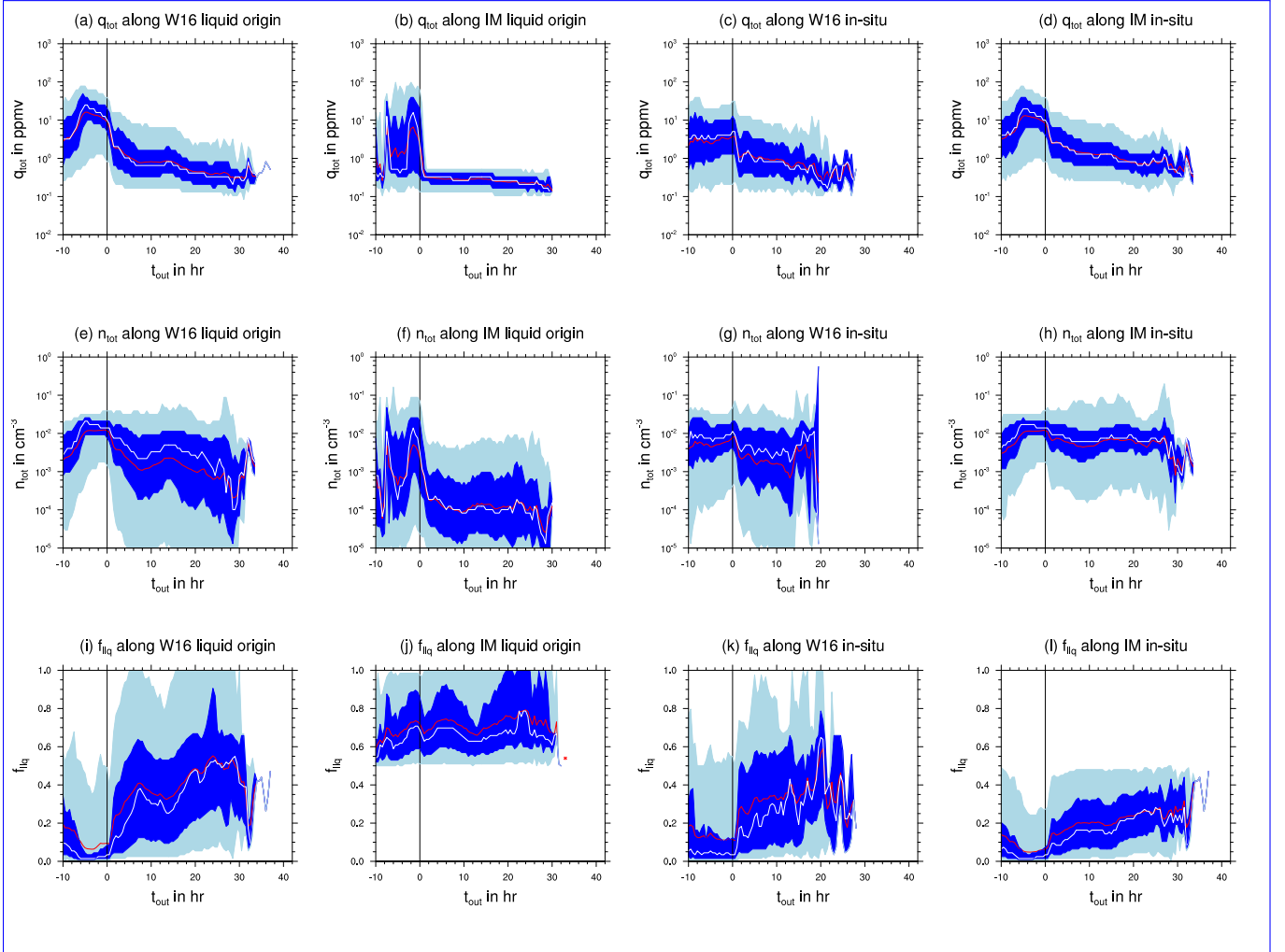
Figure 8. Statistics of total ice mass content q_{tot} (a-d), total ice number density-concentration n_{tot} (e-h) and liquid-origin-liquid-origin fraction f_{liq} (i-l) along liquid-origin-liquid-origin and in-situ sections as identified by W16 (first and third column) and ice-modes-based-the IM method (second and fourth column) for the first cirrus segment after end of ascent. The median (mean) of each variable is represented by the white (red) line, and the 25 th -25 th to 75 th -75 th (5 th -5 th to 95 th -95 th ) percentile range by dark (light) blue shading.
