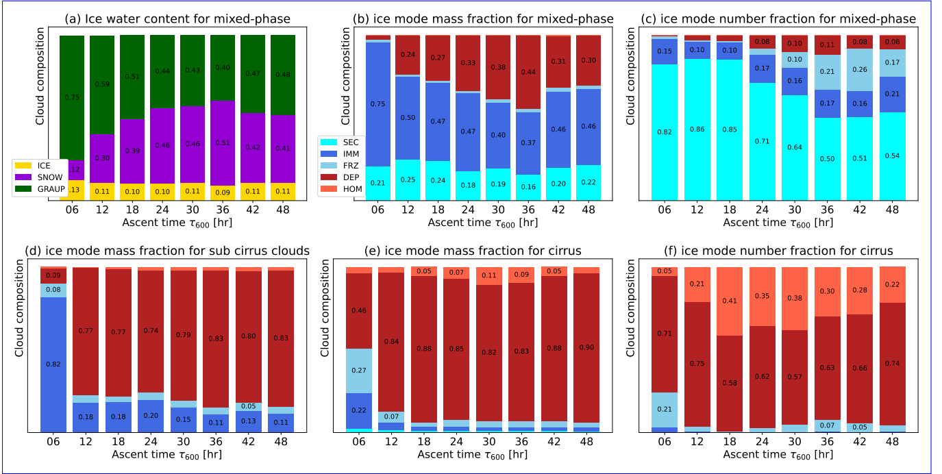
Figure 5. Relative contribution-Volume integrated ratios of the different frozen hydrometeor types (a) and different ice modes (b-f) to-for the ice-mass content (a, b, d, e) and ice-number concentrations (c, f) as function of the ascent timescale \tau_{600} . Panels (a-c) show results for mixed-phase clouds, panel (d) for the pure ice-cloud-ice-clouds at sub-cirrus temperatures, and panel (e, f) for cirrus clouds. We only display value labels for relative contributions \geq 0.05 . The x-axis labels signify the upper limit of the respective ascent timescale bin.
