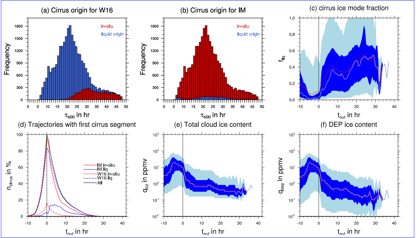
Figure 7. Histogram of WCB ascent timescale \tau_{600} colored by cirrus cloud origin according to (a) W16 and (b) our ice modes based classification, respectively. Panel (c) shows the liquid-origin-liquid-origin fraction as a function of time after ascent t_{out} with the mean (median) indicated by a red (white) line and the 25 th 25 th to 75 th 75 th (5 th 5 th to 95 th 95 th ) percentile range by dark (light) blue shading. Panel (d) shows the percentage of trajectories containing a (first) cirrus segment in the outflow for all segments (black), ice modes in-situ (red), ice modes liquid origin (blue), W16 in-situ (red dashed), and W16 liquid origin (blue dashed) segments . Panels (e) and (f) show the total ice water content and the ice water content of DEP, respectively.
