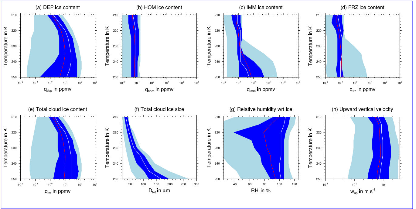
Figure 6. Statistics of the mass content of the different ice modes (a) q_{dep} , (b) q_{hom} , (c) q_{imm} , (d) q_{frz} , (e) the total cloud ice mass content q_{tot} , (f) mean cloud ice size D_{tot} , as well as (g) relative humidity wrt ice RH_i and (h) upward vertical velocity w_{up} as a function of temperature. The median (mean) of each variable is shown by the white (red) line, the 25 th –25 th to 75 th –75 th percentile range by dark blue shading and the 5 th –5 th to 95 th –95 th percentile in light blue shading.
