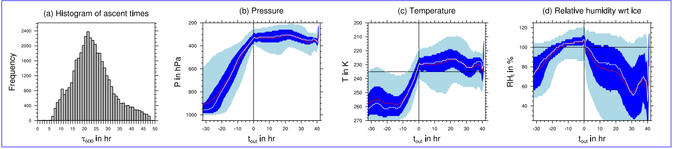
Figure 3. (a) Histogram of WCB (fastest) ascent time-times \tau_{600} . Statistics along WCB trajectories for (b) pressure p , (c) temperature and (d) relative humidity with respect to ice RH_i are shown as a function of outflow time t_{out} . The median is indicated by a white line, the mean by a red line. The 25 th -25 th to 75 th -75 th percentile range is indicated by dark blue shading and the 5 th -5 th to 95 th -95 th percentile in light blue shading.
