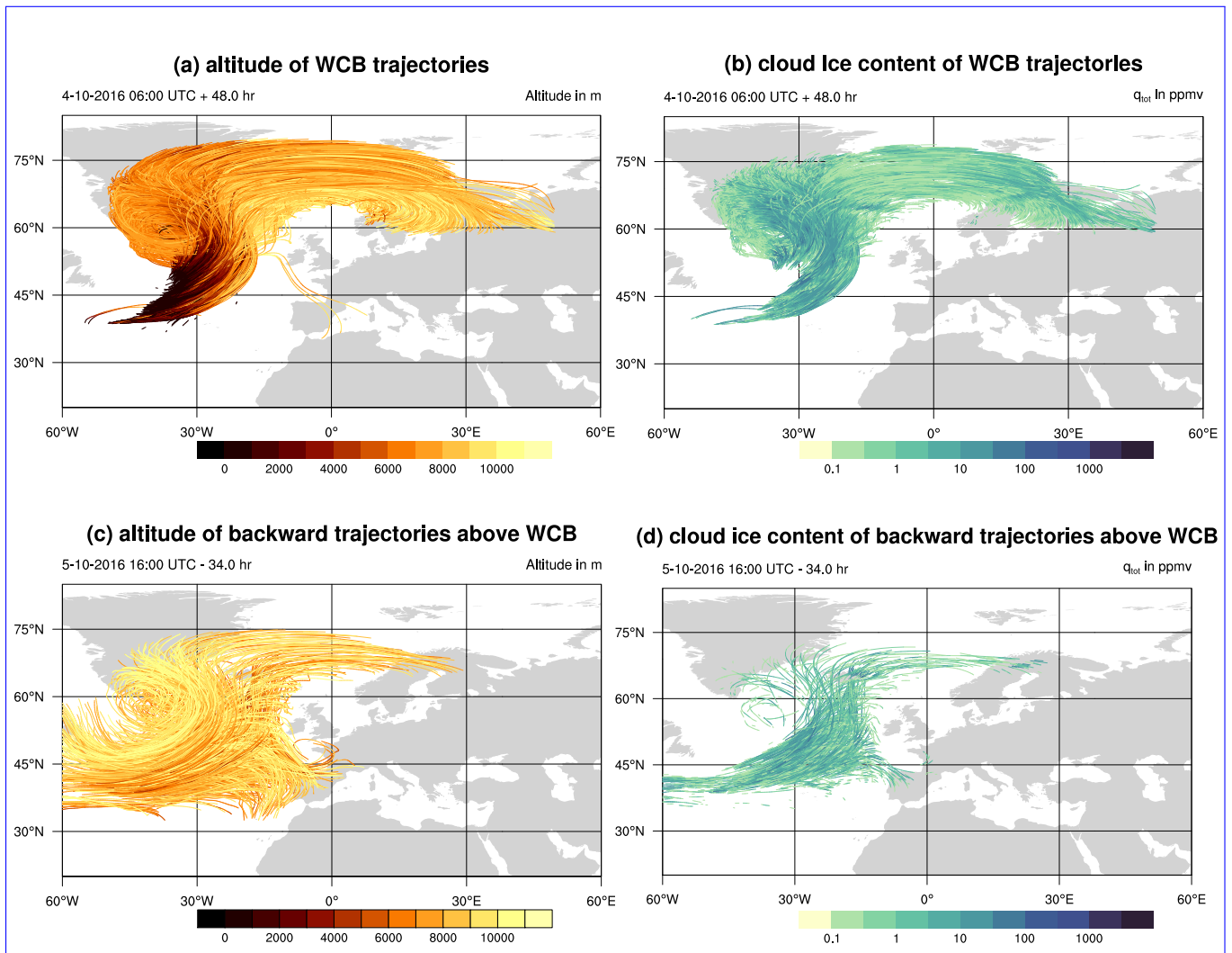
Figure 2. WCB trajectories starting at 4 th 4 th October 06:00 UTC (a,b) and backwards trajectories started above the WCB at 5 th 5 th October 16:00 UTC (c,d). Colored Trajectories are colored according to altitude (a,c) and total cloud ice content (b,d), respectively. Only randomly selected 5% of all trajectories used in the analysis are shown.
