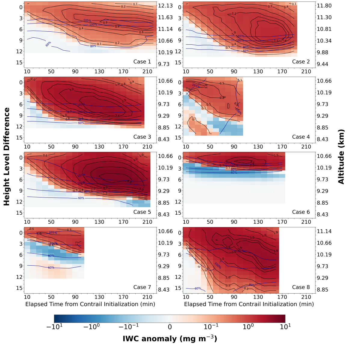
Figure 10. Time–height evolution of contrail ice water content anomalies ( \text{IWC} \Delta \text{IWC} ) anomalies for different cases, defined as the difference between the perturbation (contrail) and control (natural cloud) runs over the same region. The x-axis shows time since contrail initialization; the y-axis shows height level differences from flight height. Black contours denote IWC anomalies ( \text{mg m}^{-3} ), and blue contours indicate \text{RH}_{\text{ice}} (%) from the control run. Warm colors indicate positive anomalies; cool colors indicate negative ones.
