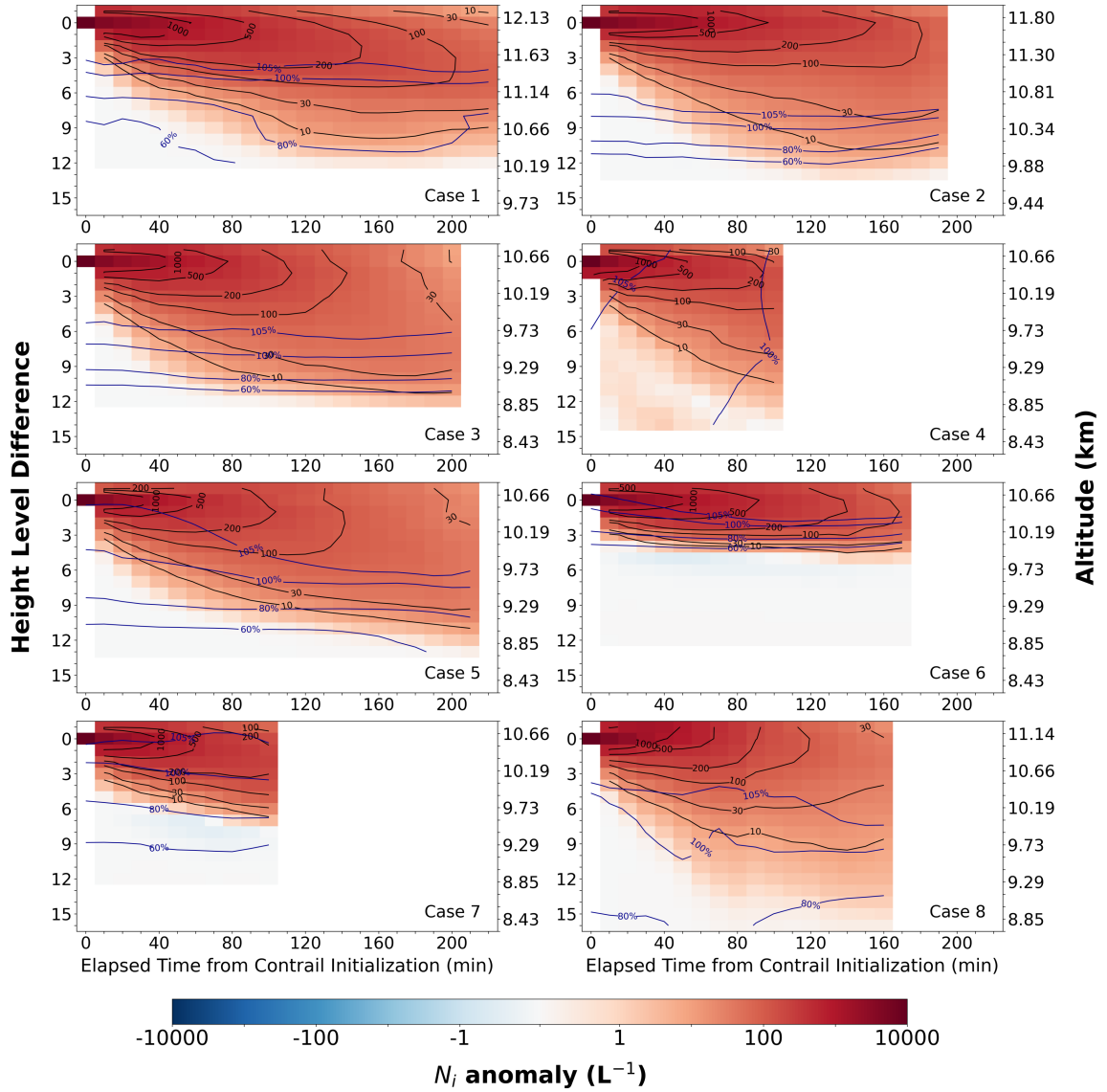
Figure 8. Time–height evolution of contrail ice crystal number concentration anomalies ( N_i \Delta N_i ; perturbation minus control) anomalies for different cases, defined as the difference between the perturbation (contrail) and control (natural cloud) runs over the same region. The x-axis shows time since initialization; the y-axis shows height level differences from flight height. Black contours denote N_i anomalies; blue contours show RH_{ice} (%) from the control run. Warm colors indicate positive N_i anomalies; cool colors indicate negative ones.
