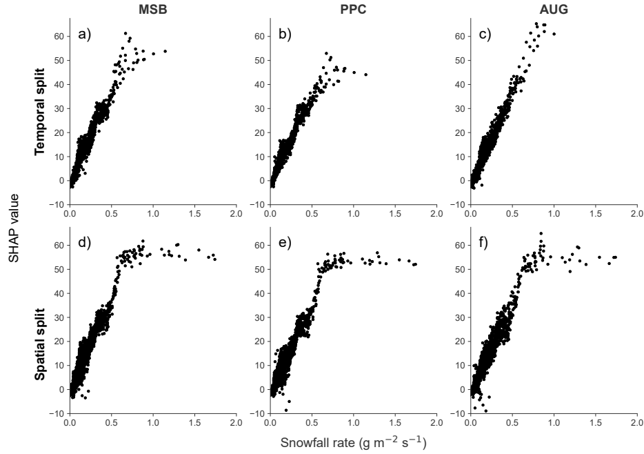
Figure 8. Scatter plot of the SHAP values against measured values of the daily averaged snowfall rate. The SHAP values quantify the deviation in the predicted \Delta SWE from its average value over the test samples, as caused by the specific value of the snowfall rate in each of them. The three ML-based setups are compared for both temporal (a-c) and spatial (d-f) data splits.
