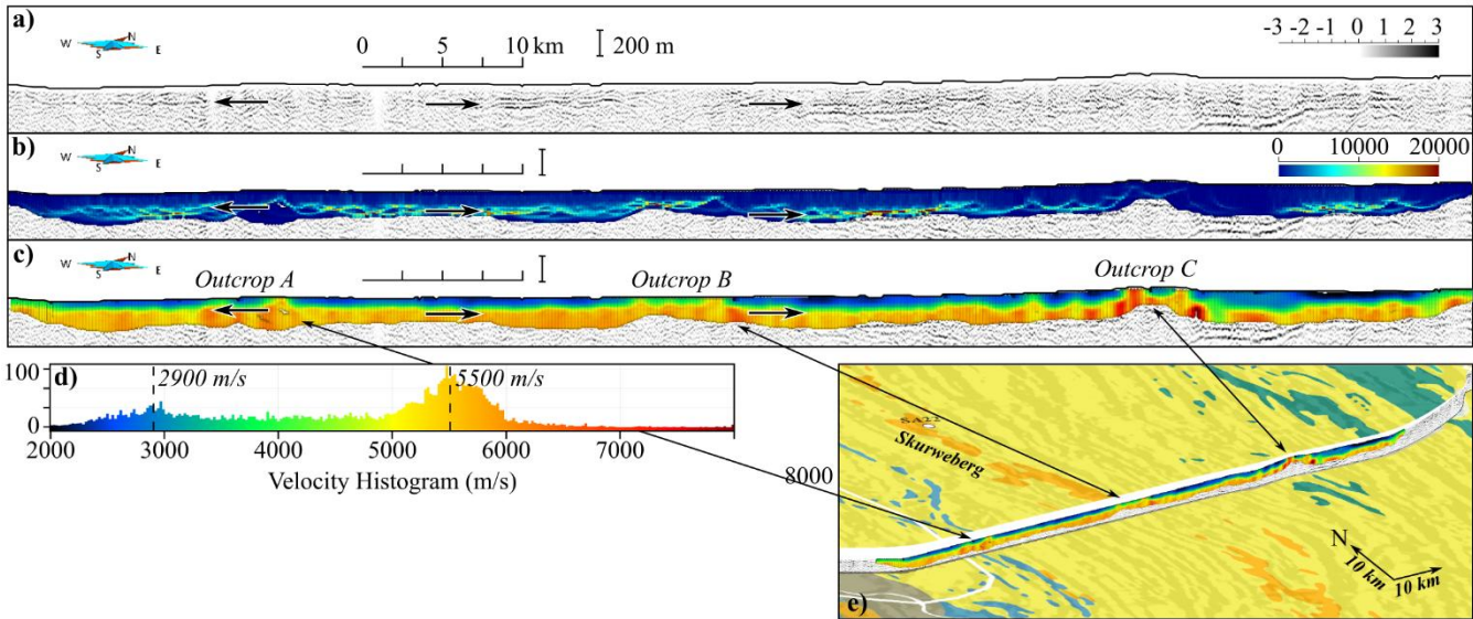
480 Figure 11: Results of the first-break traveltime tomography, showing (a) the reflection section, (b) the computed raypath count, and (c) the velocity field. The colourbar for (c) is plotted as a histogram in (d), and (e) shows the velocity results overlaid on the geology map from Figure 2 to illustrate outcrops. Black arrows delineate a strong lateral velocity contrast that are coincident with regions of reflectivity.
