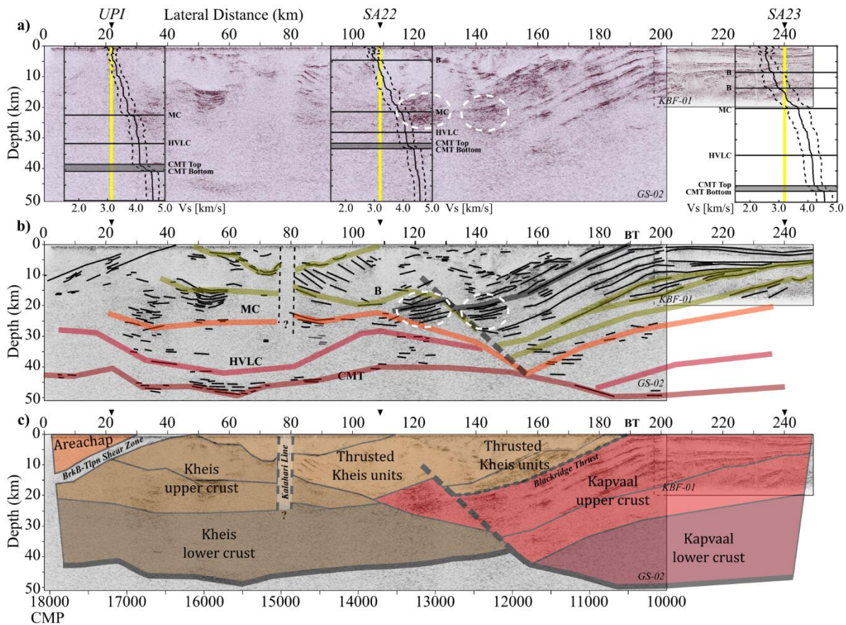
585 Figure 12: First-order crustal interpretation based on integrated reflection seismic and RF results. From top to bottom, (a) shows the seismic station inversion results overlaid on the reflection seismic section, (b) shows the interpolated horizons of the RF results, and (c) shows the resulting crustal model.
