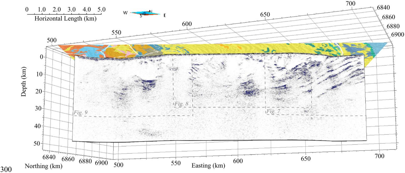
Figure 5: The amplitude envelope, or instantaneous amplitude, of the reprocessed GS-02 seismic section plotted in 3D space. Boxes indicate portions of the profile that are enlarged in subsequent images. Plotted on top of the seismic section is the geological map as in Figure 2.
