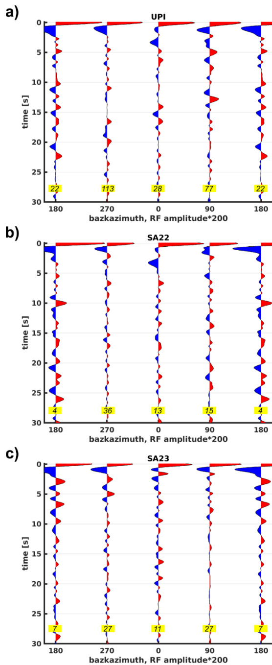
Figure A2: Backazimuth plots of RFs at stations UPI (a), SA22 (b) and SA23 (c). The RFs were stacked in bins of four quadrants pointing to the north (-45 to 45 degrees with respect to north), south (135 to 225 degrees), east (45 to 135 degrees) and west (225 to 315 degrees). Italic numbers with a yellow background indicate the number of events in each stack. Stacks of more RFs are naturally more robust representations than stacks with fewer events. Note that the southern quadrant is represented twice at 180 degrees.
