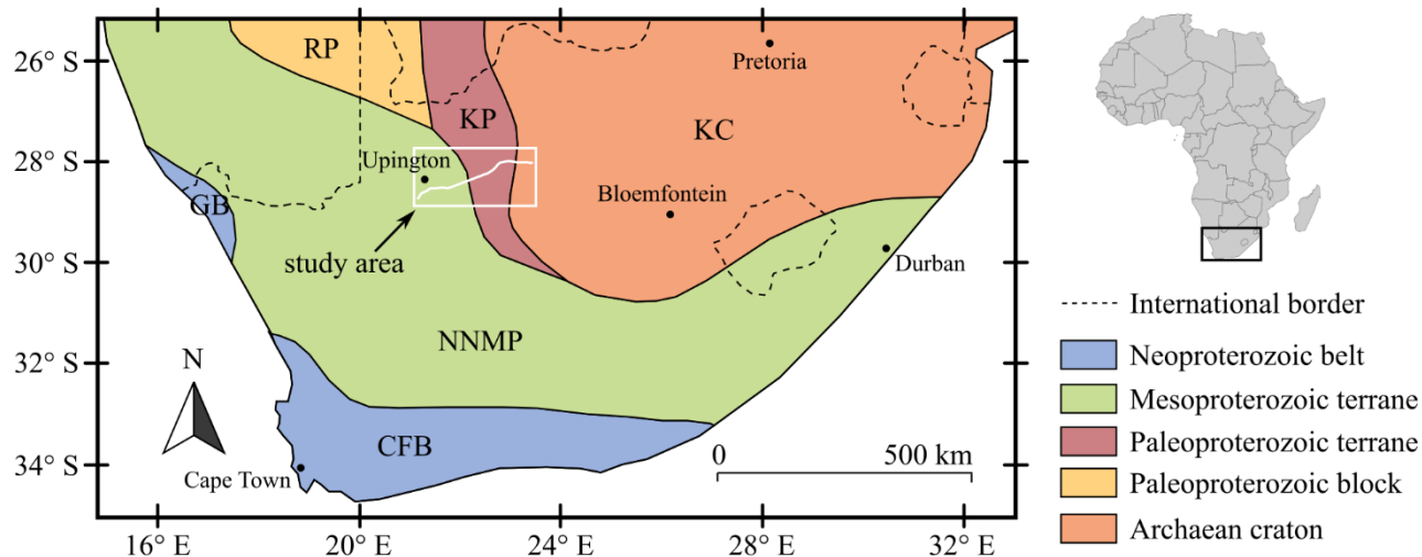
Figure 1: Map showing the major tectonic provinces of southern Africa and the location of our study region, along with the seismic profiles overlaid in unicolour white (Figure 2 shows independent profiles). RP Rehoboth Province; KP Kheis Province (here inclusive of the Kaaieen Terrane); KC ; Kaaipvaal Craton; NNMP Namaqua-Natal Metamorphic Province; GB Gariep Belt; CFB Cape Fold Belt.
