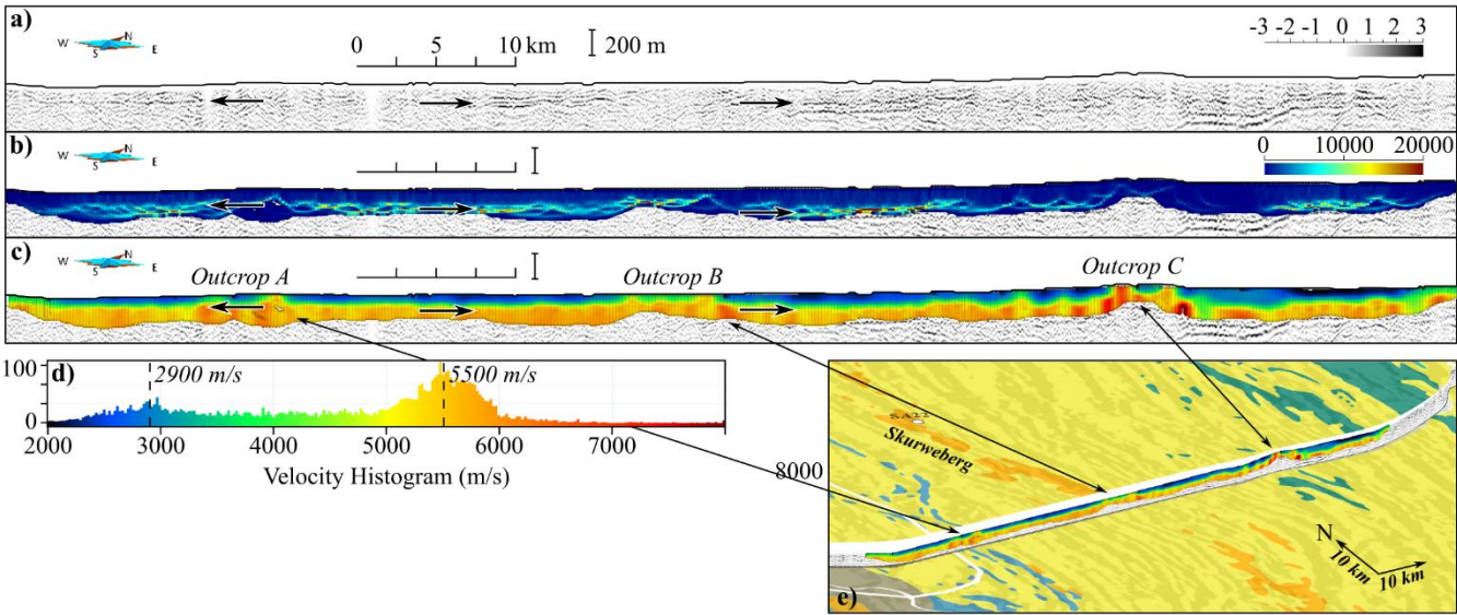
475 Figure 11: Results of the first-break traveltime tomography, showing (a) the reflection section, (b) the computed raypath count, and (c) the velocity field. The colourbar for (c) is plotted as a histogram in (d), and (e) shows the velocity results overlaid on the geology map from Figure 2 to illustrate outcrops. Black arrows delineate a strong lateral velocity contrast that are coincident with regions of reflectivity.
