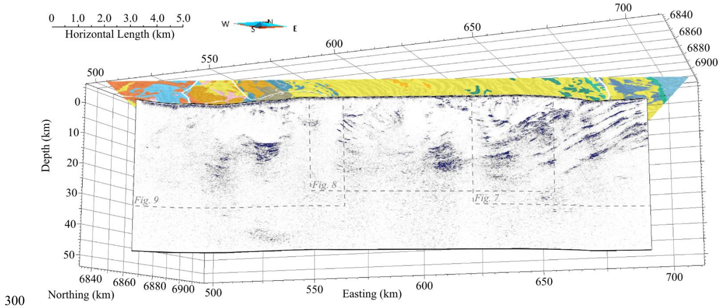
300 Figure 5: The amplitude envelope, or instantaneous amplitude, of the reprocessed GS-02 seismic section plotted in 3D space. Boxes indicate portions of the profile that are enlarged in subsequent images. Plotted on top of the seismic section is the geological map as in Figure 2.
