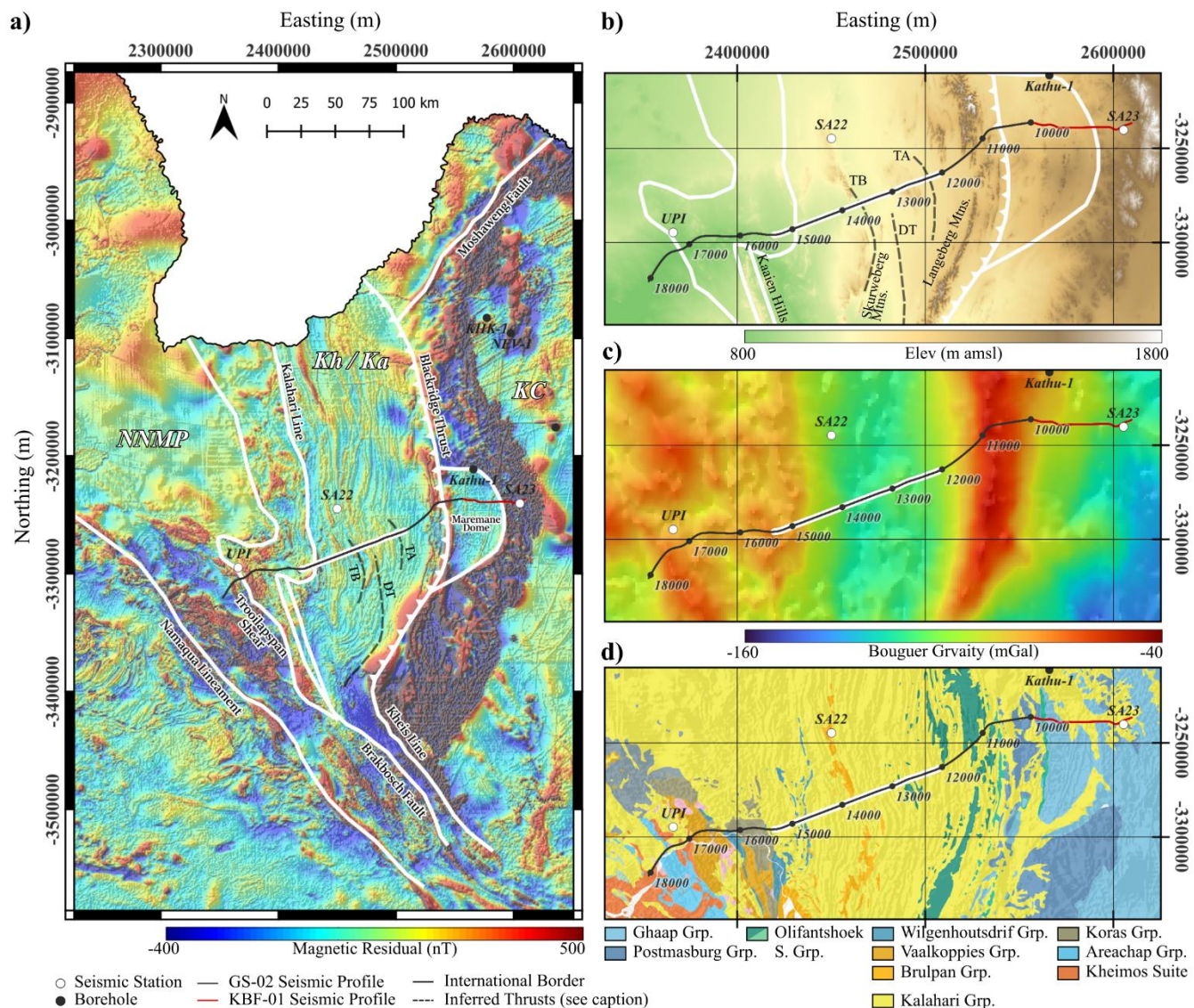
100 Figure 2: Geophysical and geological maps of the study area, including (a) aeromagnetic, (b) elevation, (c) gravity and (d) outcrop geology. Major tectonic boundaries are labeled on the aeromagnetic map. The two profiles used in the study, GS-02 and KBF-01, are plotted in black and red, respectively. The straight portion of the GS-02 profile that is highlighted in white demarcates the extent of the tomography. White circles with labels mark the broadband seismic stations. Inferred thrust traces TA (“Thrust A”; Van 105 Niekerk and Beukes, 2019), TB (“Thrust B”; Van Niekerk and Beukes, 2019), and DT (Dabep Thrust; Moen, 1999) are also plotted. Major terranes are labeled as: NNMP - Namaqua-Natal Metamorphic; Kh/Ka – (Kheis / Kaaien provinces); KC – Kaapvaal Craton. Coordinate reference system used: Web Mercator Projection.
