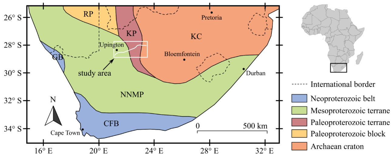
70 Figure 1: Map showing the major tectonic provinces of southern Africa and the location of our study region, along with the seismic profiles overlaid in unicolour white (Figure 2 shows independent profiles). RP Rehoboth Province; KP Kheis Province (here inclusive of the Kaaien Terrane); KC; Kaapvaal Craton; NNMP Namaqua-Natal Metamorphic Province; GB Gariep Belt; CFB Cape Fold Belt.
