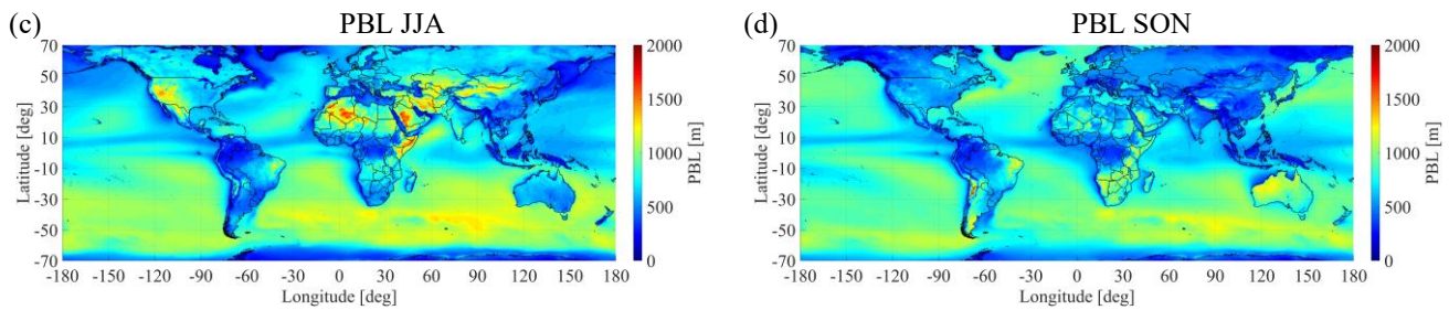
Figure 5: ERA5 mean PBL height (m) above mean surface elevation, seasonally grouped for December–January–February (DJF; Fig.5a), March–April–May (MAM; Fig.5b), June–July–August (JJA; Fig.5c), and September–October–November (SON; Fig.5d) and for the year-period 2006 to 2023.
