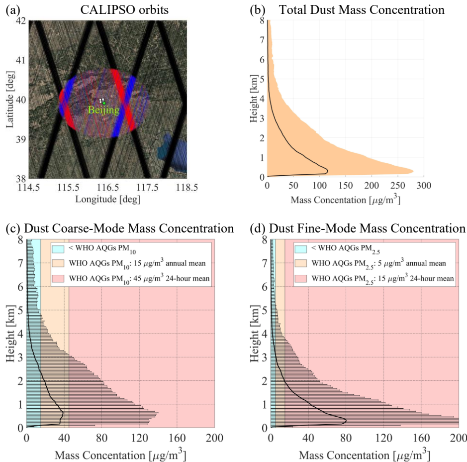
Figure 7: CALIPSO daytime (red lines) and nighttime (blue lines) overpasses within 100 km distance from the Beijing megacity (Fig. 7a), mean mass concentration ( \mu g m^{-3} ) profiles of dust (Fig. 7b), coarse-mode dust (Fig. 7c), and fine-mode dust (Fig. 7d), for the period extending between 06/2006 and 07/2023. The figure provides for the cases of the coarse-mode (Fig. 7c) 450 and fine-mode (Fig. 7d) mean dust mass concentration profiles the corresponding World Health Organization (WHO) air quality guidelines (AQG) for PM_{10} and PM_{2.5} respectively, and for both the cases of 24-hour-mean and annual-mean particulate matter exposure. Layer background: © Google Maps.
