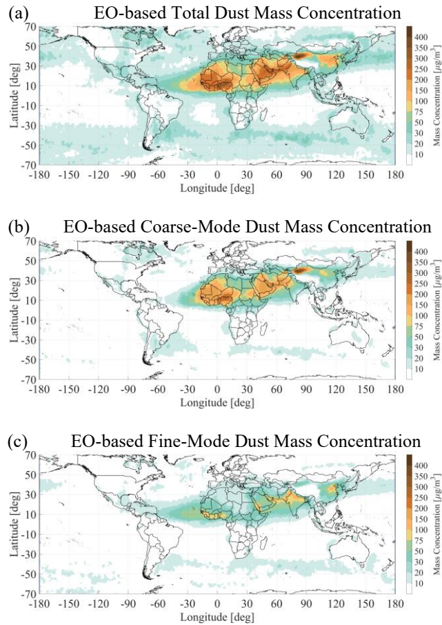
Figure 4: EO-based total (Fig.4a), coarse-mode (Fig.4b), and fine-mode dust (Fig.4c) dust mean mass concentration ( \mu\text{g m}^{-3} ), corresponding to the altitudinal range 0 - 500 m above mean surface elevation, gridded at 1^\circ \times 1^\circ spatial resolution and for the temporal period extending between June 2006 and July 2023.
