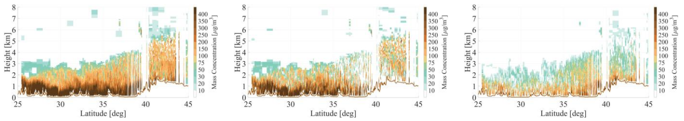
215 Figure 2: Illustration of the established methodology towards extracting the atmospheric dust component from the total aerosol load and accordingly separating the fine-mode and coarse-mode components of atmospheric dust, provided on the basis of an indicative CALIPSO-Beijing nighttime overpass on the 16 th of April 2018-04-16 between 18:29:57 and 18:35:30 UTC (Fig. 2a). On the second row, the quality-assured total backscatter coefficient at 532 nm (Fig.2b), Feature Type (Fig.2c), and Aerosol Subtype (Fig.2d) are provided. The third row provides the final products of total dust (Fig.2e), coarse-mode dust (Fig.2f), and 220 fine-mode dust (Fig.2g) in terms of quality-assured profiles of backscatter coefficient at 532 nm. On the fourth row, the total dust (Fig.2h), coarse-mode dust (Fig.2i), and fine-mode dust (Fig.2j) components of the total aerosol load in terms of quality- assured extinction coefficient at 532 nm profiles are shown. The fifth row provides the total dust (Fig.2k), coarse-mode dust (Fig.2l), and fine-mode dust (Fig.2m) components of the total aerosol load in terms of profiles of mass concentration ( \mu\text{g m}^{-3} ). Layer background: © Google Maps. Layer background: © Google Maps.
