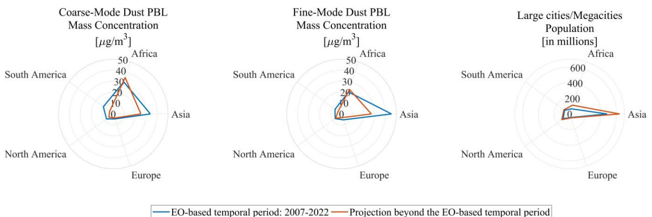
1045 Figure 16: Average continental-scale coarse-mode dust PBL mass concentration (Fig.16-left), fine-mode dust PBL mass concentration (Fig.16-center), and population of the large cities and megacities (Fig.16-right), depicting the long-term EO- based mean conditions (blue line) and for the projection beyond the EO-based temporal period (red line).
