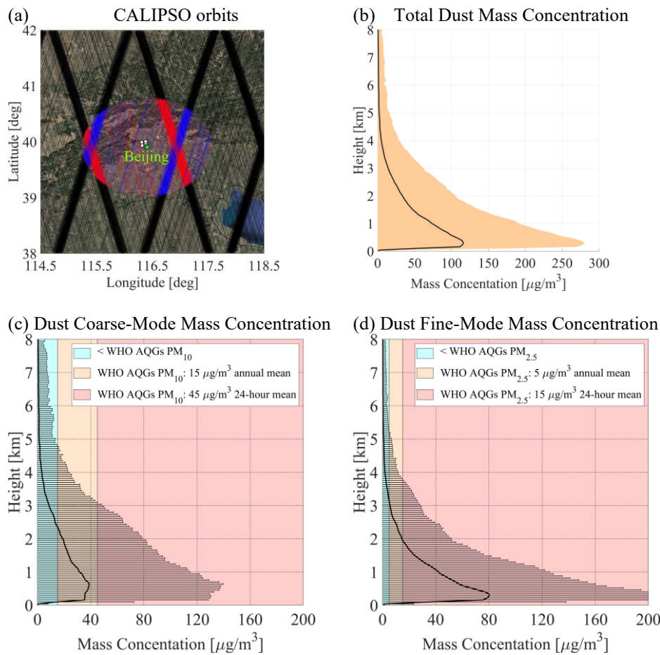
Figure 7: CALIPSO daytime (red lines) and nighttime (blue lines) overpasses within 100 km distance from the Beijing megacity (Fig.7a), mean mass concentration ( \mu\text{g m}^{-3} ) profiles of dust (Fig.7b), coarse-mode dust (Fig.7c), and fine-mode dust (Fig.7d), for the period extending between 06/2006 and 07/2023. The figure provides for the cases of the coarse-mode (Fig.7c) and fine-mode (Fig.7d) mean dust mass concentration profiles the corresponding World Health Organization (WHO) air quality guidelines (AQG) for PM 10 and PM 2.5 respectively, and for both the cases of 24-hour-mean and annual-mean particulate matter exposure. Layer background: © Google Maps.
