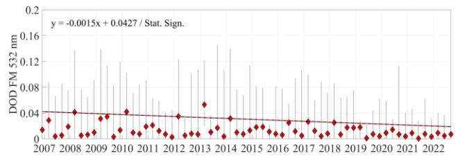
Figure 9: EO-based seasonal-mean PBL coarse-mode DOD at 532 nm (Fig.9a) and fine-mode DOD at 532 nm (Fig.9b) and reported trends, computed on the basis of CALIPSO overpasses within 100 km radius from the Beijing megacity area and for the temporal period extending between DJF/2006 and SON/2022.
