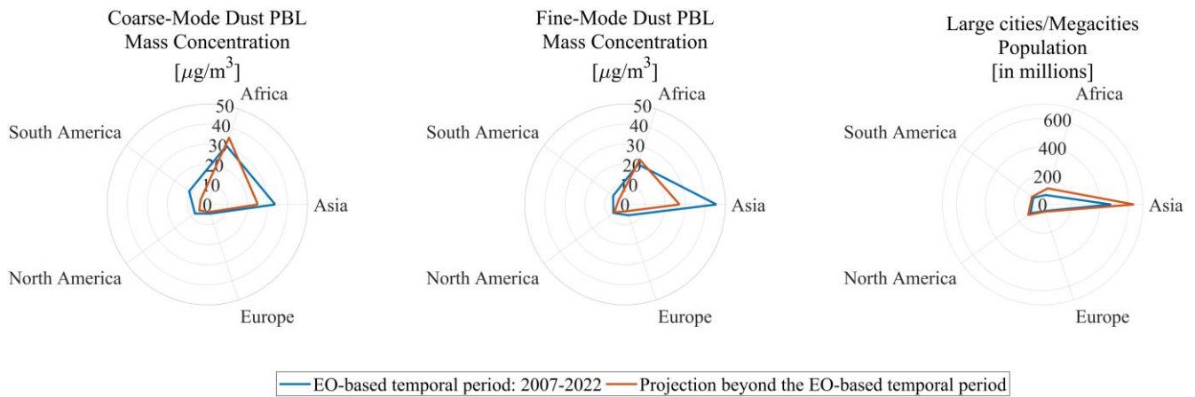
1110 Figure 16: Average continental-scale coarse-mode dust PBL mass concentration (Fig.16-left), fine-mode dust PBL mass concentration (Fig.16-center), and population of the large cities and megacities (Fig.16-right), depicting the long-term EO-based mean conditions (blue line) and for the projection beyond the EO-based temporal period (red line).
