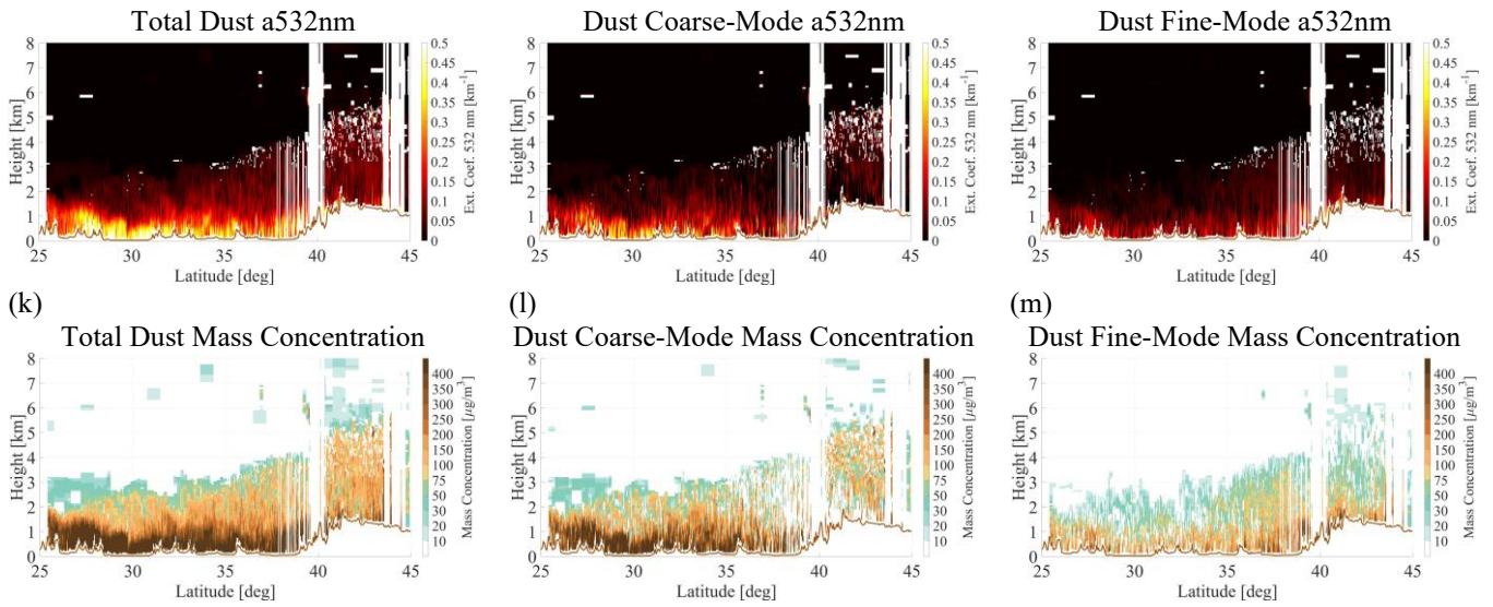
Figure 2: Illustration of the established methodology towards extracting the atmospheric dust component from the total aerosol load and accordingly separating the fine-mode and coarse-mode components of atmospheric dust, provided on the basis of an indicative CALIPSO-Beijing nighttime overpass on the 16 th of April 2018-04-16 between 18:29:57 and 18:35:30 UTC (Fig. 2a). On the second row, the quality-assured total backscatter coefficient at 532 nm (Fig.2b), Feature Type (Fig.2c), and Aerosol Subtype (Fig.2d) are provided. The third row provides the final products of total dust (Fig.2e), coarse-mode dust (Fig.2f), and fine-mode dust (Fig.2g) in terms of quality-assured profiles of backscatter coefficient at 532 nm. On the fourth row, the total dust (Fig.2h), coarse-mode dust (Fig.2i), and fine-mode dust (Fig.2j) components of the total aerosol load in terms of quality-assured extinction coefficient at 532 nm profiles are shown. The fifth row provides the total dust (Fig.2k), coarse-mode dust (Fig.2l), and fine-mode dust (Fig.2m) components of the total aerosol load in terms of profiles of mass concentration ( \mu\text{g}/\text{m}^3 ). Layer background: © Google Maps. Layer background: © Google Maps.
