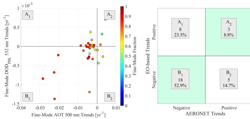
Figure 12: Geographical location of the large cities of the world for which both EO-based temporal trends of fine-mode PBL DOD at 532 nm and AERONET-based temporal trends of fine-mode AOT at 500 nm are calculated (Fig.12-upper panel). Green and red dots denote world-cities with similar and different trend signs, respectively. Scatter plot between EO-based temporal trends of fine-mode PBL DOD at 532 nm and AERONET-based temporal trends of fine-mode AOT at 500 nm (Fig.12-lower left). The color bar indicates the AERONET fine-mode fraction. Confusion matrix of possible trend signs among the two datasets (Fig.12-lower right).
