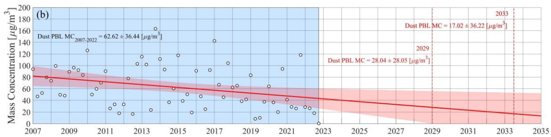
995 Figure 15: Beijing megacity dust coarse-mode (a) and fine-mode (b) mass concentration within the PBL. Cycles in white colour correspond to seasonal mean mass concentration values for the CALIPSO period 2007-2022 (shaded area in light blue). Projection into the temporal period beyond 2022 and up to the year 2035 is shown in terms of linear regression extension and 95% confidence interval for predictions.
