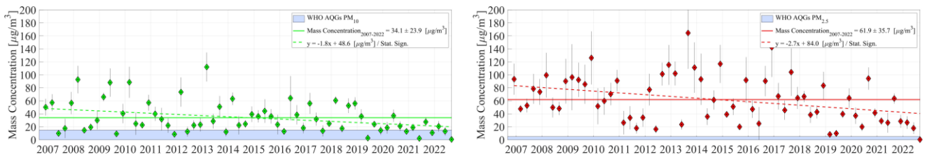
Figure 11: EO-based seasonal-mean PBL coarse-mode dust mass concentration (Fig.11a) and fine-mode dust mass concentration (Fig.11b) and reported trends, computed on the basis of CALIPSO overpasses within 100 km radius from the Beijing megacity area and for the temporal period extending between DJF/2006 and SON/2022. The shaded areas denote the WHO AQG for PM 10 (Fig.1 1a) and PM 2.5 (Fig.1 1b) in terms of annual-mean particulate matter exposure.
