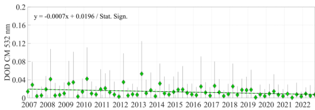
Figure 9: EO-based seasonal-mean PBL coarse-mode DOD at 532 nm (Fig.9a) and fine-mode DOD at 532 nm (Fig.9b) and reported trends, computed on the basis of CALIPSO overpasses within 100 km radius from the Beijing megacity area and for the temporal period extending between DJF/2006 and SON/2022.
