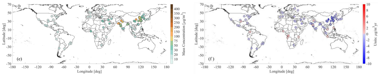
Figure 13: Dust (first row), coarse-mode dust (second row), and fine-mode dust (third row) PBL mass concentration (left column) and PBL mass concentration trends (right column) as established on the basis of CALIPSO overpasses within 100 km radius from each world-city with population greater than 5 million as reported by the United Nations (UN; 2018a, 2019) and on the basis of the temporal period DJF/2006-SON/2022.
