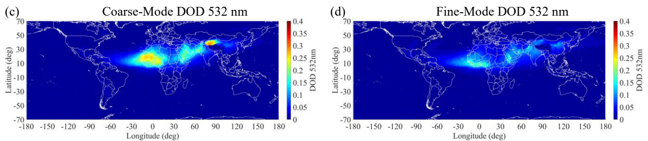
295 Figure 3: CALIOP-based AOD at 532 nm (Fig.3a), ESA-LIVAS DOD at 532 nm (Fig.3b), and coarse-mode DOD at 532 nm (Fig.3c) and fine-mode DOD at 532 nm (Fig.3d), gridded at 1^{\circ} \times 1^{\circ} spatial resolution and for the temporal period extending between June 2006 and July 2023.
