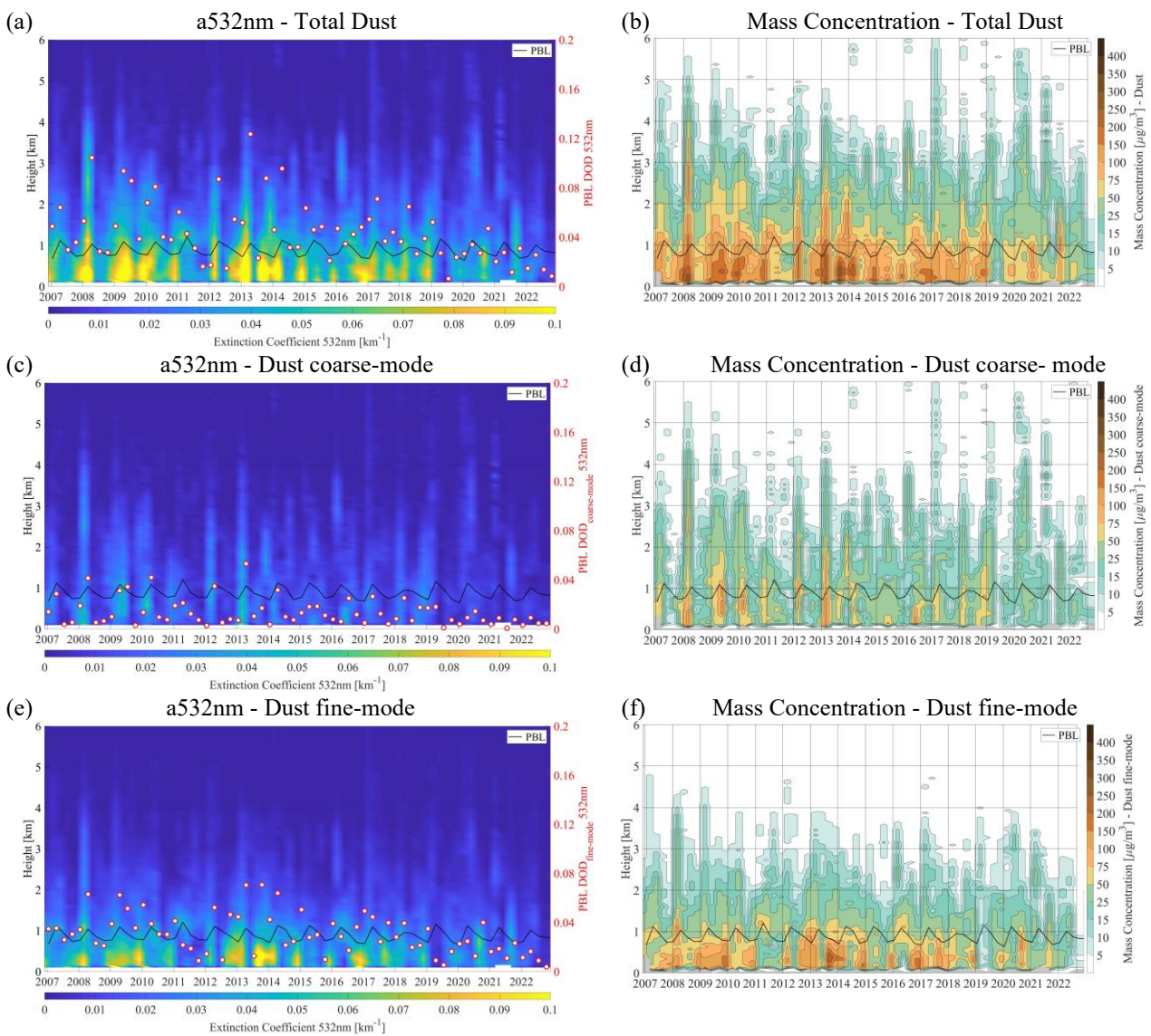
575 Figure 8: Dust (first row), coarse-mode dust (second row), and fine-mode dust (third row) seasonal-mean extinction coefficient at 532 nm profiles (left column) and mass concentration profiles (right column) as established on the basis of CALIPSO overpasses within 100 km radius from the Beijing megacity area and for the temporal period extending between DJF/2006 and
