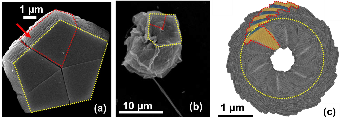
Figure B7: Comparison between the B. bigelowii and the reconstructed N. globulus . (a) SEM image of the pentagonal skeleton of B. bigelowii , adapted from Bown, 2010. The yellow dotted lines mark the boundaries of the pentagonal skeleton and the red dotted lines represent a segment. The red arrow indicates the parallel stacking of the lamellae, forming a segment. (b) The organic substrate, acts as template for the calcification of B. bigelowii . The yellow dotted lines represent the boundary of the substrate that resembles the pentagonal skeleton. The substrate is divided into five parts, with one part marked by the red dotted lines, mimicking the shape of the segment. Image adapted from Hagino et al., 2016. (c) The basal view of the reconstructed skeleton of N. globulus . The yellow dotted circle represents the “probable” organic substrate, acting as template for the calcification of Nannoconus . The substrate is divided into 12 parts (as Nannoconus is considered to have 12 segments), with the boundaries of one part marked by the red dotted lines.
