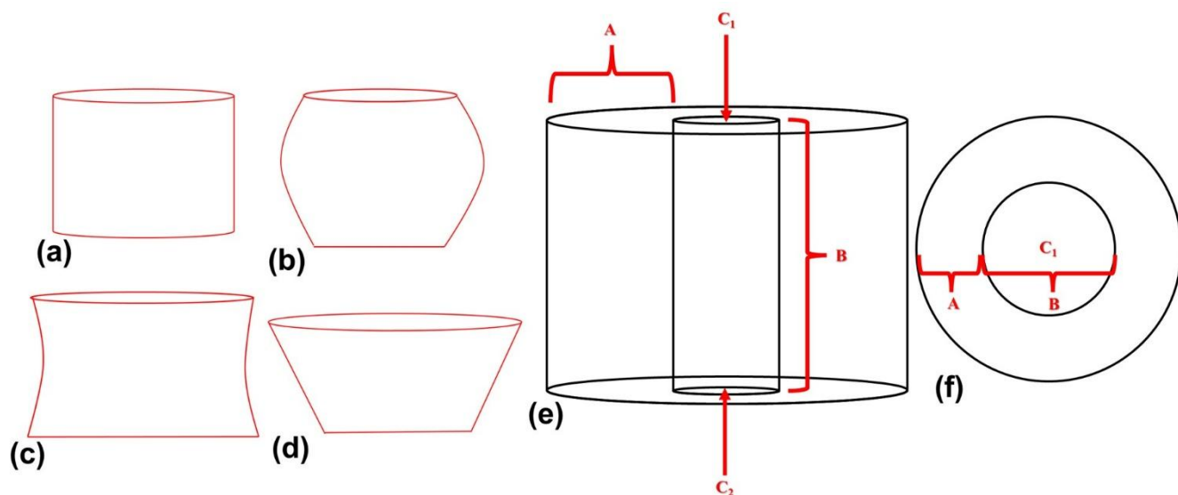
80 Figure 1: Schematic diagrams illustrating four different skeletal morphologies of four different species of Nannoconus . These are (a) cylindrical, (b) globular, (c) hour-glass, and (d) conical as observed in Nannoconus truittii , Nannoconus globulus , Nannoconus abundans , and Nannoconus steinmannii respectively. (e and f) Longitudinal and transverse views, respectively, of the schematic illustration of a cylindrical skeleton. In this figure, A and B represent the wall and the central canal respectively. C 1 and C 2 are the two terminal apertures. It should be noted that the shape of the central canal differs with the general morphology of the skeleton.
