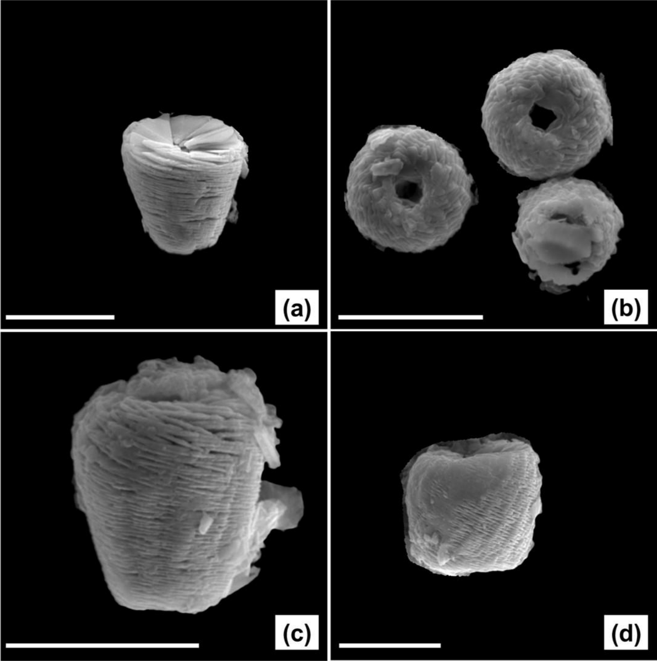
570 Figure B2: SEM images of well-preserved specimens of Nannoconus , from DSDP Leg-93-Site 603 (continental rise of the western margin of the North Atlantic) core 44, interval 115-116 cm. Individual lamella can be clearly distinguished in each of the specimens
