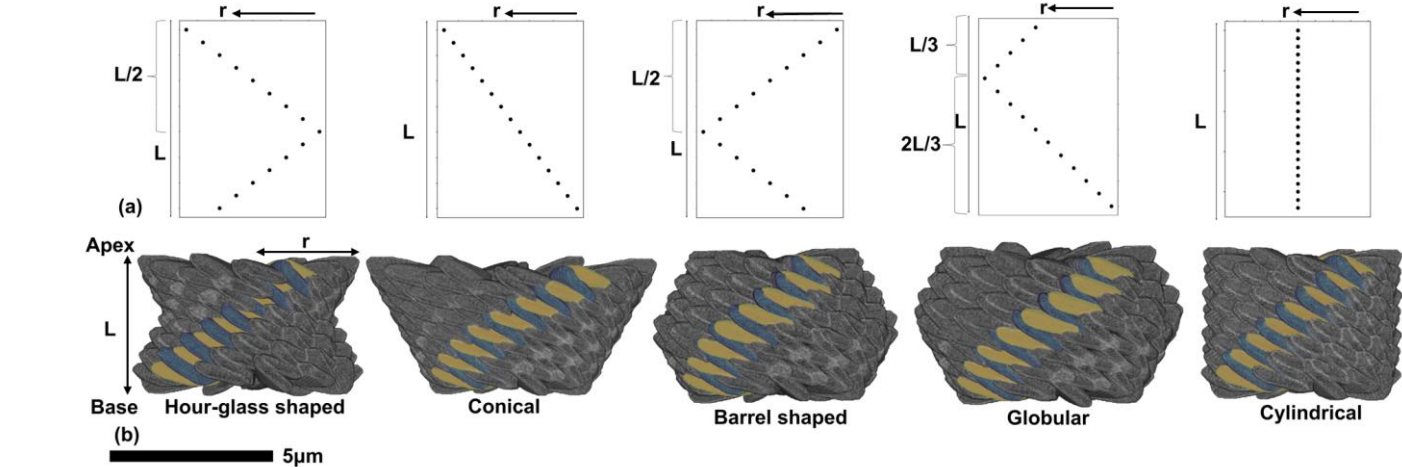
Figure 11: Five different skeletal morphologies of Nannoconus , each with distinct variation of radius ( r ) across the length ( L ). (a) Graphical expressions of five different variations of radius along the length of the reconstructed skeleton, as shown in Table 4. Each of the points on the graphs indicate individual lamella of a segment. (b) Skeletons reconstructed following each of the possibilities, using the segment model, with each skeleton highlighting a segment containing both types of lamellae-A (yellow) and -B (green).
