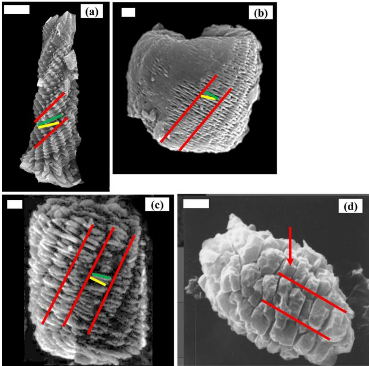
585 Figure B6: SEM images of different species of Nannoconus , with the segments, marked in red lines along with lamella-A (yellow line) and -B (green line). (a) N. funiculus ; adapted from Lees and Bown (2016). (b) N. globulus , from DSDP Leg-93-Site 603 (continental rise of the western margin of the North Atlantic; core 44, interval 115-116 cm) presented in Fig. B2d in this study. (c) 590 N. truitii ; adapted from Hattner and Wise (1980), as available in the Nannotax3 website (Young et al., 2022). (d) N. compressus ; adapted from Bown and Cooper (1998). The red arrows indicate lamellae that have fused and thickened due to overgrowth. The two types of lamellae (i.e., -A and -B) cannot be distinguished separately. This specimen, however, has preserved the organization of the segments. The white bar represents 1 \mu\text{m} .
