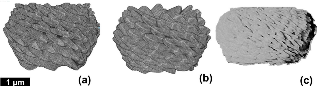
Figure 9: Two different reconstructions of the entire skeleton of N. globulus . (a) reconstruction based on the layer model and (b) reconstruction based on the segment model. Similar skeletal reconstruction is also proposed by Aubry (2025); Fig. 12d. (c) External view of the specimen of N. globulus used in the PXCT experiment (see also Fig. 3b).
