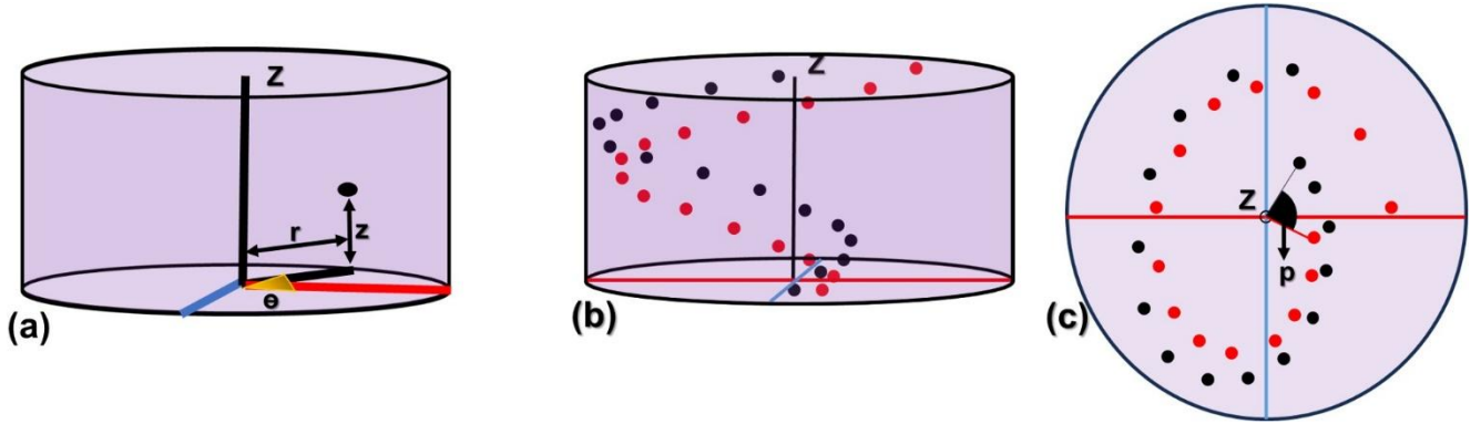
275 Figure 6: Presentation of the series of points in spiral axes to form the layers and segments in the cylindrical coordinate system. (a) Radius ( r ), azimuth ( \theta ), and vertical distance ( z ) that define a point in the cylindrical coordinate system. The red line represents the radial axis, and the blue line represents a line perpendicular to it. (b, c) Longitudinal and transverse views, respectively, of the two series of points defined by the black and red dots in the cylindrical coordinate system, representing two consecutive layers/segments. Here, “ p ” marks the angular separation between the two series of points.
