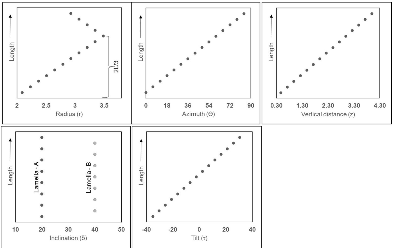
Figure B5: Graphical representation showing the variation of parameters along the length (L) of the first reconstructed segments composed of lamella-A and -B of N. globulus . The black points in the graphs, mark individual lamellae.
