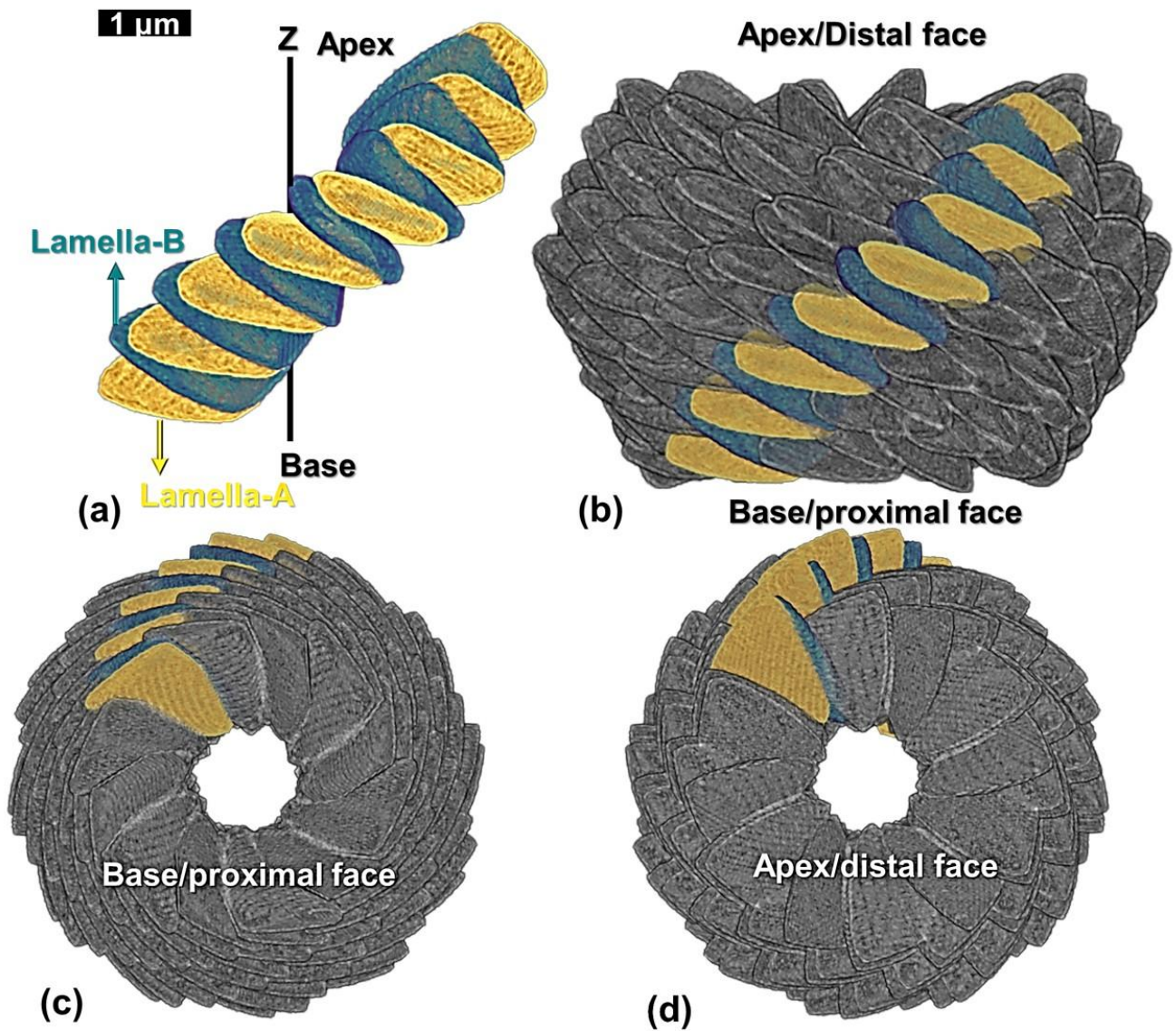
Figure 8: Reconstruction of the skeleton of N. globulus using the segment model. (a) Longitudinal view with alternating, properly oriented, lamella-A (yellow) and -B (green). (b, c, and d) Longitudinal, basal and apical views, respectively, of the combination of 12 such reconstructed segments forming the entire skeleton. A segment containing alternatively placed lamella-A and -B is highlighted. “Proximal” and “distal” (Aubry, 2013) terms refer to the orientation of the skeleton on the cell. Proximal face: face closest to the cell and distal face: face farthest from the cell.
