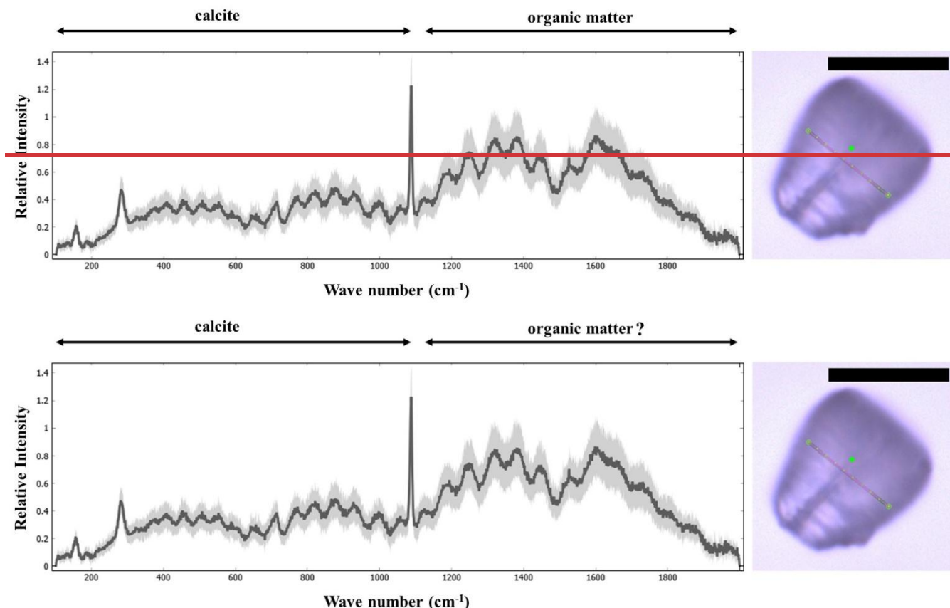
605 Figure B8: Confocal Raman spectra of Nannoconus displaying two regions corresponding to the compositional \text{CaCO}_3 and the “organic matter” preserved within the skeleton. The photomicrograph in optical microscopy (PPL) of the Nannoconus is given on the right, with a red line showing the scanning path for the spectra. The black scale bar represents 10 \mu\text{m} . PPL: plane-polarized light. The Raman spectra were obtained using a LabRAM Soleil Horiba Raman micro spectrometer with 532 nm wavelength laser- excitation and 1 \mu\text{m} spot size. A laser power of 1.1 mW was used to confirm that there is no damage to the specimens induced by the laser. The laser beam was focused on the sample through a hole of 50 \mu\text{m} using an objective at 100X magnification. The specimen was subjected to linear scans along the surface (5–10 \mu\text{m} ) and also inside the specimen (4–5 \mu\text{m} ). A total 25 scans were recorded, each with an acquisition time of 2 seconds. Peaks were fitted in the spectrum using Gaussian functions in Quasar software (Toplak et al., 2017) as a part of the analyses. The spectra have been normalized to the maximum intensity. The black spectrum represents the average of all 25 recorded spectra of the Nannoconus .
