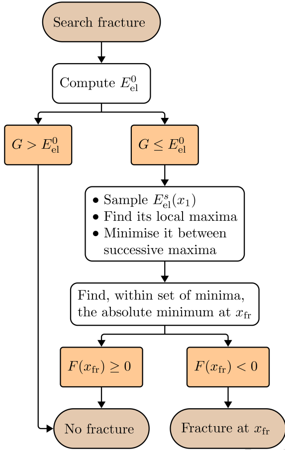
Figure 2. Algorithmic steps behind a fracture search.
