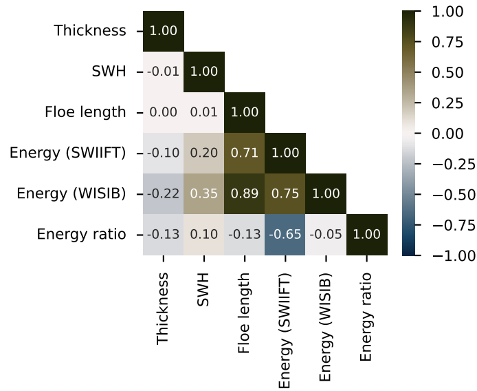
Figure B3. Correlation matrix between input parameters and energy derived from SWIFT and WISIB. We use the Spearman correlation coefficient.
