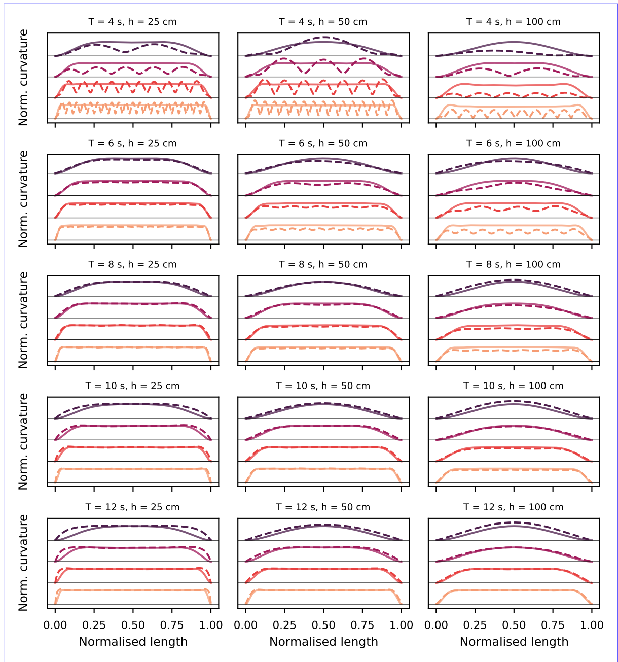
Figure B1. Comparison of curvature envelopes derived from SWIFT or WISIB for different periods of wave forcing (row) and different ice thicknesses (columns). Within each panel, from top to bottom (and darker to lighter hue) are floe lengths of 50 m, 100 m, 200 m and 400 m, and the solid line is the SWIFT solution, while the dashed line is the WISIB solution. The x-axes are normalised with respect to floe lengths, and individual curvatures are normalised with respect to the maximal curvature computed with SWIFT. We display only the positive branch of the envelopes, which are symmetrical with respect to each corresponding y-axis. The origin of these y-axes is shown with a thin horizontal black line.
