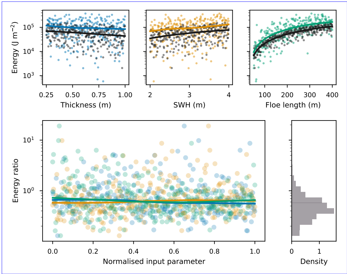
Figure B2. Comparison of potential elastic energy derived from SWIFT or from WISIB. Top row: energy as a function of three parameters, with coloured dots for SWIFT and black dots for WISIB. Lowess regression lines are superimposed. Bottom row: on the left, ratios of energy, as described in the text; the colours correspond to the variables of the top row, which were normalised to fit on the same axis. On the right, distribution of the energy ratio.
