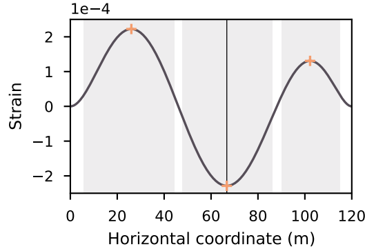
Figure 4. Strain-based fracture parameterisation parametrisation, for a situation corresponding to Fig. 1. The line represents the maximum bending strain along the floe. The shaded vertical strips indicate where the strain exceeds, in absolute value, a typical critical strain of \varepsilon_{cr} = 3 \times 10^{-5} . The crosses indicate local extrema, and the vertical line the global extrema.
