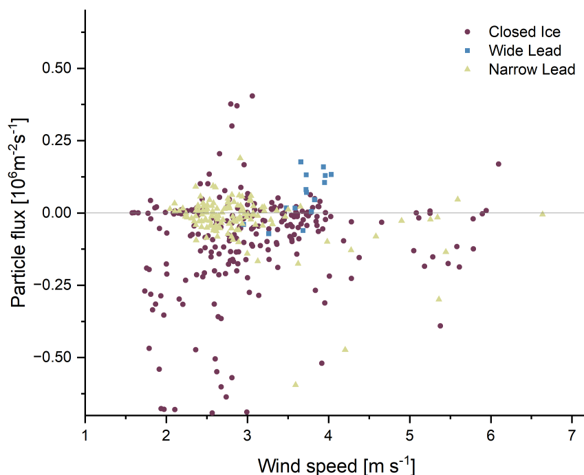
Figure A6. Particle flux [ P , 10^6 \text{m}^{-2} \text{s}^{-1} ] and windspeed [ \text{m s}^{-1} ] at the three surface types closed ice , wide lead and narrow lead for the entire measurement period.
