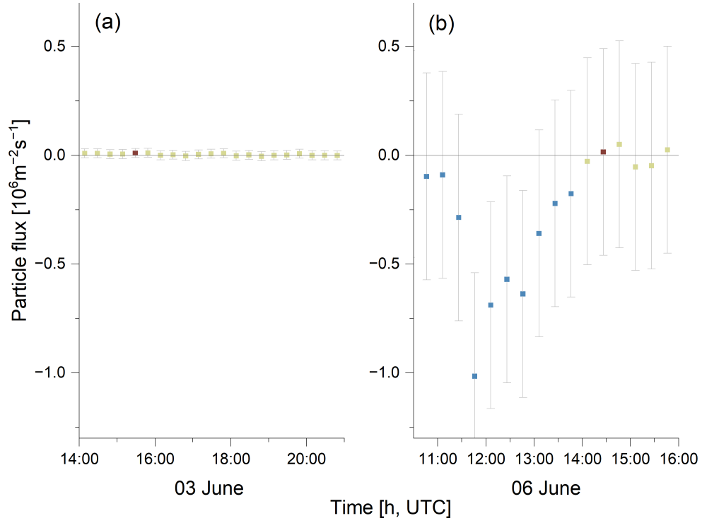
Figure A5. Particle flux [P, 10^6 \text{ m}^{-2} \text{ s}^{-1}] at surface type closed ice on (a) 3 June and (b) 6 June 2023. The brown color indicates net particle emission intervals, and the blue color indicates net particle deposition intervals. The beige color indicates intervals, where u^* < 0.15 \text{ m s}^{-1} . The grey-shaded bars illustrate the maximum error value for the day of measurement, as estimated by Monte Carlo simulations.
