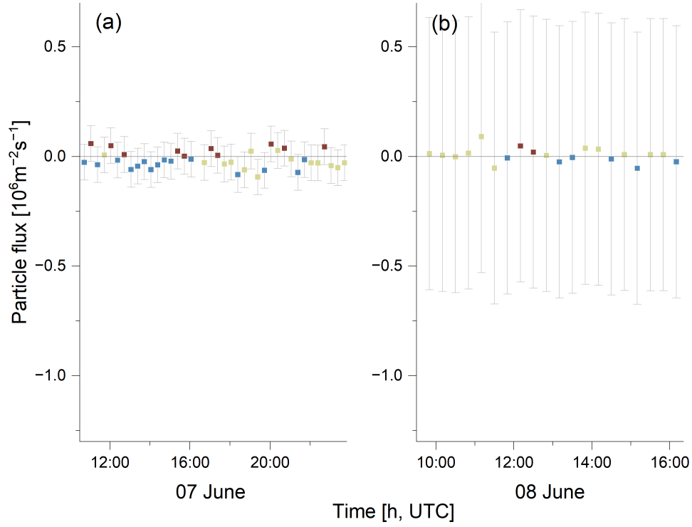
Figure A4. Particle flux [P, 10^6 \text{ m}^{-2} \text{ s}^{-1}] at surface type narrow lead on (a) 7 June and (b) 8 June 2023. The brown color indicates net particle emission intervals, and the blue color indicates net particle deposition intervals. The beige color indicates intervals, where u^* < 0.15 \text{ m s}^{-1} . The grey-shaded bars illustrate the maximum error value for the day of measurement, as estimated by Monte Carlo simulations.
