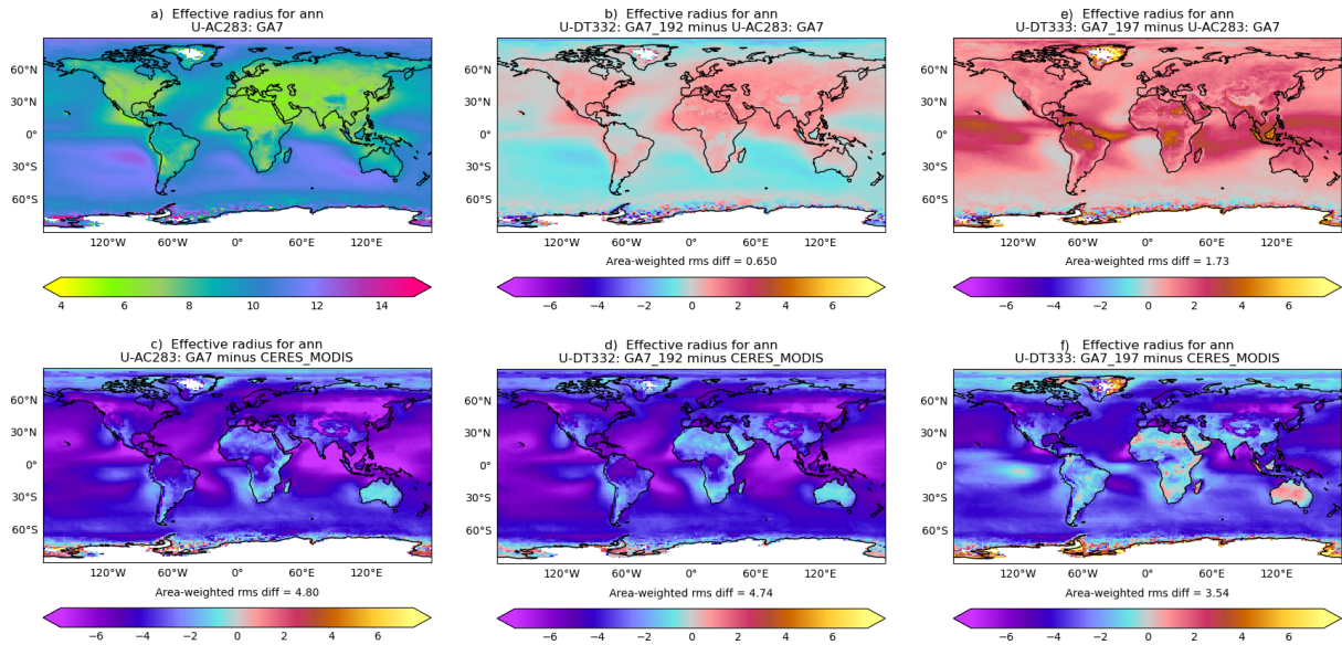
Figure 2. Annual mean cloud droplet effective radius (μm) in the 20 year N96 atmosphere/land only climate simulations compared to Clouds and Earth’s Radiant Energy System (CERES) Moderate Resolution Imaging Spectrometer (MODIS) showing (a) GA7GL7, (b) the effect of the Liu parametrisation (Sect. 3.2.1), (c) the effect of the improved Turbulent Kinetic Energy (TKE) diagnostic (Sect. 3.4.4), (d) the difference between GA7GL7 and MODIS, (e) the difference between GA7GL7 with the Liu parametrisation and MODIS, and (f) the difference between GA7GL7 with the improved TKE diagnostic and MODIS.
