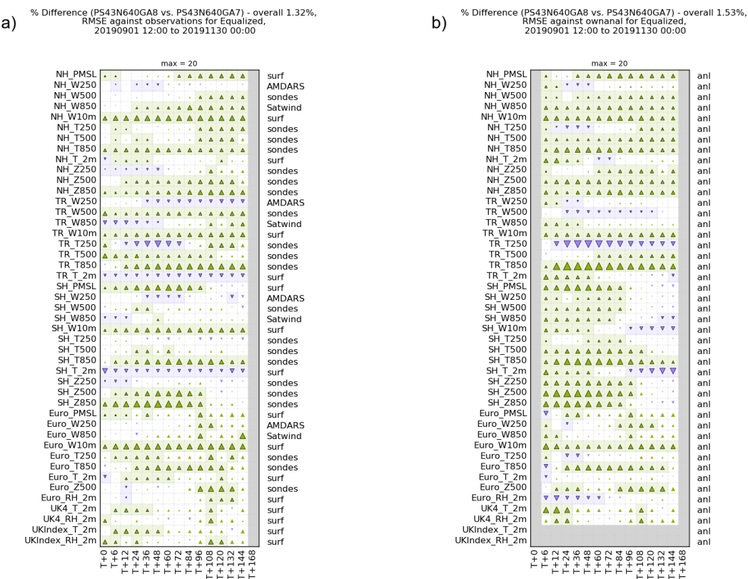
Figure 14. Global evaluation suite scorecards for GA8GL9 vs GA7GL7 for a three month N640 DA non-hybrid trial for September, October and November 2019 with respect to (a) observations and (b) own analysis. Shaded boxes are statistically significant. Green upward pointing triangles indicate the RMSEs in GA8GL9 are reduced relative to GA7GL7, and downward pointing purple triangles indicate where the RMSEs are increased. The area of the triangles is proportional to the change in RMSE with a change of 5 % filling the box.
