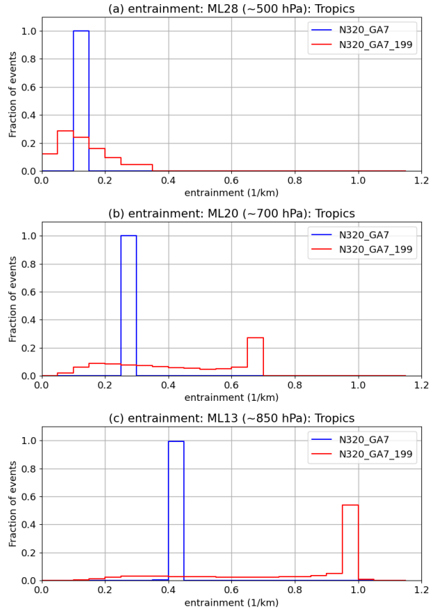
Figure 5. Histogram of entrainment rate for deep convection ( \text{km}^{-1} ) in the tropics ( 20^\circ \text{S} to 20^\circ \text{N} ) at model levels (a) 28 ( \sim 5.6 \text{ km}/500 \text{ hPa} ), (b) 20 ( \sim 2.9 \text{ km}/700 \text{ hPa} ) and (c) 13 ( \sim 1.3 \text{ km}/850 \text{ hPa} ) for GA7GL7 and GA7GL7 with ProgEnt from a 5 day N320 case study. The entrainment rate was sampled hourly. To facilitate the production of the entrainment diagnostic, only a single convective substep was used in the model runs.
