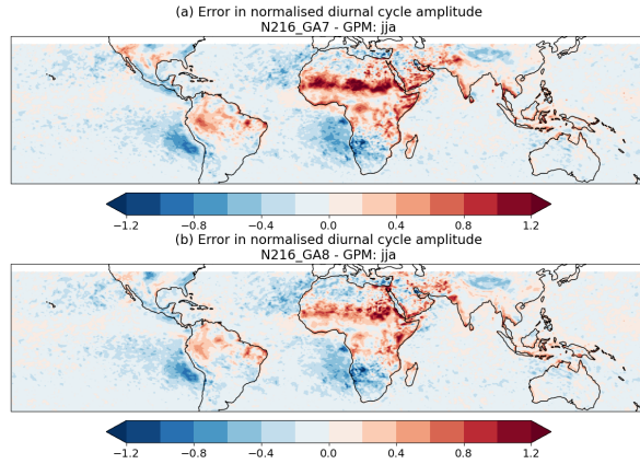
Figure 6. Error in normalised amplitude of the seasonal mean diurnal cycle for a) GA7GL7 and b) GA8GL9 relative to GPM for JJA. The season mean diurnal cycles from the model configurations are aggregated using 20 years of 3-hourly instantaneous precipitation rates. The seasonal mean diurnal cycle for GPM IMERG (Huffman et al., 2020a, b) was aggregated from 10 years of 3-hourly instantaneous precipitation rates and regridded to the model grid using area-averaged weighting. The normalised amplitude is calculated by dividing the standard deviation of the mean diurnal cycle by its mean (i.e. the coefficient of variation of the seasonal mean diurnal cycle).
