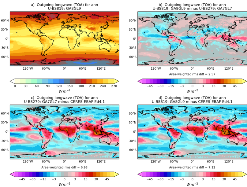
Figure 9. Annual mean top-of-atmosphere outgoing LW radiation ( \text{Wm}^{-2} ) in the 27 year N216 atmosphere/land only climate simulations compared to Clouds and Earth’s Radiant Energy System (CERES) Energy Balanced and Filled (EBAF)dataset version 4.1 (NASA/LARC/S-D/ASDC, 2019) showing (a) GA8GL9, (b) the difference between GA8GL9 and GA7GL7, (c) bias in GA7GL7 relative to CERES-EBAF and (d) bias in GA8GL9 relative to CERES-EBAF.
