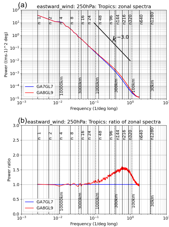
Figure 18. Zonal power spectra of tropical 250 hPa winds from GA8GL9 and GA7GL7 from 0Z and 12Z forecasts during November from the N640 DA trial showing (a) the absolute spectra and (b) the ratio relative to the GA7GL7 spectra.
