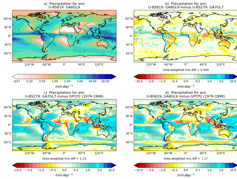
Figure 12. Annual mean precipitation ( \text{mm day}^{-1} ) in the 27 year N216 atmosphere/land only climate simulations compared to GPCP (Adler et al., 2003). Layout is the same as in Fig. 9.
