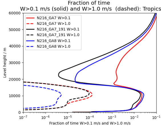
Figure 4. Vertical profile showing the fraction of the time where the vertical velocity exceeds 0.1 \text{ ms}^{-1} in solid and 1.0 \text{ ms}^{-1} in dashed from 20 year N216 atmosphere/land only climate simulations using GA7GL7 , GA7+191 and GA8GL9 for 20^\circ \text{ S} to 20^\circ \text{ N} .
