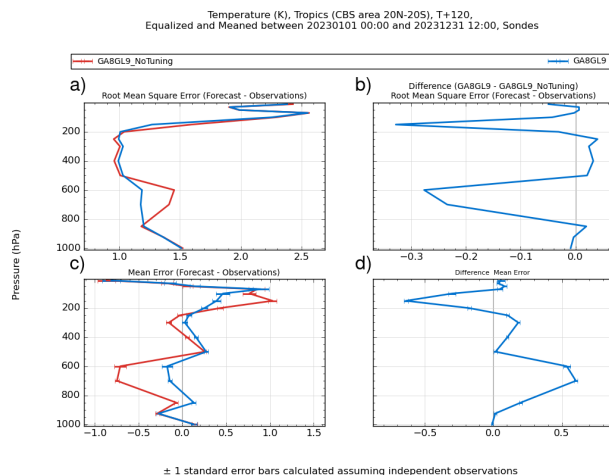
Figure 7. Verification with respect to sondes of tropical T+120 temperatures forecasts from N320 GA8 without tunings and standard GA8 showing a) RMSE, b) difference in RMSE, c) mean error, and d) difference in mean error for 59 cases between January and December 2023.
