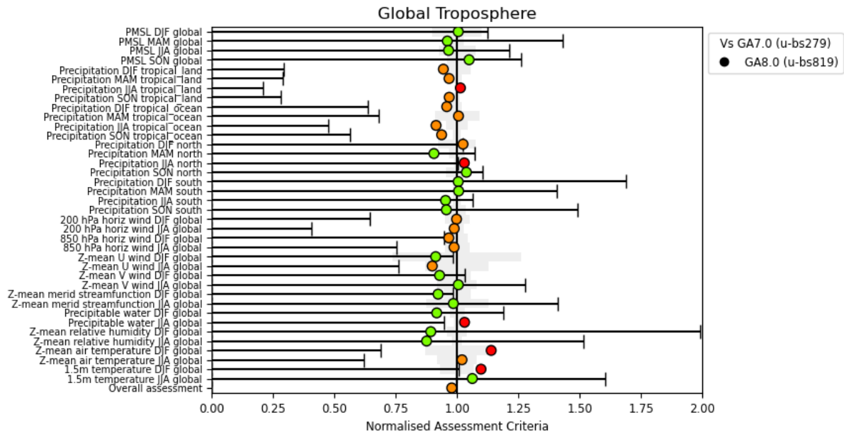
Figure 8. Normalised assessment plot (ratio of mean field RMSEs) for a number of atmospheric fields from a GA8GL9 atmosphere/land-only climate simulation at N216 horizontal resolution compared to an equivalent simulation using GA7GL7. Statistics shown are for seasons December–February (DJF), March–May (MAM), June–August (JJA) and September–November (SON) and for regions global, tropical land (land points between 30° N and 30° S), tropical ocean (sea points between 30° N and 30° S), north (30°–90° N) and south (30°–90° S). The observation datasets used are HadSLP2 pressure at mean sea level (Allan and Ansell, 2006), GPCP precipitation (Adler et al., 2003), SSMI precipitable water (Wentz and Spencer, 1998) and CRUTEM3 1.5 m temperature (Brohan et al., 2006), whilst the remaining climatologies are from ERA-interim reanalyses (Berrisford et al., 2009). The whisker bars are observational uncertainty, which is calculated by comparing these with alternative datasets; these are ERA-40 pressure at mean sea level and precipitable water (Uppala et al., 2005), CMAP precipitation (Xie and Arkin, 1997), Legates and Willmott (1990) 1.5 m temperature and MERRA reanalyses for everything else (Bosilovich, 2008). Green circles denote fields for which the RMSE lies within observational uncertainty, whilst light orange or red circles denote fields that do not, and for which the RMSE is improved or degraded respectively.
