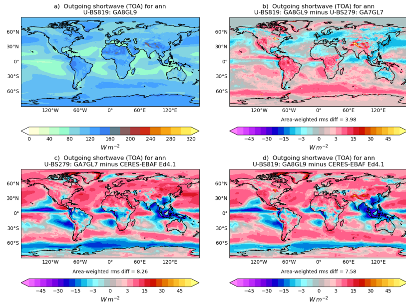
Figure 11. Annual mean top-of-atmosphere outgoing SW radiation ( \text{Wm}^{-2} ) in the 27 year N216 atmosphere/land only climate simulations compared to Clouds and Earth’s Radiant Energy System (CERES) Energy Balanced and Filled (EBAF) dataset version 4.1 (NASA/LARC/SD/ASDC, 2019). Layout is the same as in Fig. 9.
