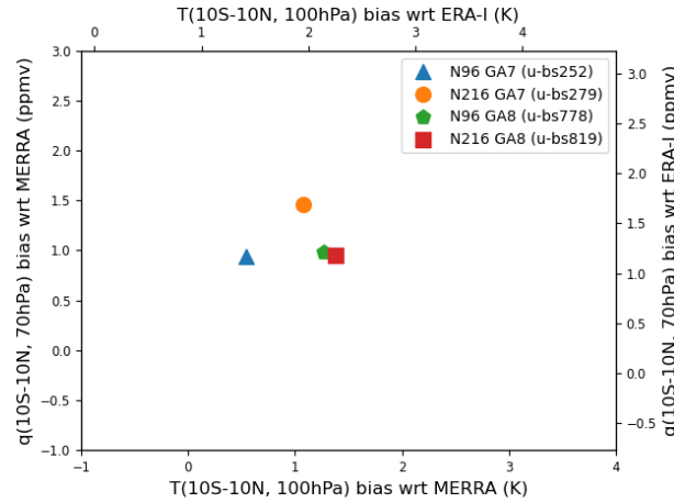
Figure 13. Tropical tropopause layer temperature biases and lower stratospheric humidity biases from 27 year N96 and N216 atmosphere/land-only climate simulations of GA7L7 and GA8L9 with respect to MERRA and ERA-Interim reanalyses (following Hardiman et al. (2015))
