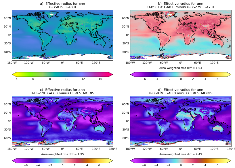
Figure 10. Annual mean cloud droplet effective radius ( \mu\text{m} ) in the 27 year N216 atmosphere/land only climate simulations compared to Clouds and Earth's Radiant Energy System (CERES) Moderate Resolution Imaging Spectrometer (MODIS) Edition 2.6. Layout is the same as in Fig. 9.
