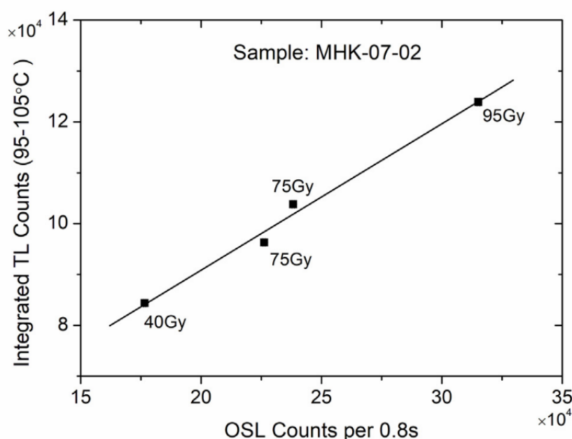
Fig. 1. Figure shows the correlation of TL and OSL signals from a single grain.
