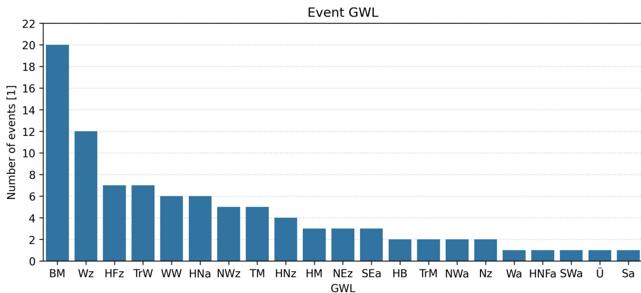
Figure R3: Number of Großwetterlagen (GWL) connected to the HPEs investigated in the study.
