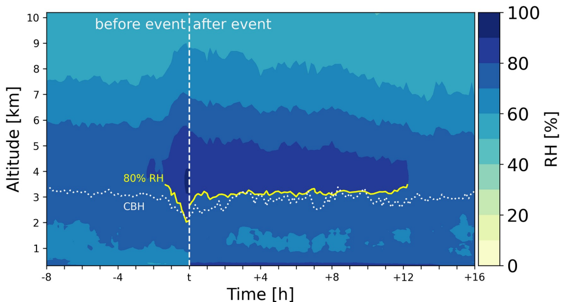
Figure R3: Median vertical structure of relative humidity for WEGN3D (as shown in panel b of Figure 4 in the main paper). The yellow line indicates the 80% RH contour line, the dotted white line marks the CBH.
