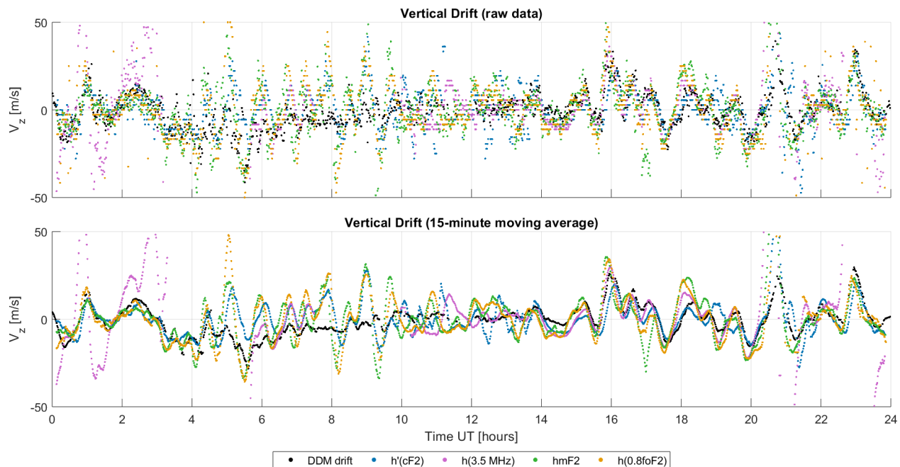
485 Figure 5: Comparison of vertical drifts obtained for Campaign I using various methods with a 15-minute measurement interval: DDM - black, green light-blue - hmF2, blue red - h'F2, purple violet - h'(3.5 MHz), orange green - h'(0.8foF2). No smoothing is applied in the upper panel, while a 15-minute smoothing window is used in the lower panel.
