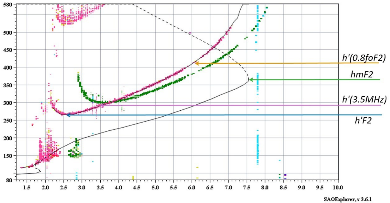
Figure 1: In the ionogram recorded in Pruhonice on March 17, 2017, and on the corresponding electron concentration profile, the parameters peak height F2-layer (hmF2), minimum virtual height of F2 trace (h'F2), virtual height of plasma with plasma frequency 3.5 MHz h'(3.5MHz), and virtual height of plasma with 80 % of critical frequency foF2 (h'(0.8*foF2)) are depicted.
