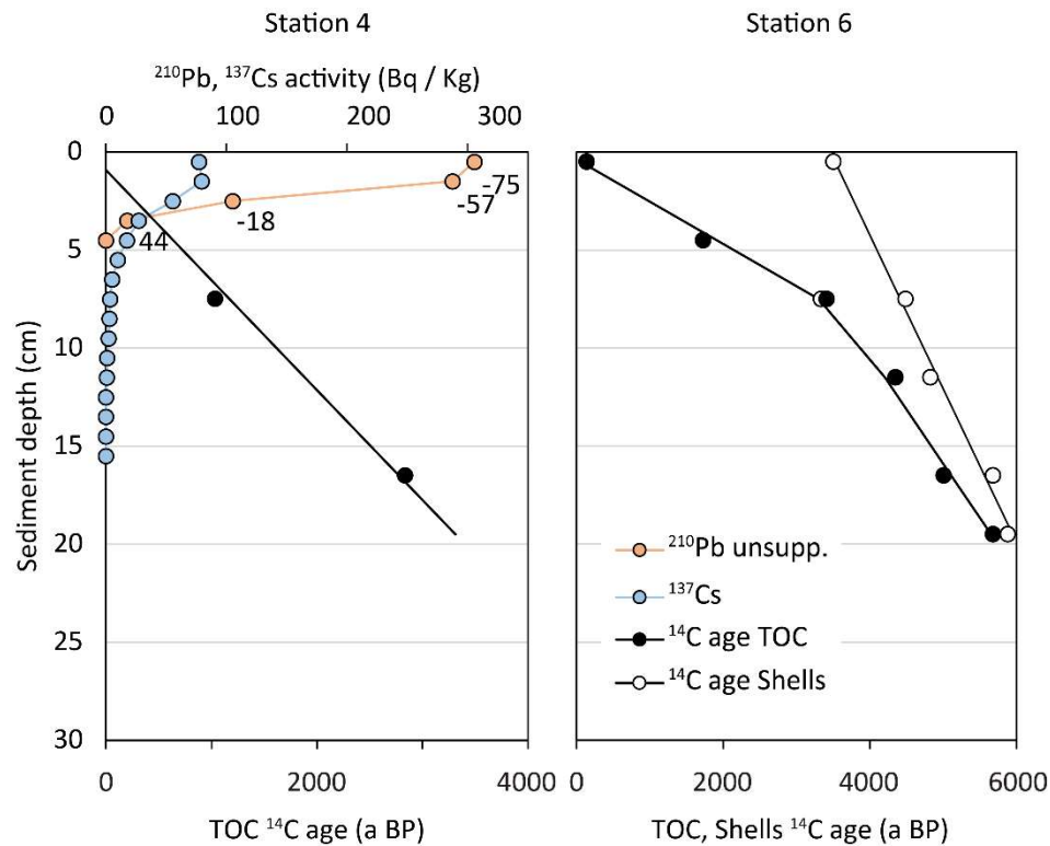
210 Figure 2: Results of radioisotope analyses of cores 4 and 6: Radiocarbon ( ^{14}\text{C} ) ages of organic sediment (black circles), radiocarbon ages of carbonate shells (white circles). Measurements of unsupported ^{210}\text{Pb} (orange circles) and ^{137}\text{Cs} (blue circles). Numbers along ^{210}\text{Pb} plot indicate sediment age according to CRS model. No ^{210}\text{Pb} or ^{137}\text{Cs} data are available for core 6.
