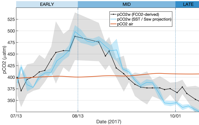
450 Figure 9. Summer 3-day average time series of p\text{CO}_{2\text{w}} derived from F_{\text{CO}_2} using Eq. (1) (black line) and p\text{CO}_{2\text{w}} projection calculated using temperature and salinity relationships (Takahashi et al., 1993; Sarmiento and Gruber, 2006; blue line). Shaded regions represent standard deviation.
