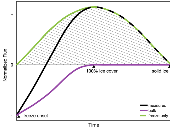
515 Figure 10. Theoretical diagram representing the competing downward air-sea fluxes with upward freeze-related component of the flux during marginal sea ice conditions. The seasonal freeze-only component of the flux can be calculated by integrating the area under its curve (hatched area). The designation of “solid ice” refers to the moment during winter when low sea ice temperatures render the ice matrix impermeable (Gosink et al., 1976).
