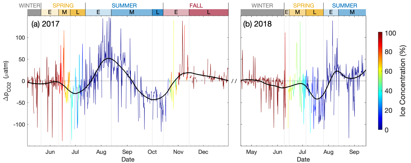
330 Figure 7. Time series of \Delta p\text{CO}_2 (i.e., p\text{CO}_{2w} - p\text{CO}_{2\text{air}} ) estimated using Eqs. 1 and 2. Color of the line represents ice concentration. The black curve represents a locally-weighted least-squares regression line fit with a quadratic polynomial.
