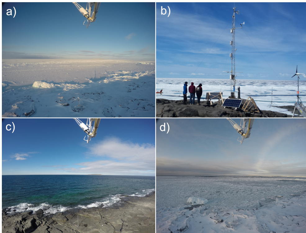
130 Figure 2. Photographs showing the seasonal sea surface conditions in front of the flux tower where (a) shows full ice coverage on 5 Nov 2017 (b) shows melt ponds on 23 June 2017, (c) shows open water on 6 Aug 2017, and (d) shows freezing on 22 Oct 2017. Images a, c, and d taken using GOPRO Hero4 camera mounted at the top of the tower. Image b taken with handheld camera.
