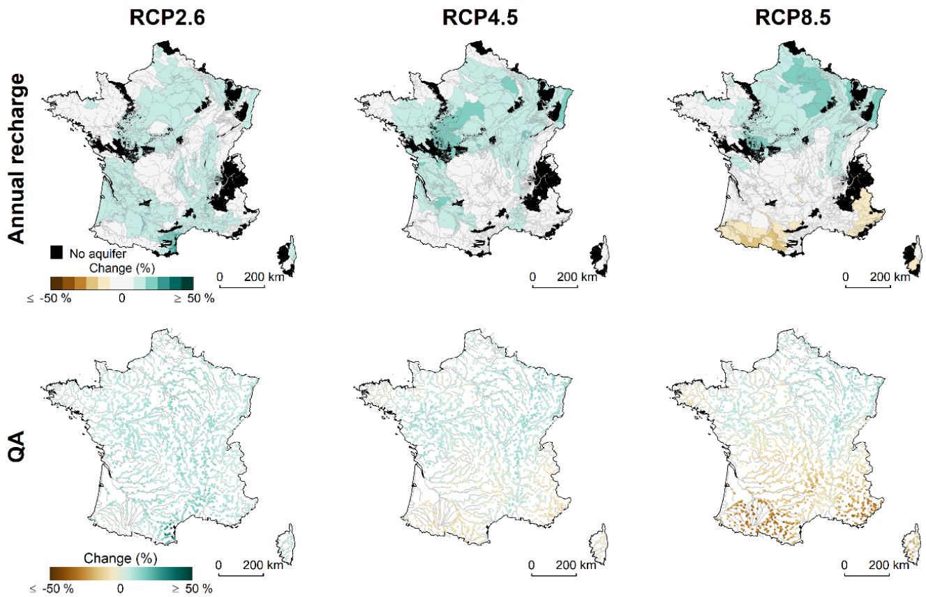
445 Figure 6: Median changes in the annual groundwater recharge and the annual flow QA between the reference period and the end of the century for the three RCPs. The areas coloured black on the maps are those where there is no aquifer and where the notion of groundwater recharge is not relevant.
