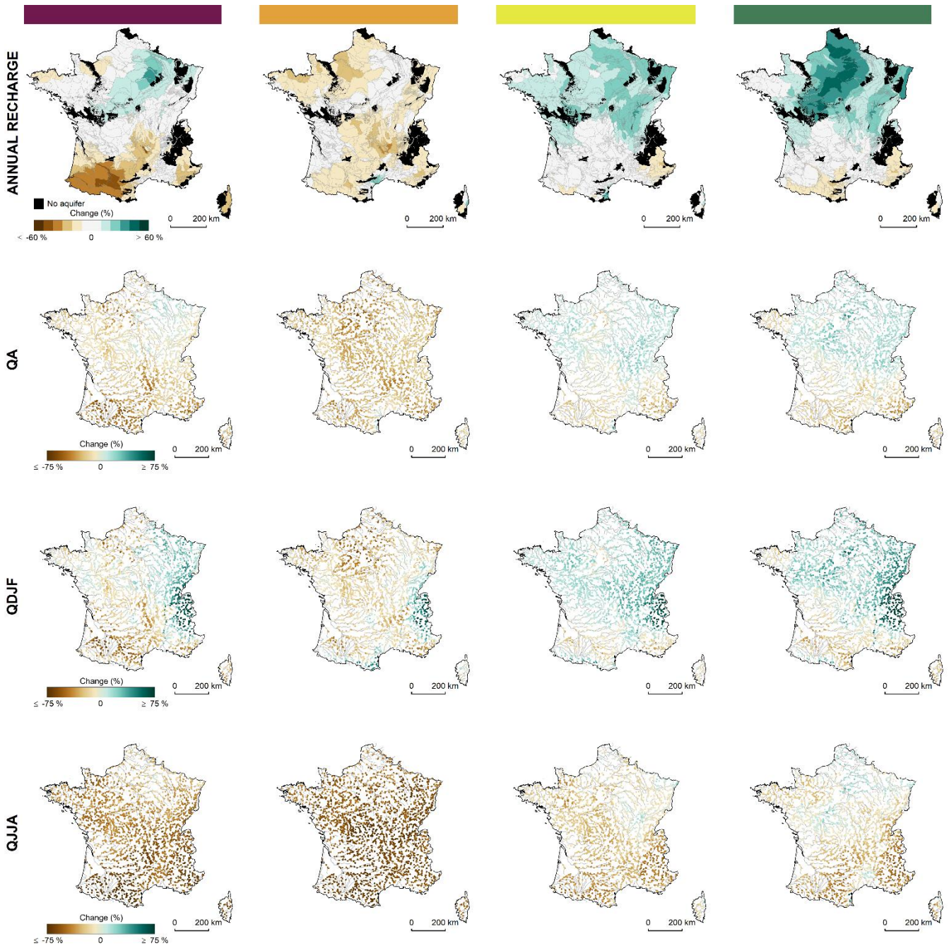
555 Figure 9: Changes in the annual groundwater recharge and the annual, winter and summer flows between the reference period and the end of the century for the four storylines. The areas coloured black on the maps are those where there is no aquifer and where the notion of groundwater recharge is not relevant. Median changes are shown for annual and seasonal flows based on available HMs (please note the different scales in Fig. 7).
