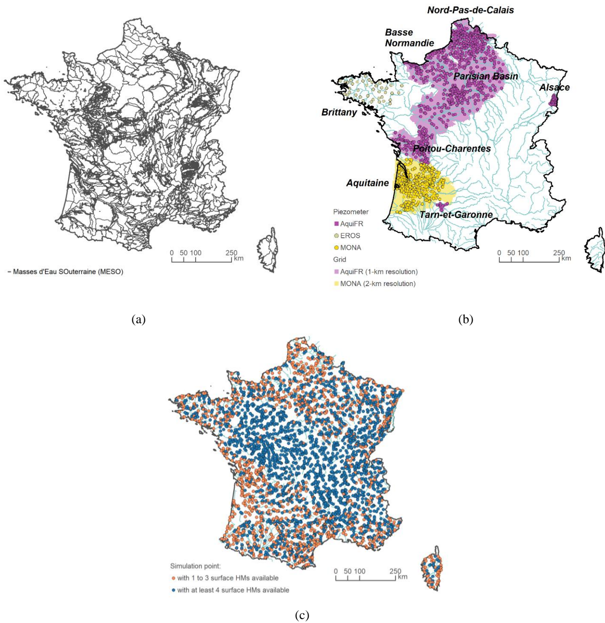
Figure 2: Partition of water bodies (MESO) used for groundwater recharge of groundwater (a), and sets of simulation grid cells and points where water level (b) and streamflow (c) data are simulated.
