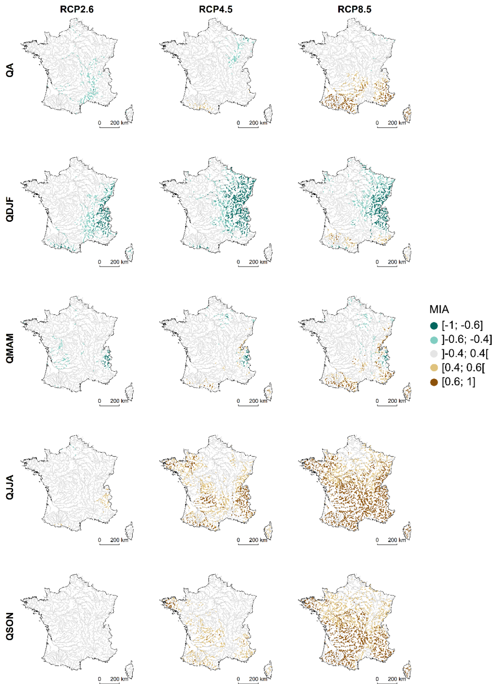
Figure 8: Agreement in median change in the annual flow QA and the seasonal flows QDJF, QMAM, QJJA, and QSON for the three RCPs.
