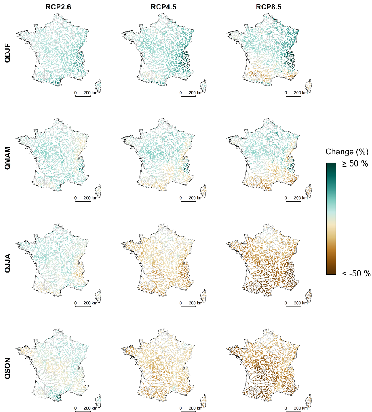
450 Figure 7: Median changes in the seasonal flows QDJF, QMAM, QJJA, and QSON between the reference period and the end of the century for the three RCPs.
