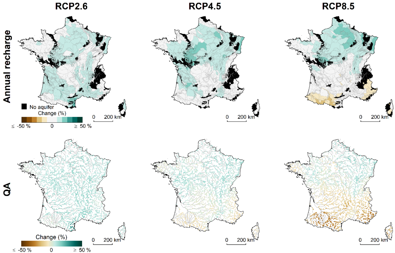
595 Figure 6: Median changes in the annual groundwater recharge and the annual flow QA between the benchmarkreference period and the end of the century for the three RCPs. The areas coloured black on the maps are those where there is no aquifer and where the notion of groundwater -recharge is not relevant.
