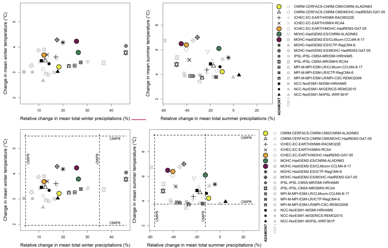
Figure 1: Changes in seasonal precipitation and temperature (winter and summer) between the benchmark reference period 1976-2005 and the end of the century 2070-2099 under RCP8.5. Dots in grey are related to projections obtained with the CDF-t bias correction method while dots in black are related to those obtained with the other bias correction method ADAMONT. Dotted lines define the range of values consistent with projected changes in CMIP6 (calculations were made in 2022).
