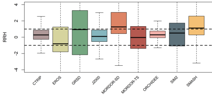
(e) q_{10} ADAMONT
