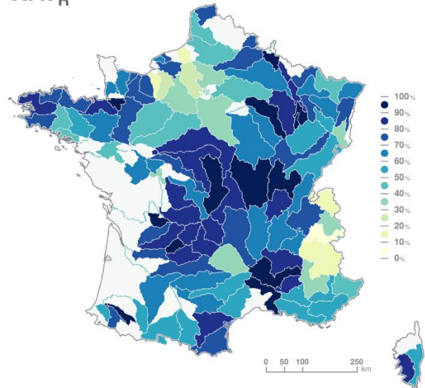
Figure 3: Proportion (%) of simulations with evaluation metrics within the acceptable range. A value of 100 % means that all HMs demonstrate numerical metrics within the acceptable range at all reference gauging stations while a null value means that all HMs demonstrate numerical metrics outside the acceptable range at all reference gauging stations. Statistics of the evaluation metrics have been computed on a division of France into 187 sub-basins ( https://www.sandre.eaufrance.fr ) to identify contrasts in HM performance over the 611 reference gauging stations.
