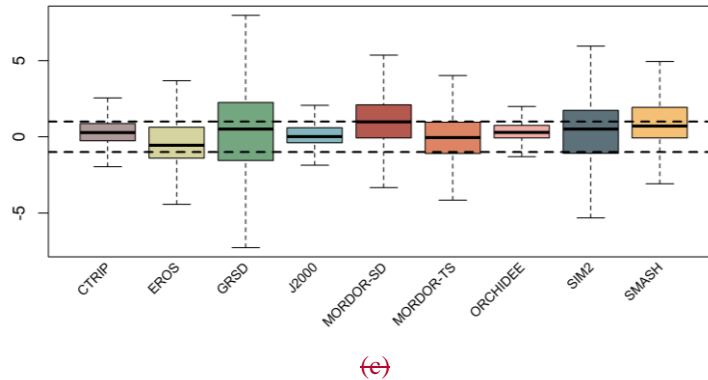
505 Figure 5: Boxplots of the RRH criterion computed for the flow quantile q90 that is exceeded 90 % of the time (a, b), the mean annual streamflow qa (c, d), and the flow quantile q10 (e, f) that is exceeded 10 % of the time (e) for both bias correction methods ADAMONT and CDF-t. The bottom and top of the box are the 25 th and 75 th percentiles, and the line is always the median. The dashed lines represent the values 1 and -1. The boxes have been ordered from left to right in alphabetical order by model name.
