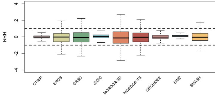
(a) q_{90} ADAMONT
