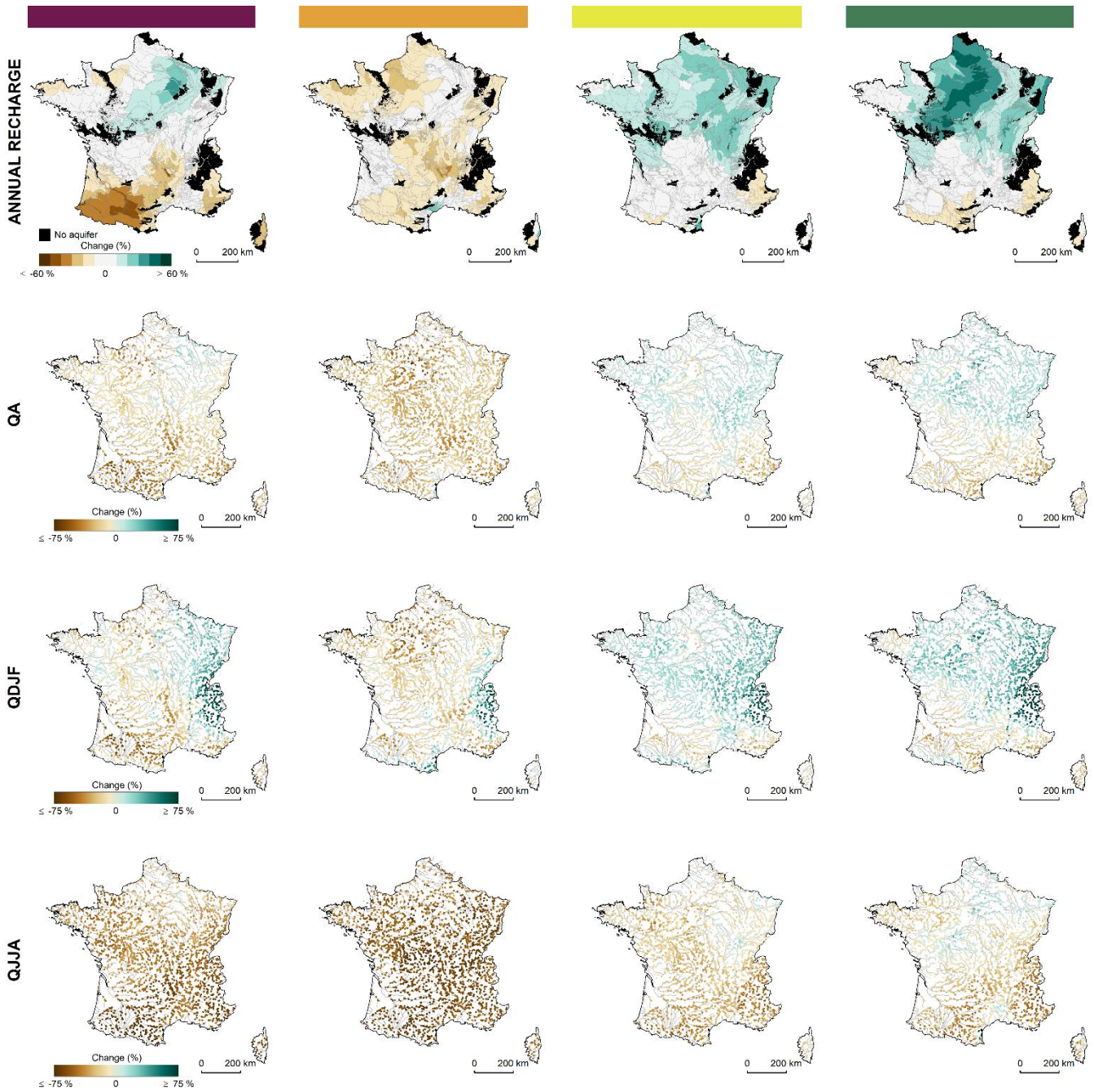
Figure 9: Changes in the annual groundwater recharge and the annual, winter and summer flows between the benchmarkreference period and the end of the century for the four storylines. The areas coloured black on the maps are those where there is no aquifer and where the notion of groundwater recharge is not relevant. Median changes are shown for annual and seasonal flows based on available HMs (please note the different scales in Fig. 7) .
