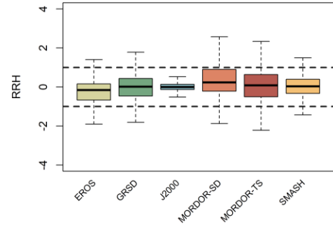
(b) q_{90} CDF-t
