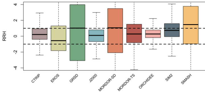
(c) q_a ADAMONT
