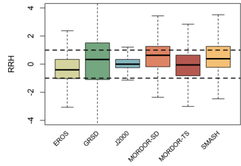
(f) q_{10} CDF-t
