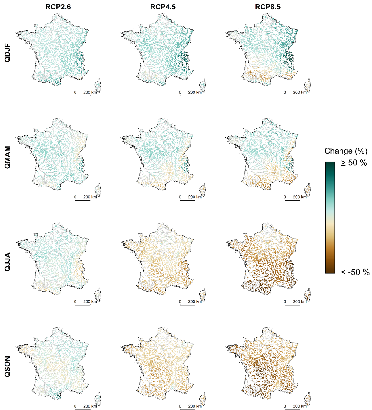
600 Figure 7: Median changes in the seasonal flows QDJF, QMAM, QJJA, and QSON between the benchmark reference period and the end of the century for the three RCPs.
