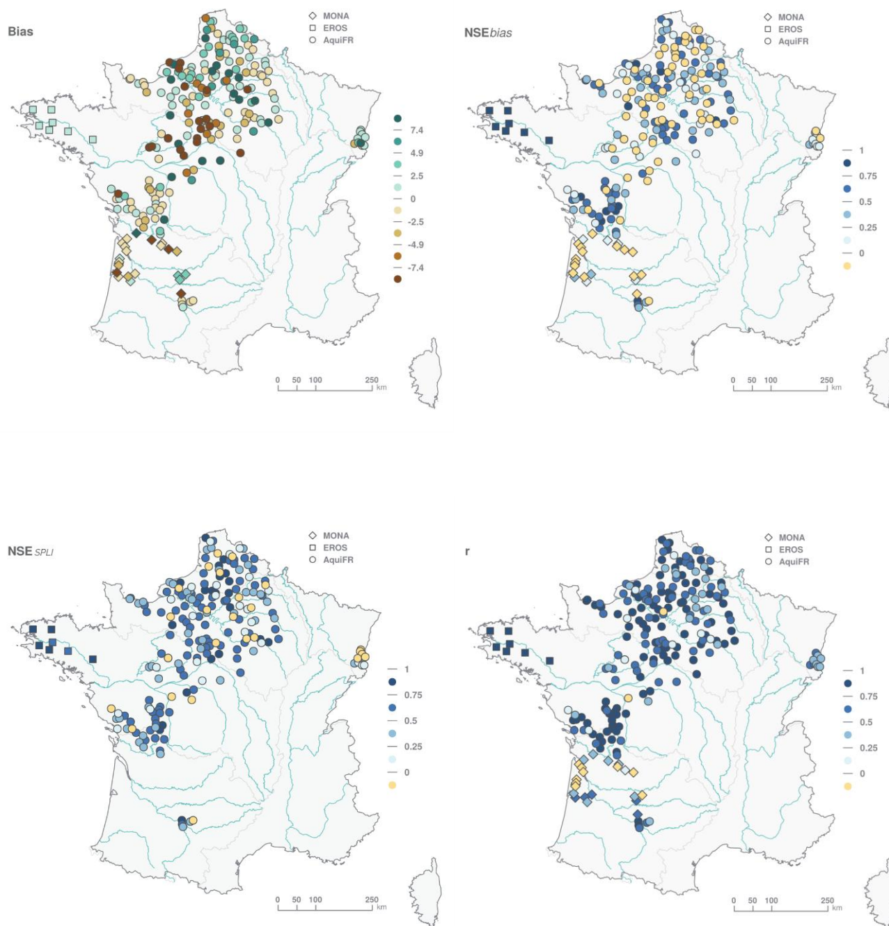
465 Figure 4: Evaluation scores obtained for the three groundwater HMs at the reference piezometers.
