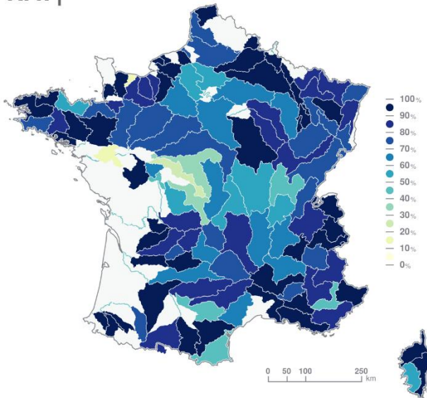
Figure 3: Proportion (%) of simulations with evaluation metrics within the acceptable range. A value of 100 % means that all HMs demonstrate numerical metrics within the acceptable range at all reference gauging stations while a null value means that all HMs demonstrate numerical metrics outside the acceptable range at all reference gauging stations. Statistics of the evaluation metrics have been computed on a division of France into 187 sub-basins ( https://www.sandre.eaufrance.fr ) to identify contrasts in HM performance over the 611 reference gauging stations.
