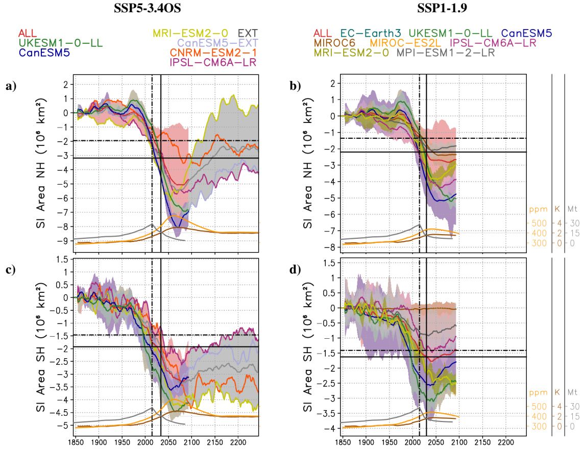
Figure 6. (a,b) Anomaly of Sea Ice (SI) area in the NH with respect to 1861-1880 obtained from the CMIP6 simulations of experiments (a) SSP5-3.4OS and (b) SSP1-1.9, including the ALL and EXT ensembles, the ensemble average for each individual model and the individual extended simulations. Envelopes show the min-max values within each ensemble. Yellow, gray and brown curves in the lower part of each panel respectively show the CO 2 concentration from Meinshausen et al. (2020), the anthropogenic aerosol emissions from Feng et al. (2020), and the global surface air temperature obtained with the SSP1-1.9 ALL ensemble and the SSP5-3.4OS EXT ensemble. The vertical lines show the year before the overshoot with the same CO 2 concentration (dashed line) and global surface air temperature (solid line) as at the end of the run (2100 for the SSP1-1.9 ALL ensemble and 2300 for the SSP5-3.4OS EXT ensemble), while the horizontal lines represent the value of SI area in the NH in the SSP1-1.9 ALL ensemble and in the SSP5-3.4OS EXT ensemble for those years. (c,d) Same as Fig. 6a,b, but for the SI area in the SH.
