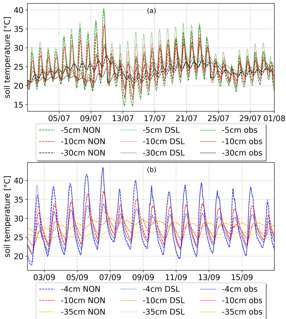
Figure 11. Soil temperature at La Cendrosa site (a) and Els Plans (b). Levels comprise at 4, 5, 10, 30 and 35 cm depending on the availability for the site. Observed temperature is shown in solid lines, the NON simulation in dashed lines and the DSL simulation in dotted lines.
