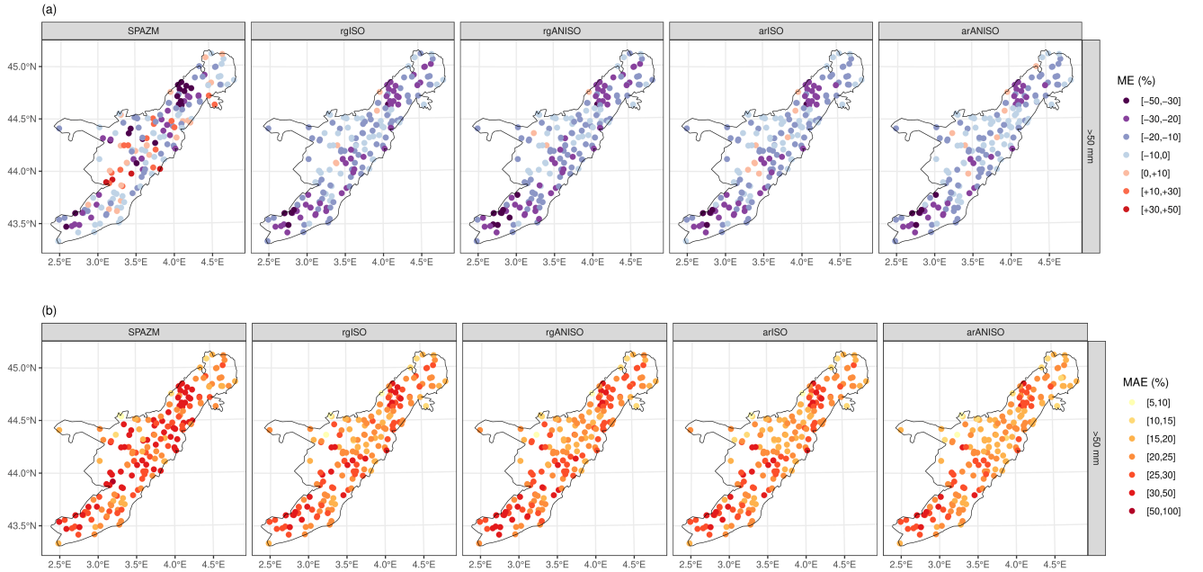
Figure 2. Cross-validation mean error (ME, (a)) and mean absolute error (MAE, (b)) for rain gauge stations in the Cévennes region, considering days with more than 50 mm. Results are shown for deterministic models (SPAZM) and stochastic models (rgISO, rgANISO, arISO, arANISO). For stochastic models, the cross-validation is conducted on the mean of 100 ensemble members from conditional simulations. Black contours indicate the Cévennes region.
